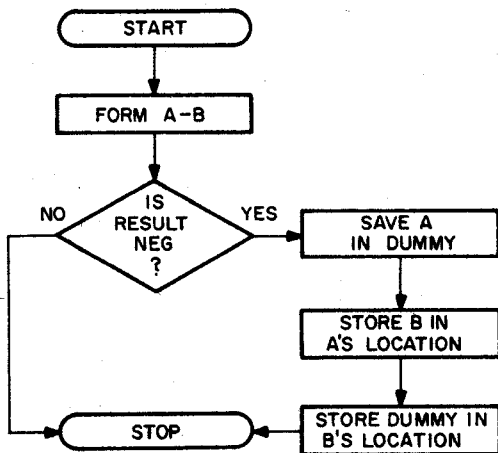
Figure 4-9 Conditional Skip
