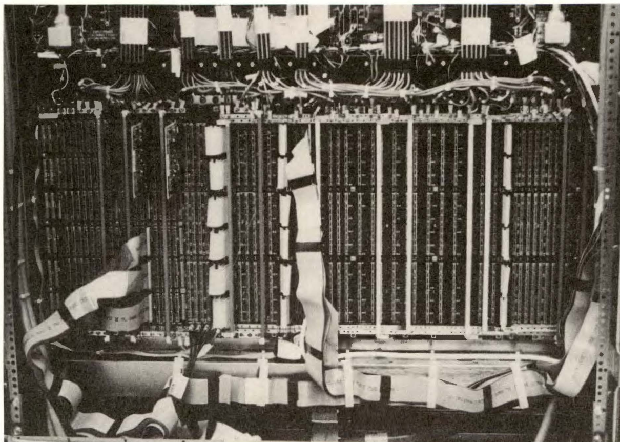
Figure 6 Backplane Assembly
