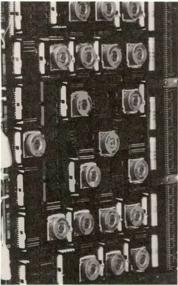
Figure 5 LSI Module
