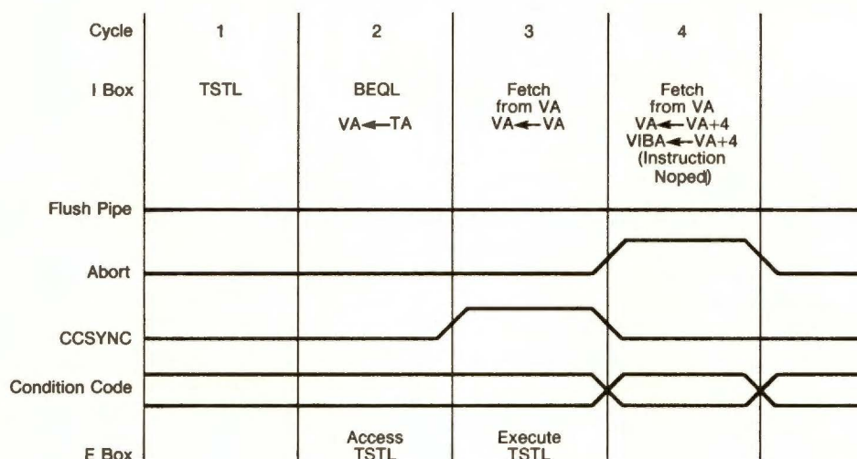
Figure 6b Branch Not Taken Sequence
