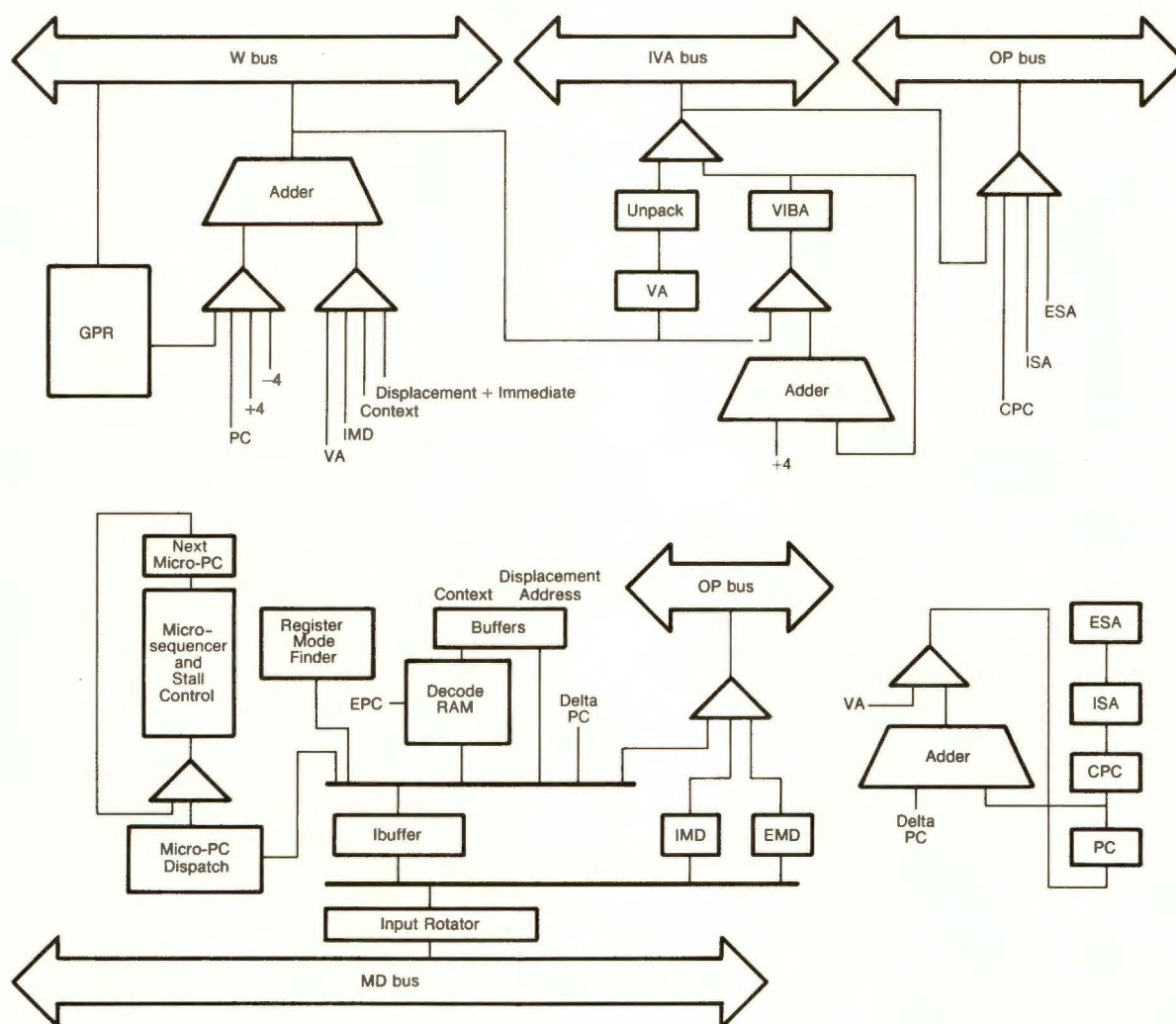
Figure 5 VAX 8600 I Box Datapath
