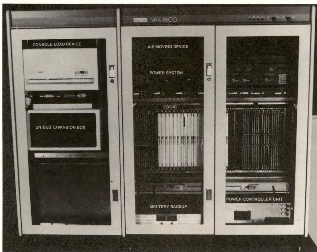
Figure 1 Card Cage
