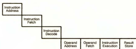
Figure 3b The VAX-11/780 Instruction Pipeline
