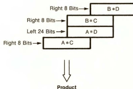
Figure 7 Wallace Tree
