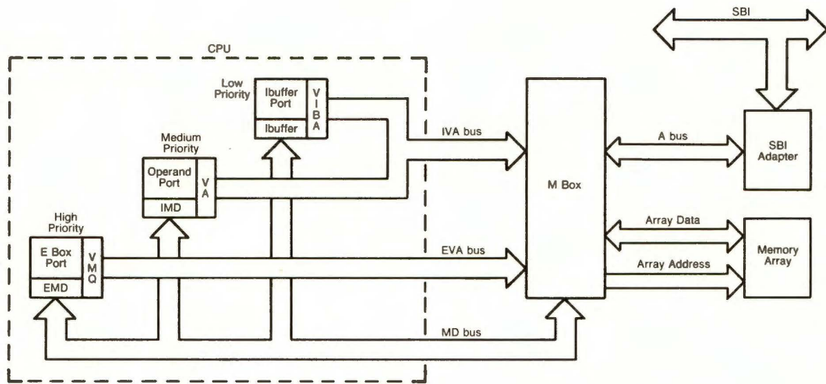
Figure 2 Port Organization
