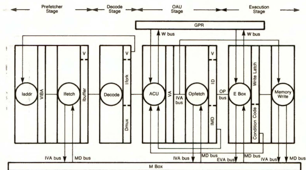
Figure 4c Simplified VAX 8600 Pipeline Model
