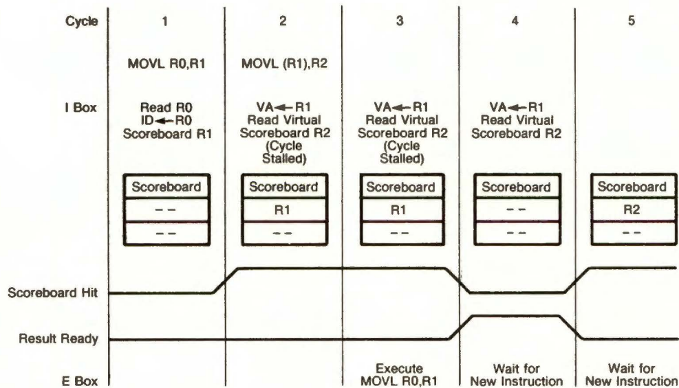
Figure 7 Scoreboard Example
