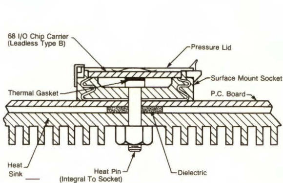
Figure 1 Heat Pin Detail
