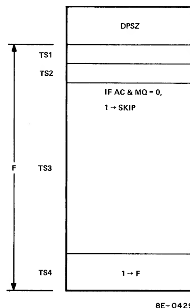
Figure 1-7 DPSZ Instruction, Flow Diagram
