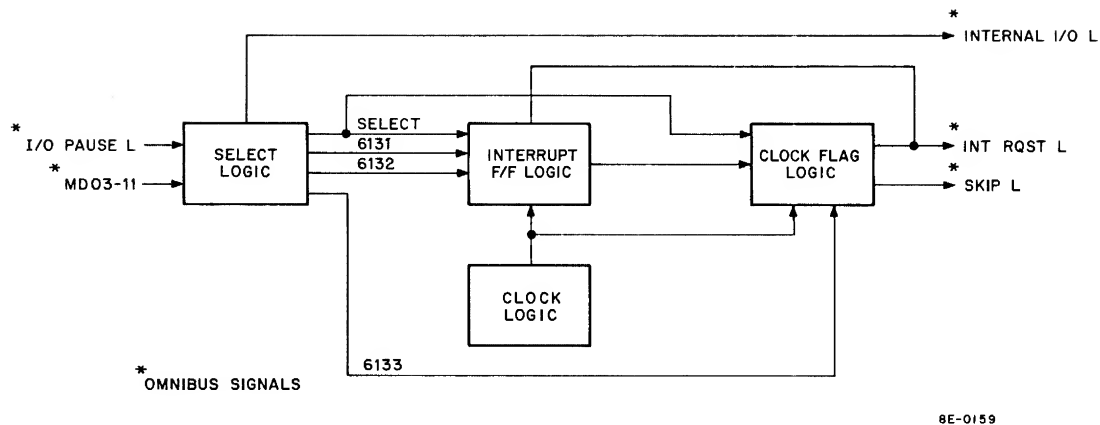
Figure 6-1 Real-Time Clock (DK8-EA, DK8-EC), Block Diagram
