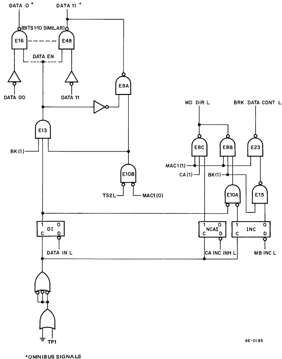
Figure 10-7 Data Transfer Logic
