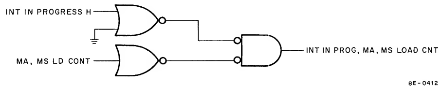
Figure 2-16 Interrupt Break Detect Logic
