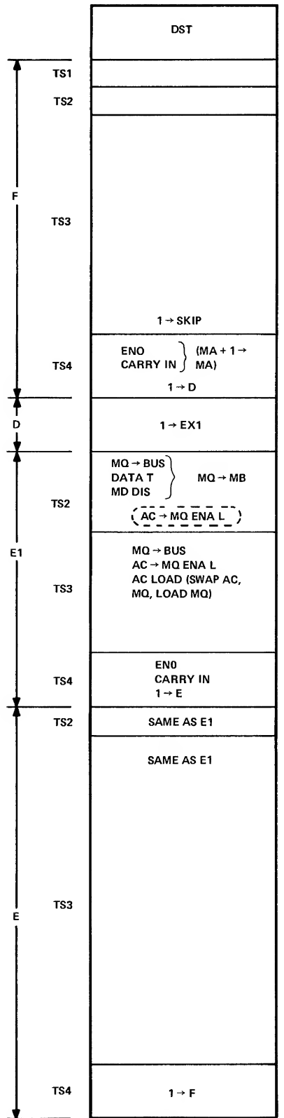
Figure 1-10 DST Instruction, Flow Diagram
