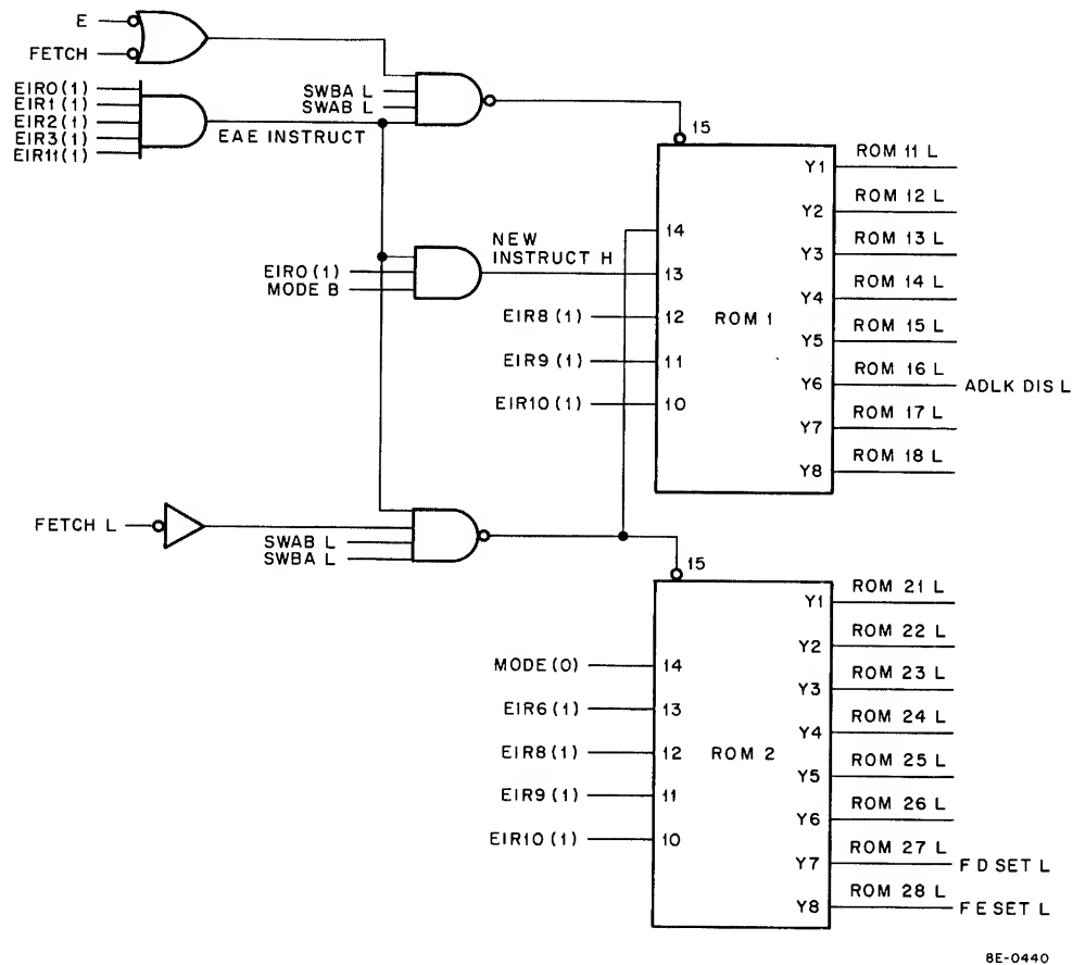
Figure 1-20 ROM Logic
