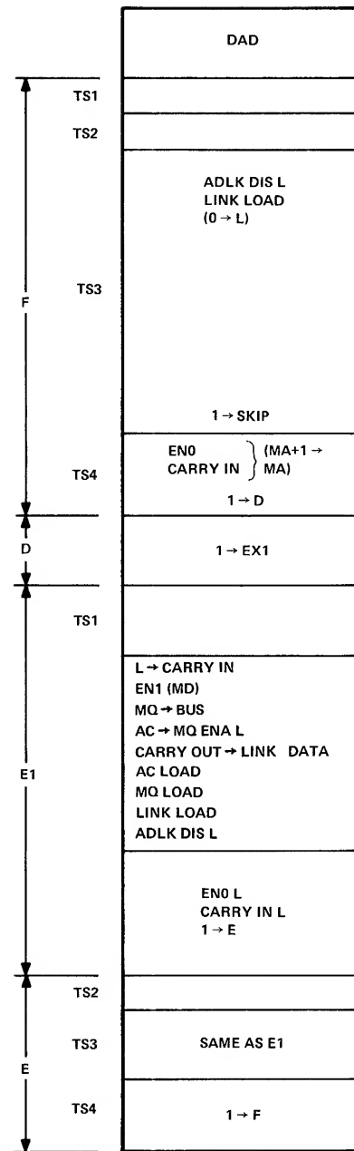
Figure 1-11 DAD Instruction, Flow Diagram
