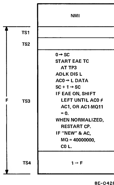
Figure 1-6 NORMALIZE Operation, Flow Diagram
