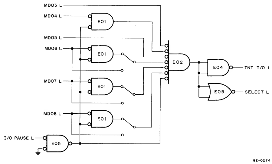
Figure 8-2 Device Select Logic
