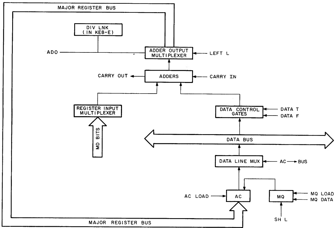
Figure 1-16 Major Registers
