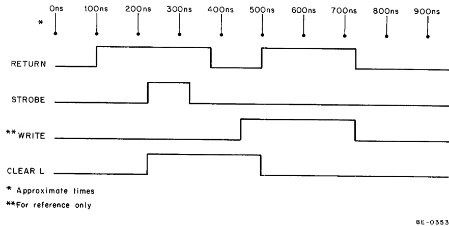
Figure 3-9 Read Timing Diagram
