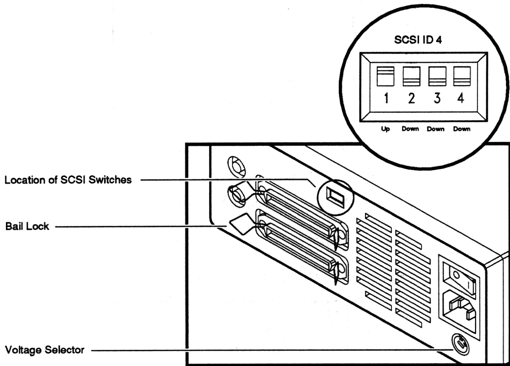
Figure 4-12 Compact Disc Voltage Selector and Factory SCSI ID Switch Positions
