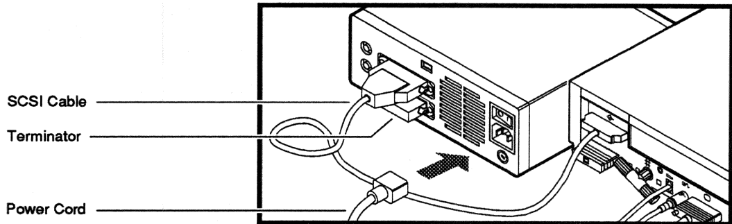
Figure 4-9 Connecting One Compact Disc Expansion Box
