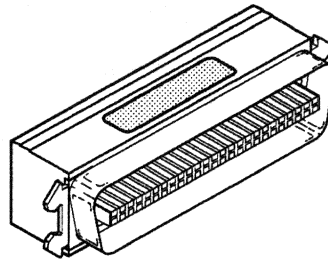
Figure 4-10 SCSI 50-Pin Terminator
