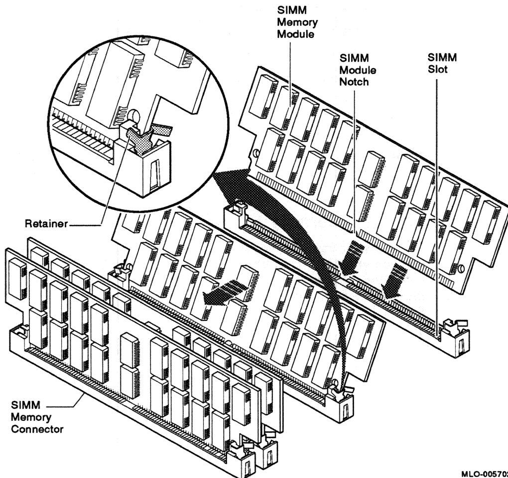
Figure 9–8 Adding Two SIMMs
