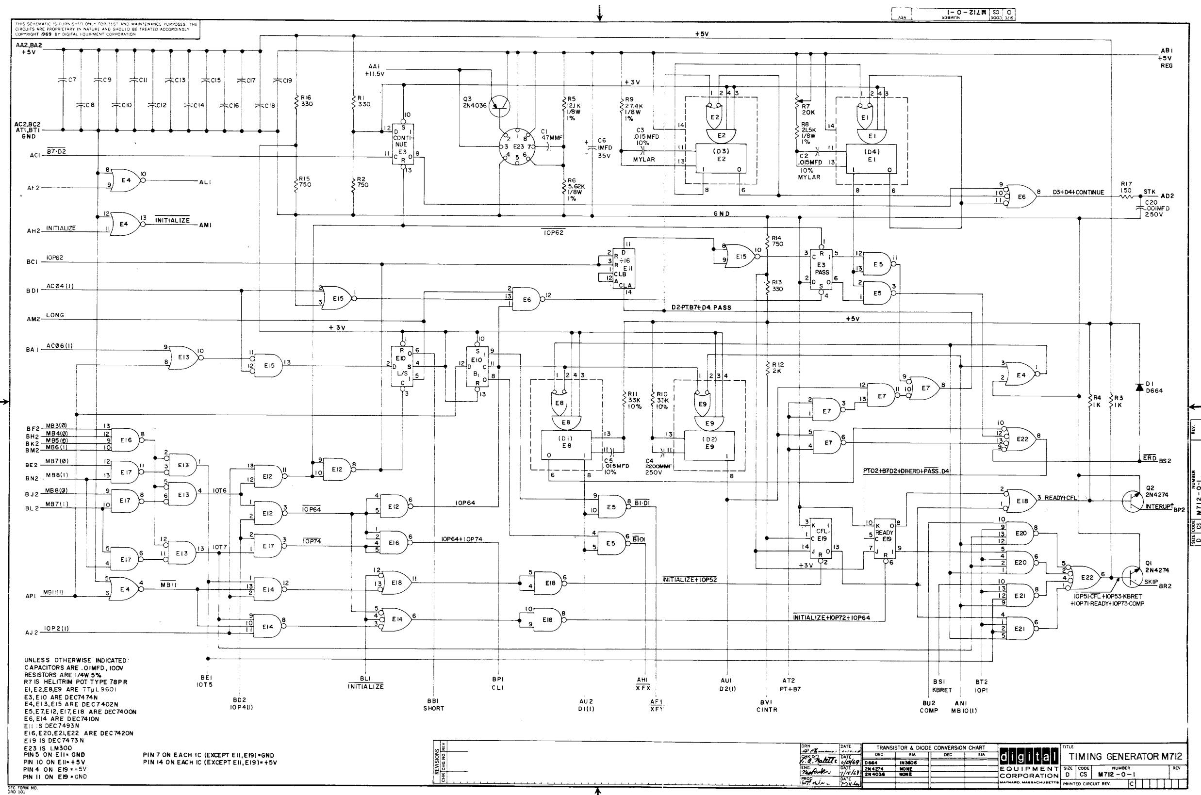
Figure 7-1. Timing Generator Module M712, Schematic Diagram, M712-0-1
