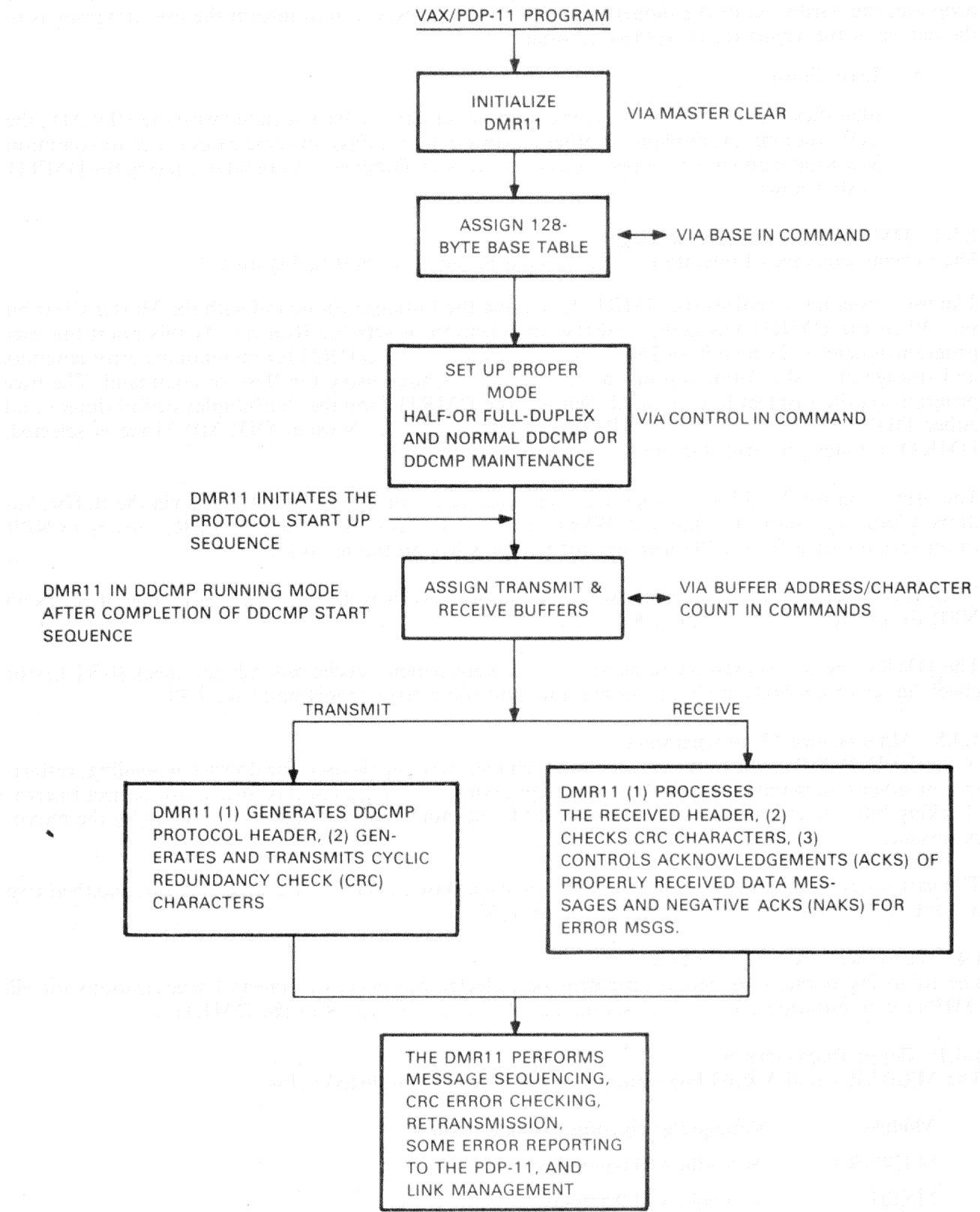
Figure 1-3 DMR11 Operation Sequencing
