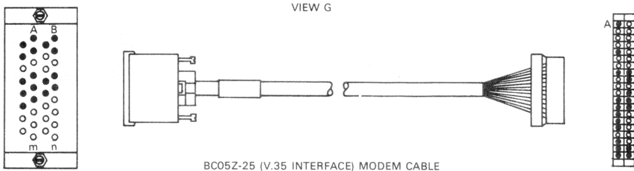
Figure 2-4 DMR11 Cable Drawings (Sheet 4 of 4)
