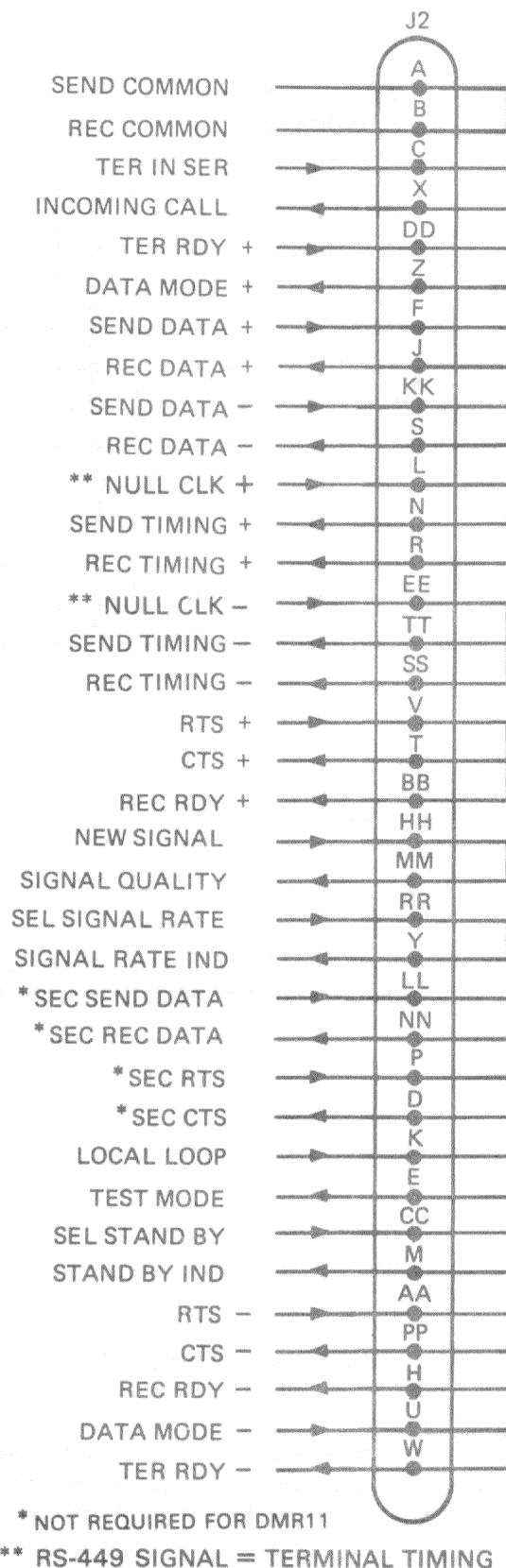
Figure 2-5 DMR11 Turnaround Test Connectors (Sheet 3 of 5)
