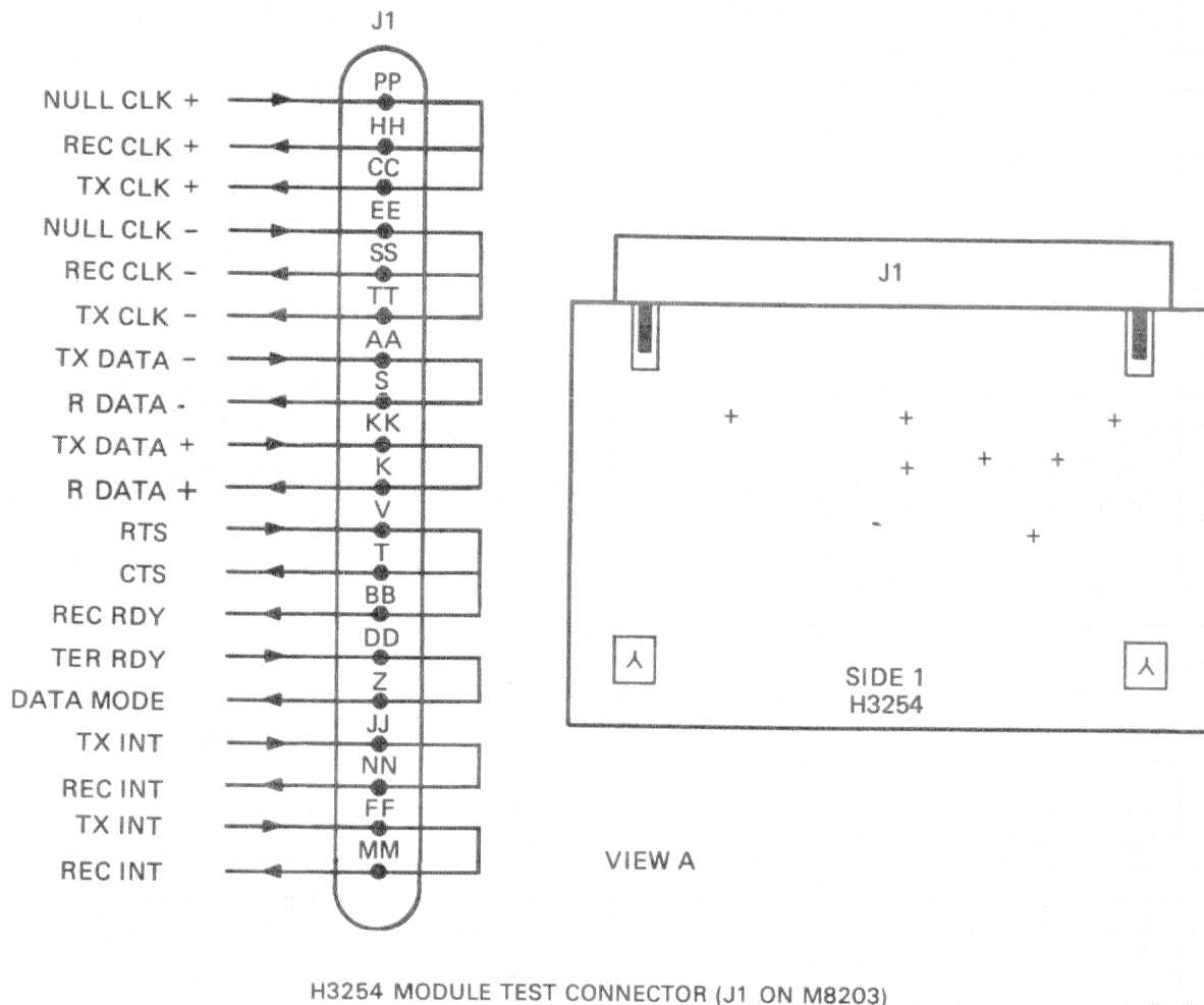
Figure 2-5 DMR11 Turnaround Test Connectors (Sheet 1 of 5)
