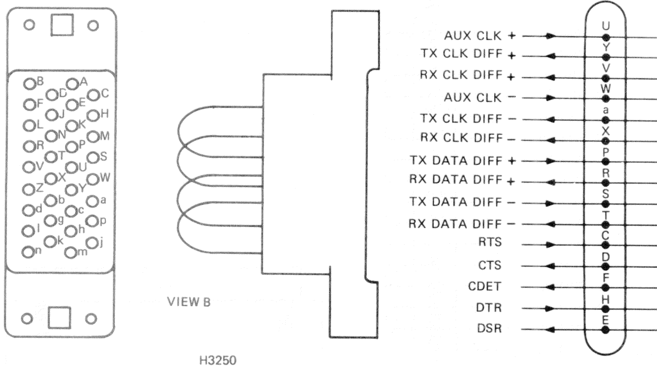
Figure 2-5 DMR11 Turnaround Test Connectors (Sheet 2 of 5)
