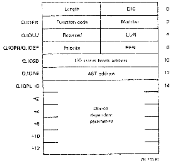
Figure 4-2: QIO Directive Parameter Block (DPB)
