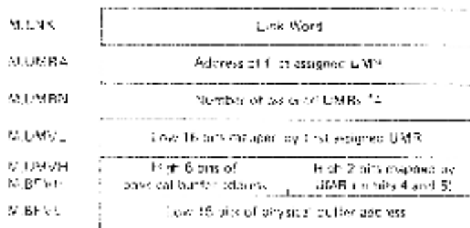
Figure 7-1: Mapping Register Assignment Block
