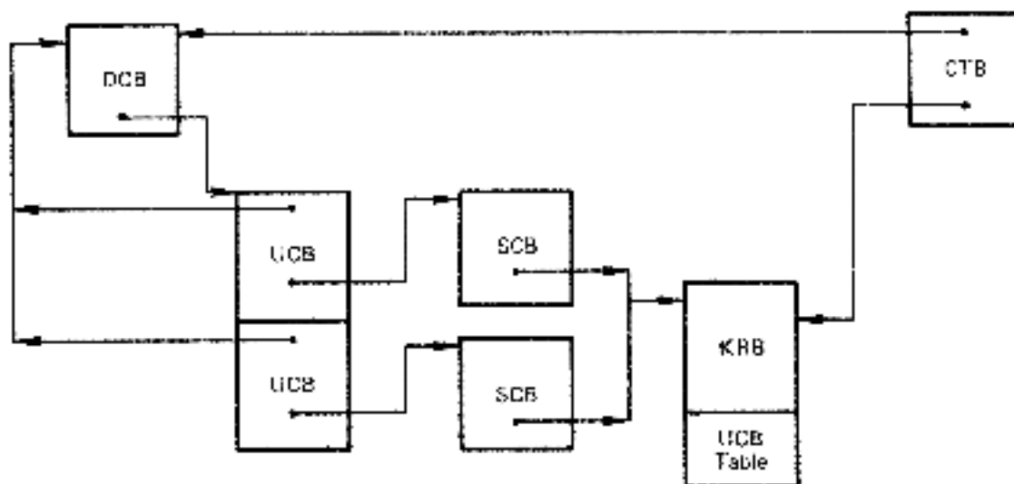
Figure 2-3 Parallel Unit Operation (Overlapped Seek)
