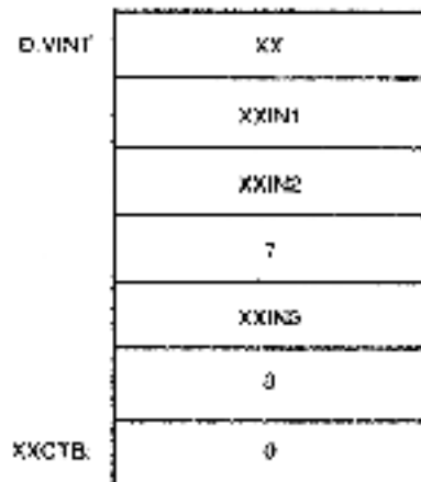
Figure 4-19: Sample Interrupt Address Block in the DDT
