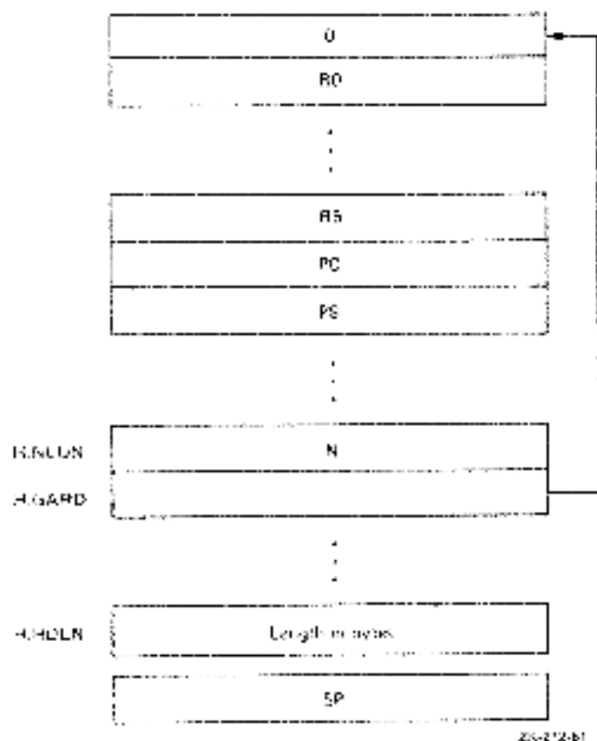
Figure 6-2: Task Header
