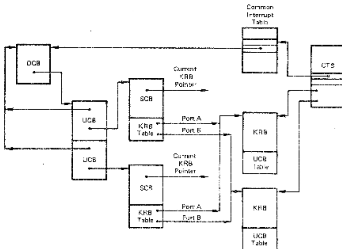
Figure 2-4 Dual-Access Operation
