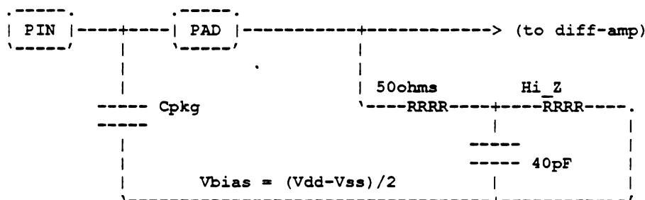
Figure 6–1: Clock Termination
