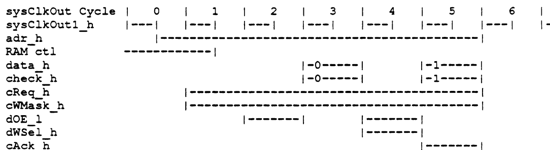
Figure 4-8: WRITE_BLOCK Sequence
