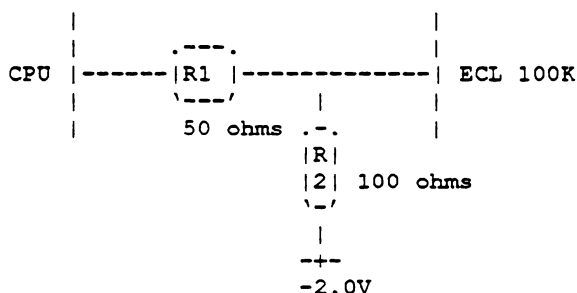
Figure 5-1: ECL Termination
