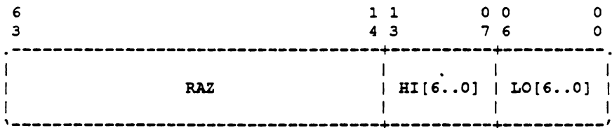
Figure 3–30: FILL_SYNDROME Register
