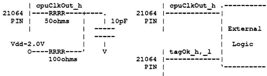
Figure 6-4: Flow-Through Delay
