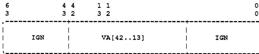
Figure 3—4: Translation Buffer Tag (TB_TAG) Register
