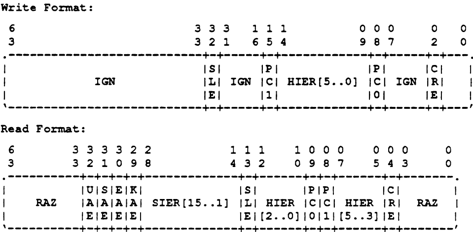
Figure 3–17: Hardware Interrupt Enable Register (HIER)
