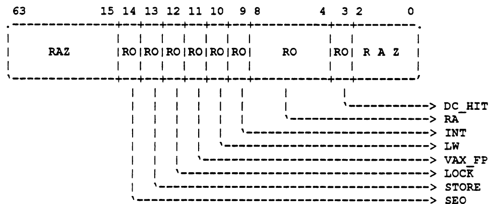
Figure 3–28: Data Cache Status Register (DC_STAT)
