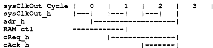
Figure 4–10: FETCH Sequence
