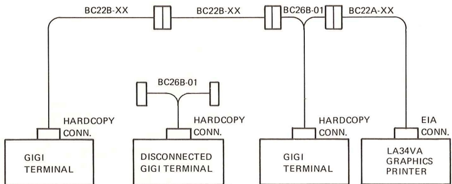
FIGURE 2-12 Removing a Terminal from a Multiterminal String
