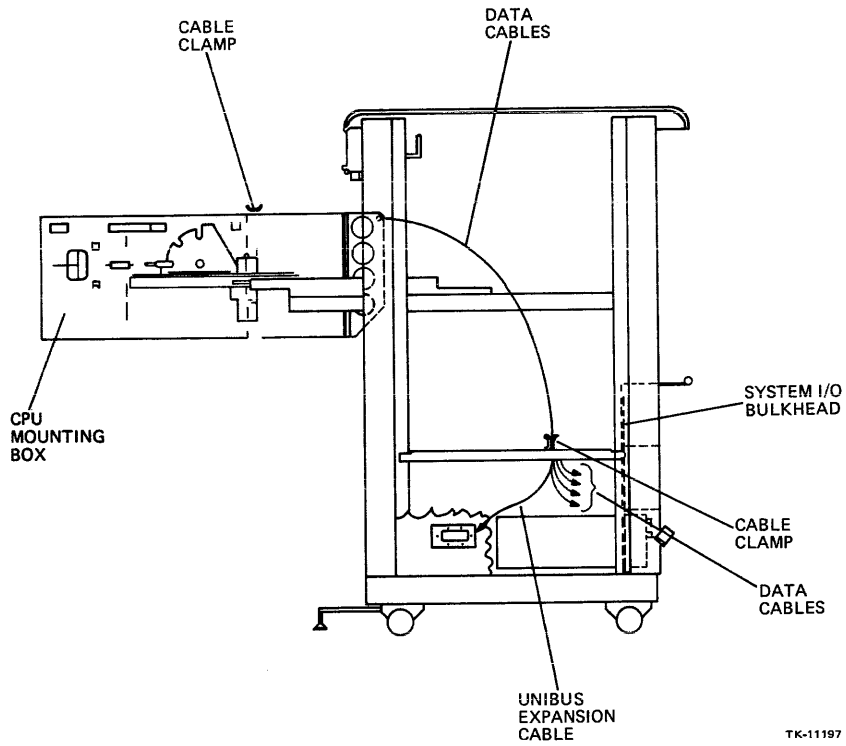
Figure 7-3 Cable Routing Through the System Cabinet with the CPU Mounting Box Extended
