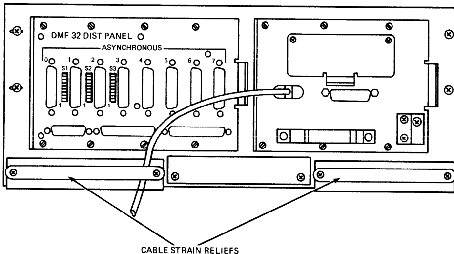
Figure 6-17 Cable Strain Reliefs for Exterior Cabling
