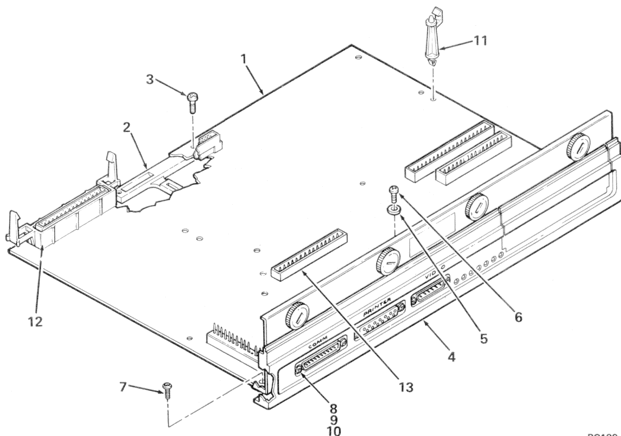
Figure 3A PC100-B CPU Assembly
