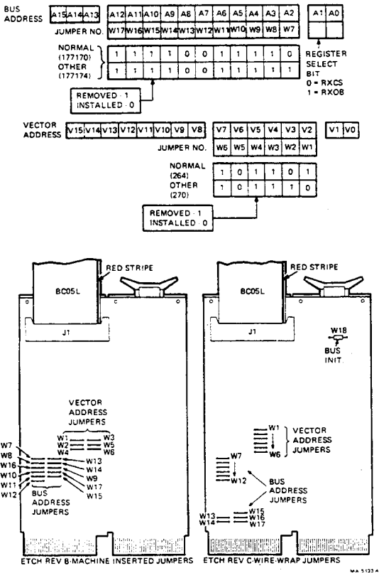
Figure 1-9 M7946 Interface (RXV11)
