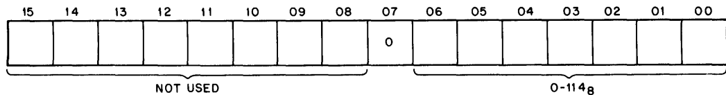
Figure 3-2 RXTA Format (RX11)
