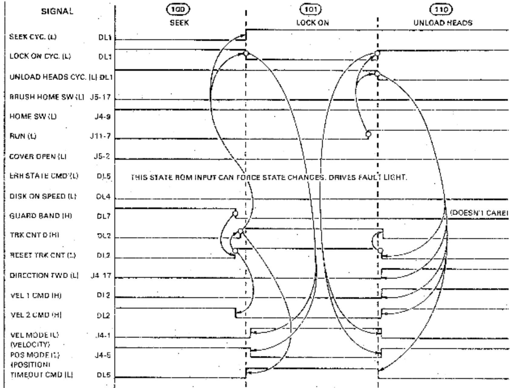
Figure 4-13 Device Startup - Lock on Track 0 Timing
