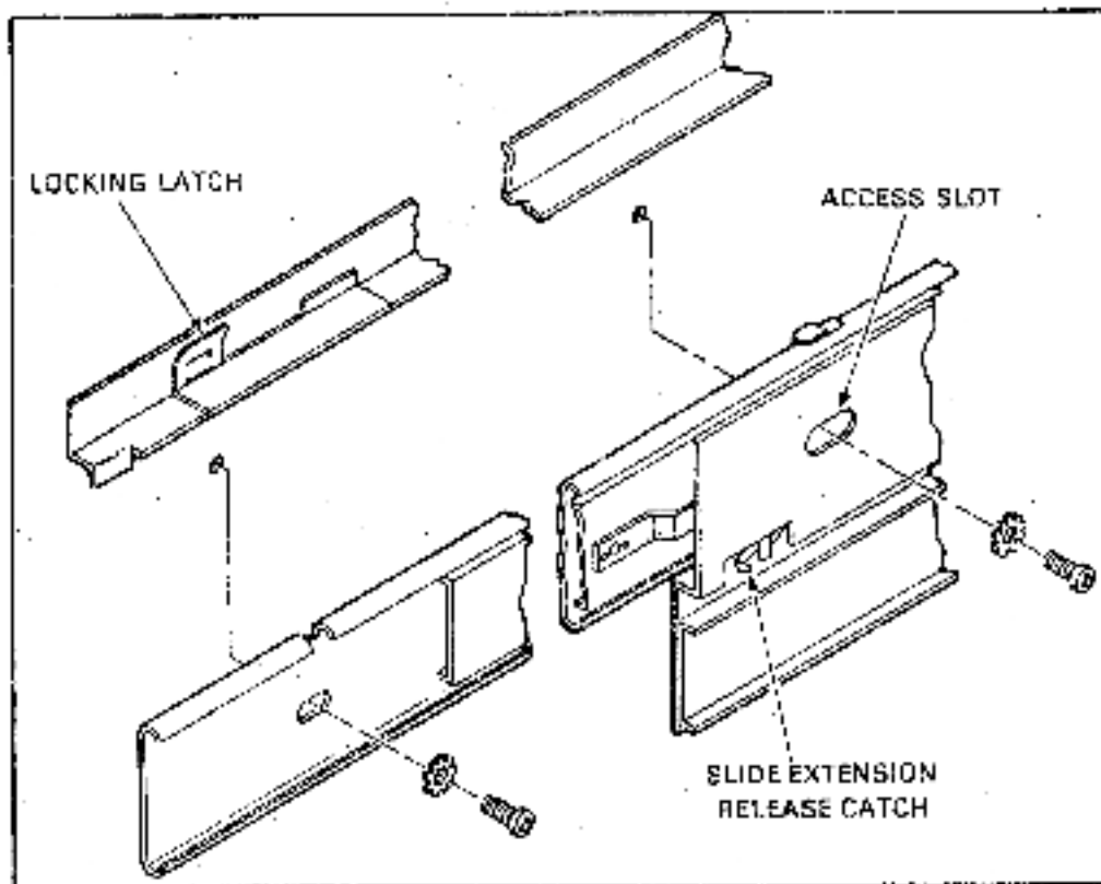
Figure B-28 RL01/RL02 Cabinet Installation
