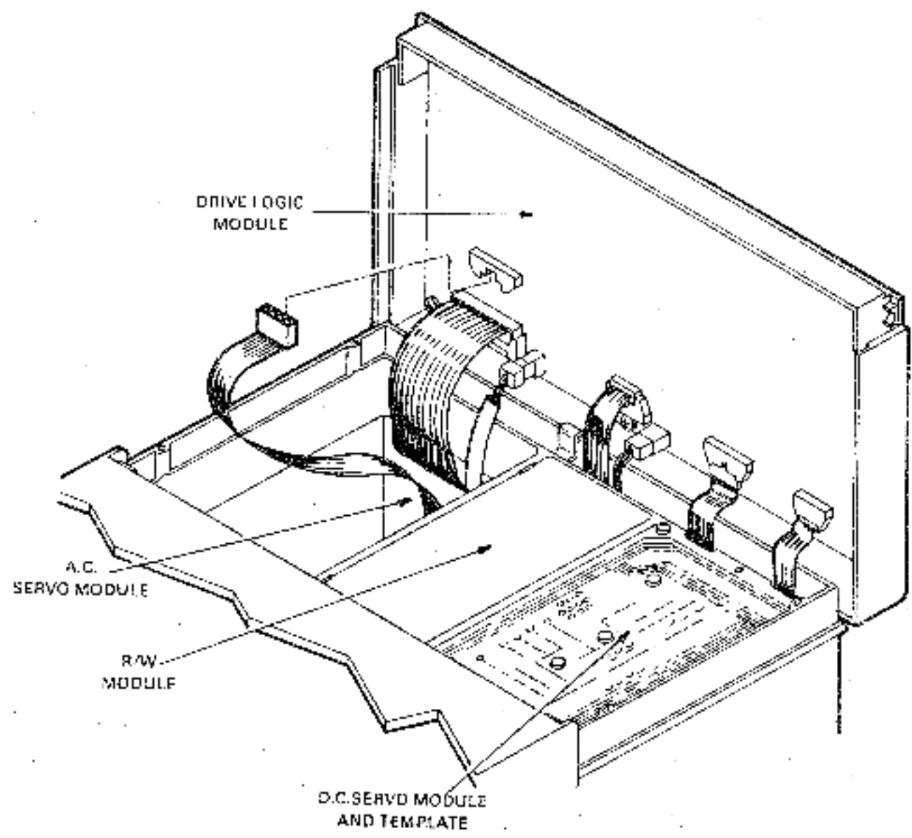
Figure 1-9 Logic Modules
