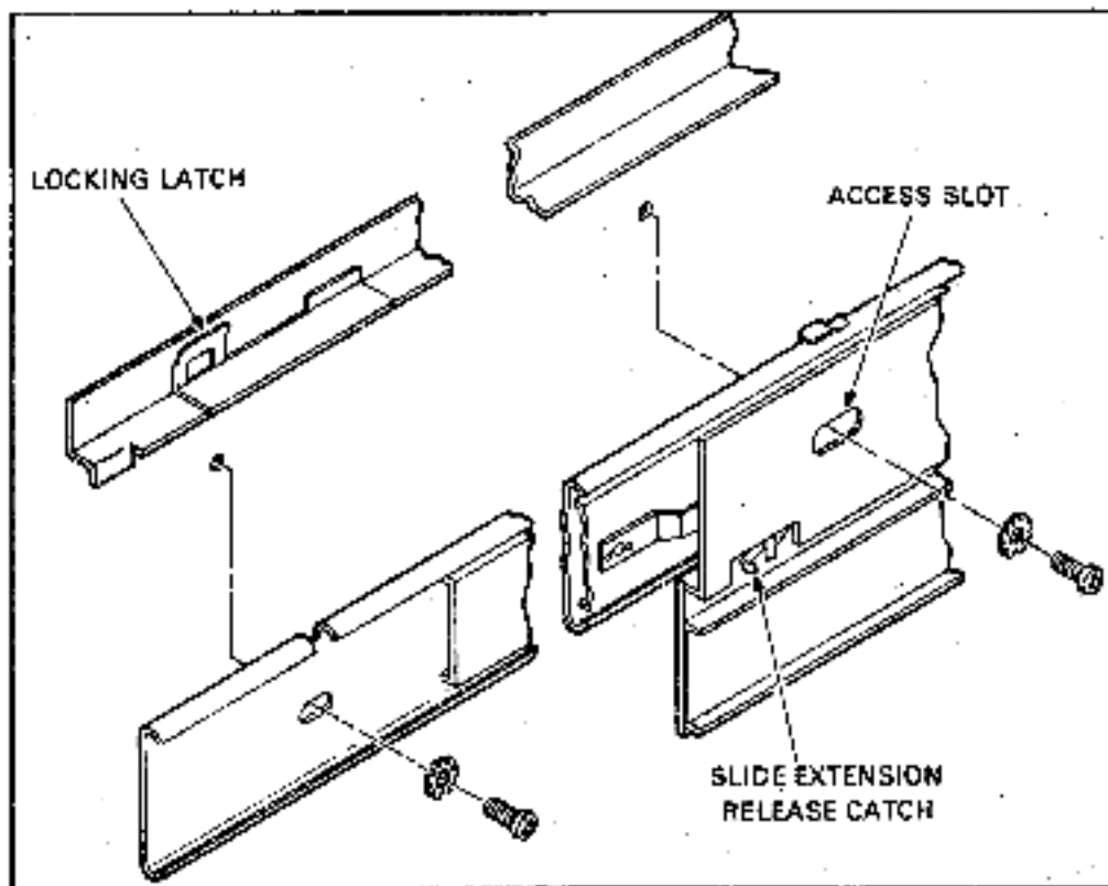
Figure 2-6 Slide Rails
