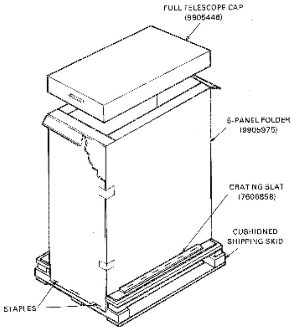
Figure 2-14 11950 Shipping Package
