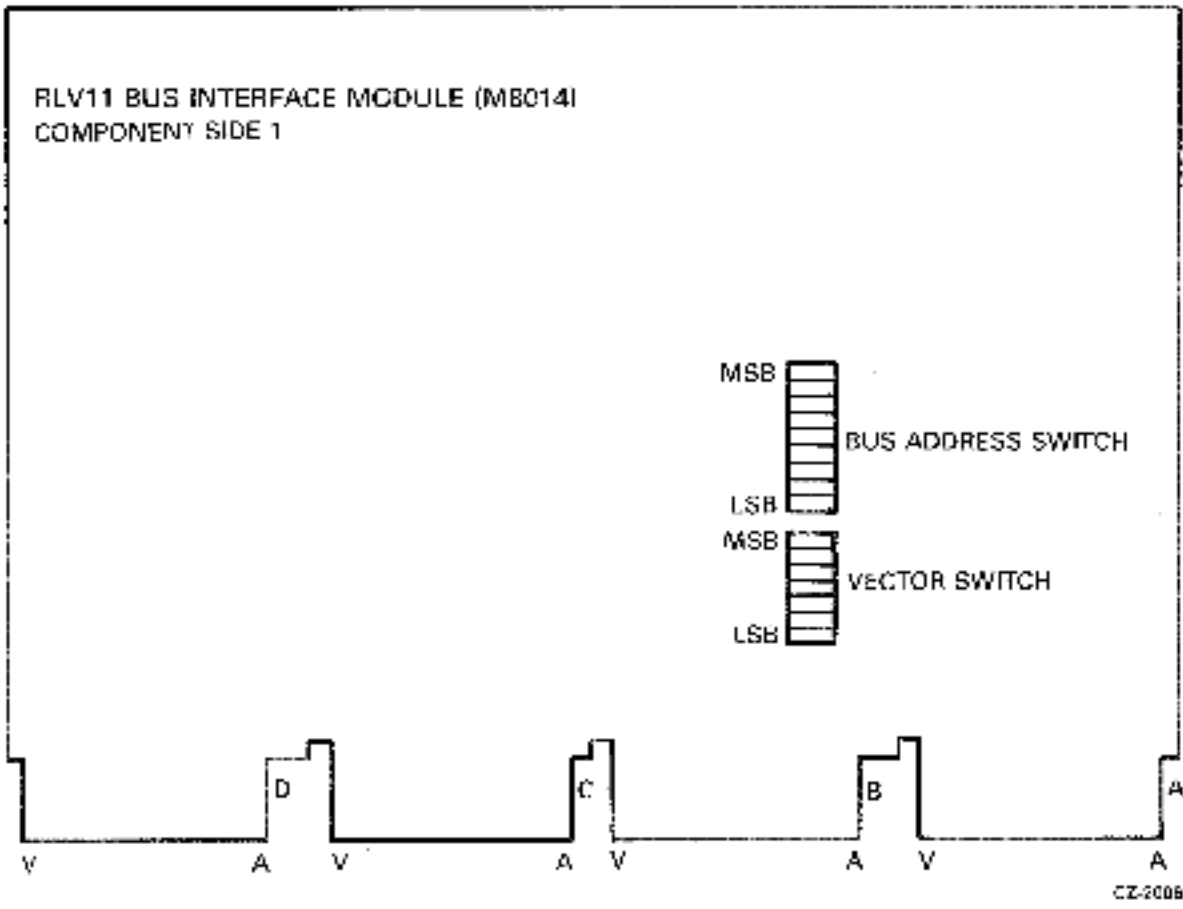
Figure 2-13 RLV11 Bus Interface Module (MB014) (Component Side)
