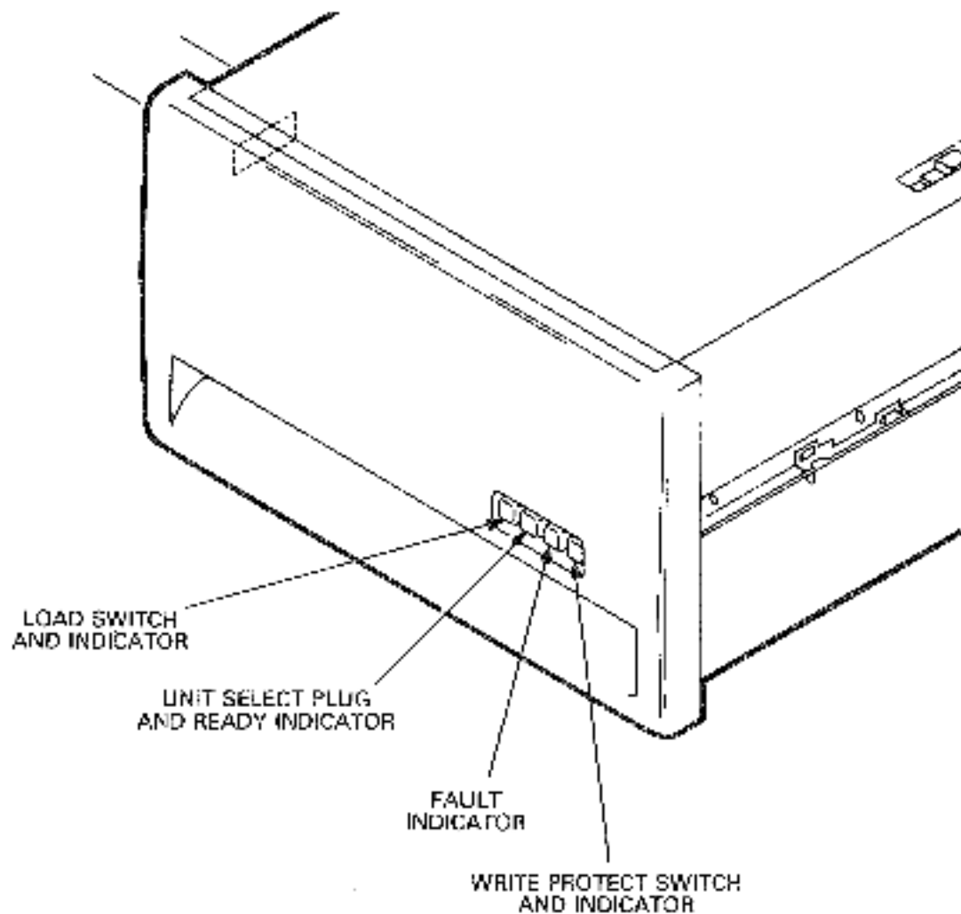
Figure 2-29 RL01/RL02 Disk Drive: front View
