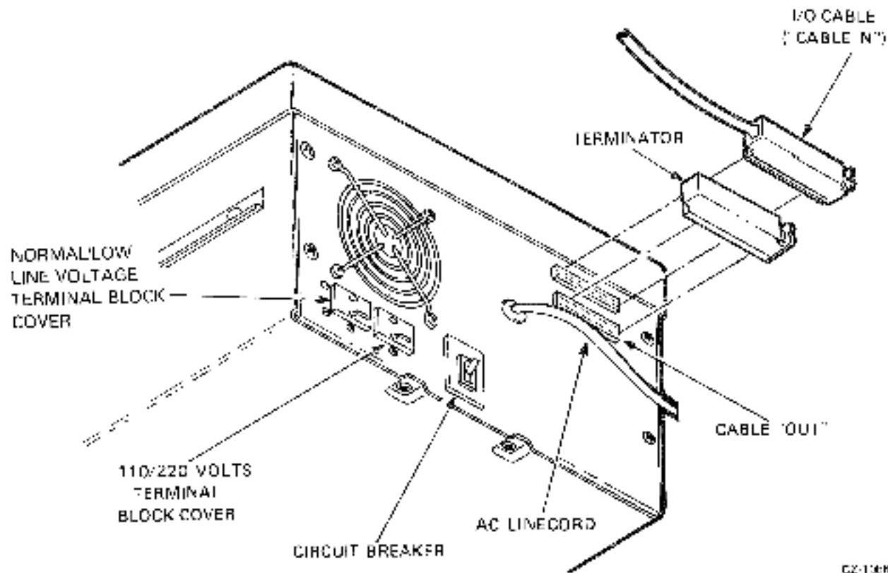
Figure 2-23. RL01/RL02 Disk Drive Rear View
