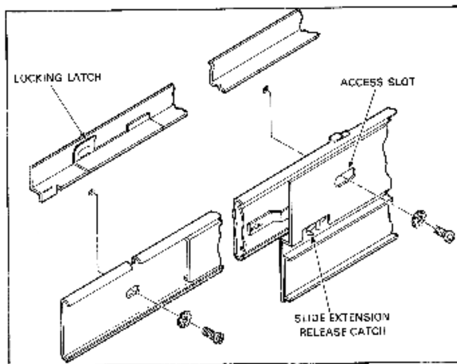
Figure 2-20 RL018102 Cabinet Installation
