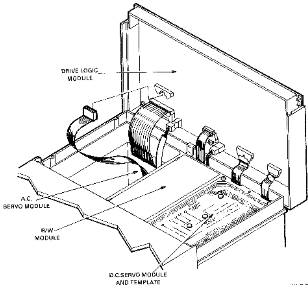
Figure 2-24 R101/R102 Disk Drive-Exposed Drive Logic Module
