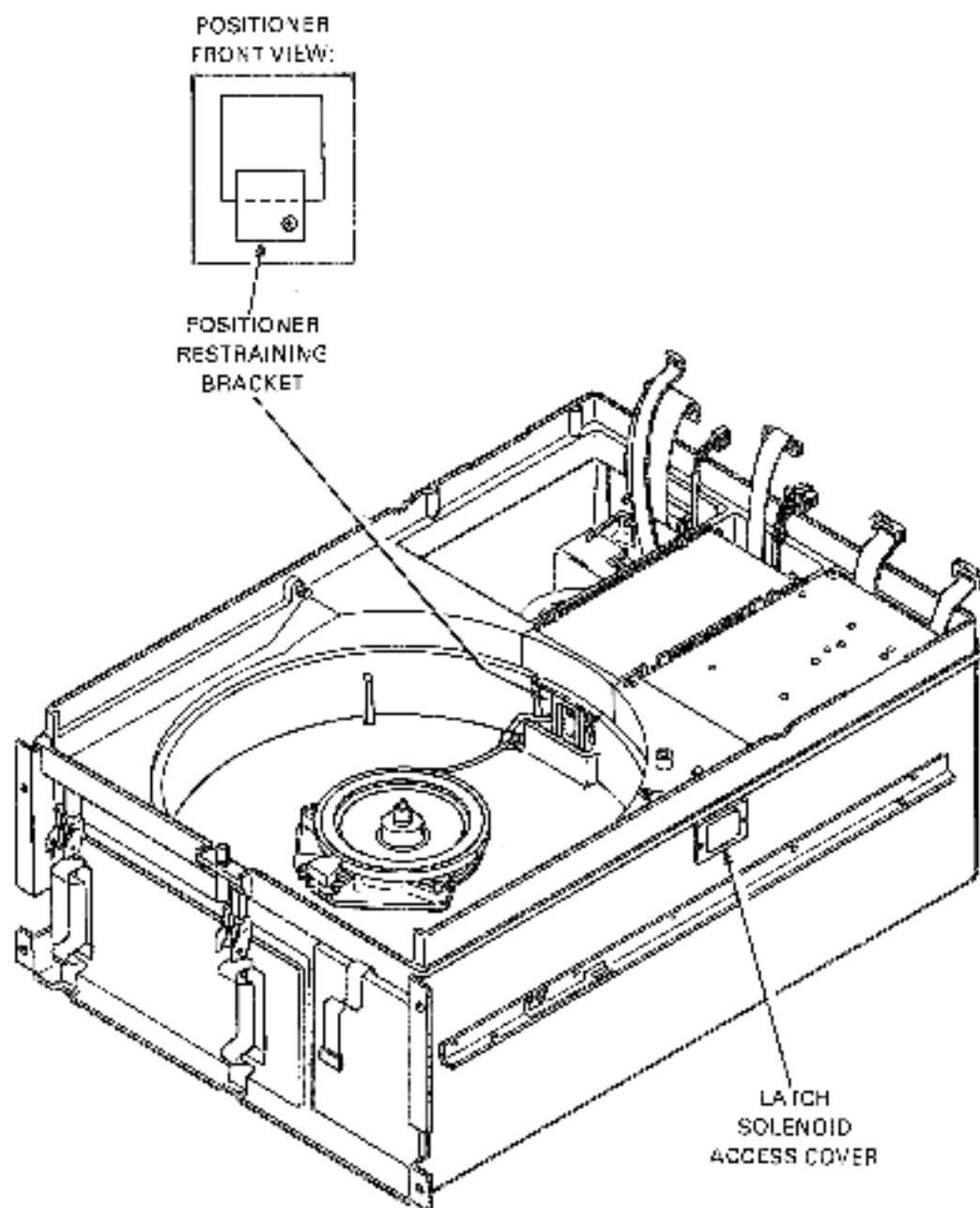
Figure 2-21 RL01/RL02 Covers Removal
