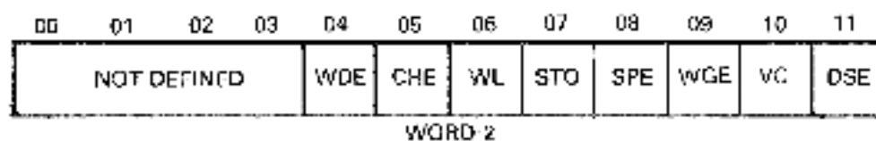
Figure 5.9. Bit Buffer for Status Word 2
