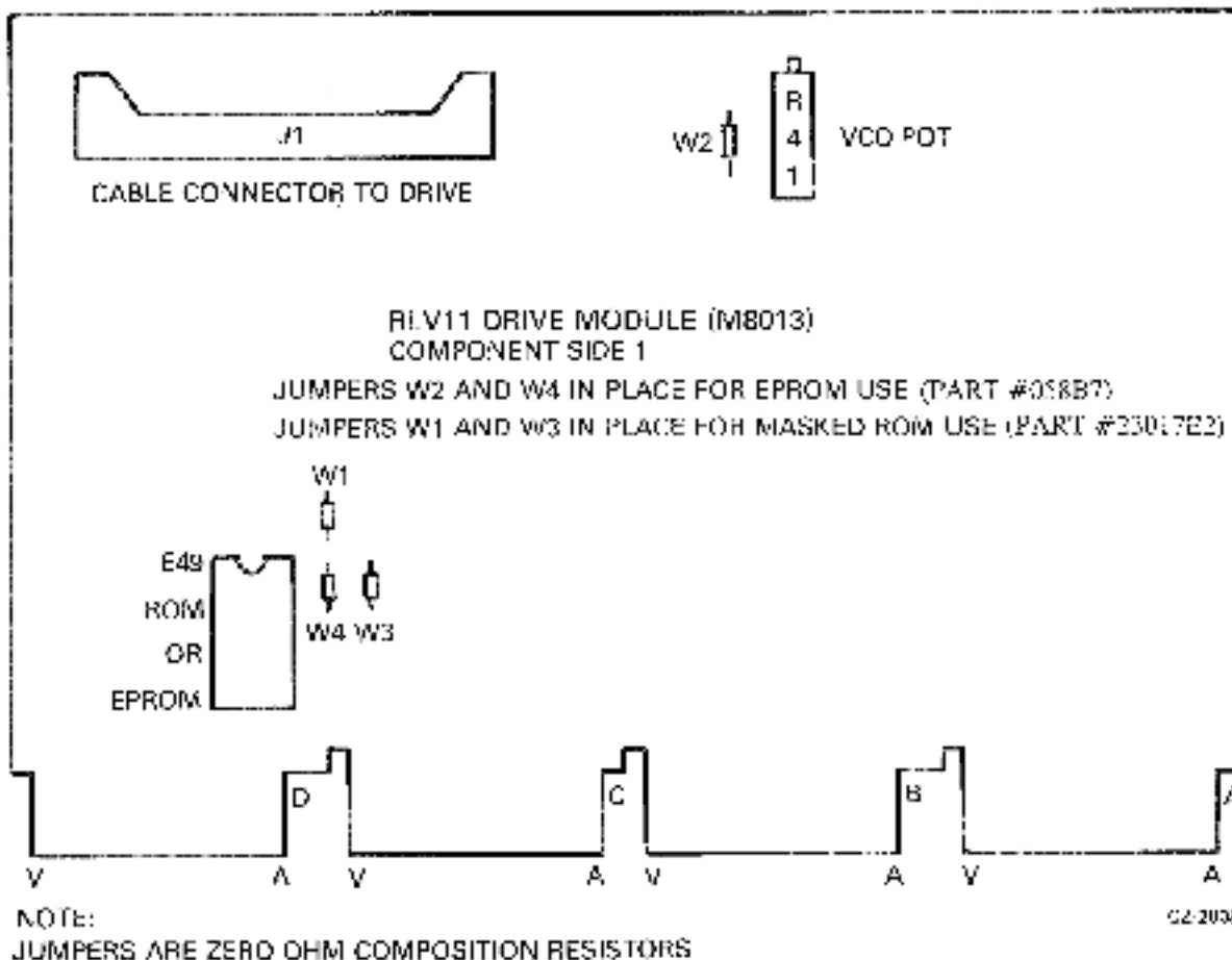
Figure 2-16 RL V11 Drive Module (M8013)
