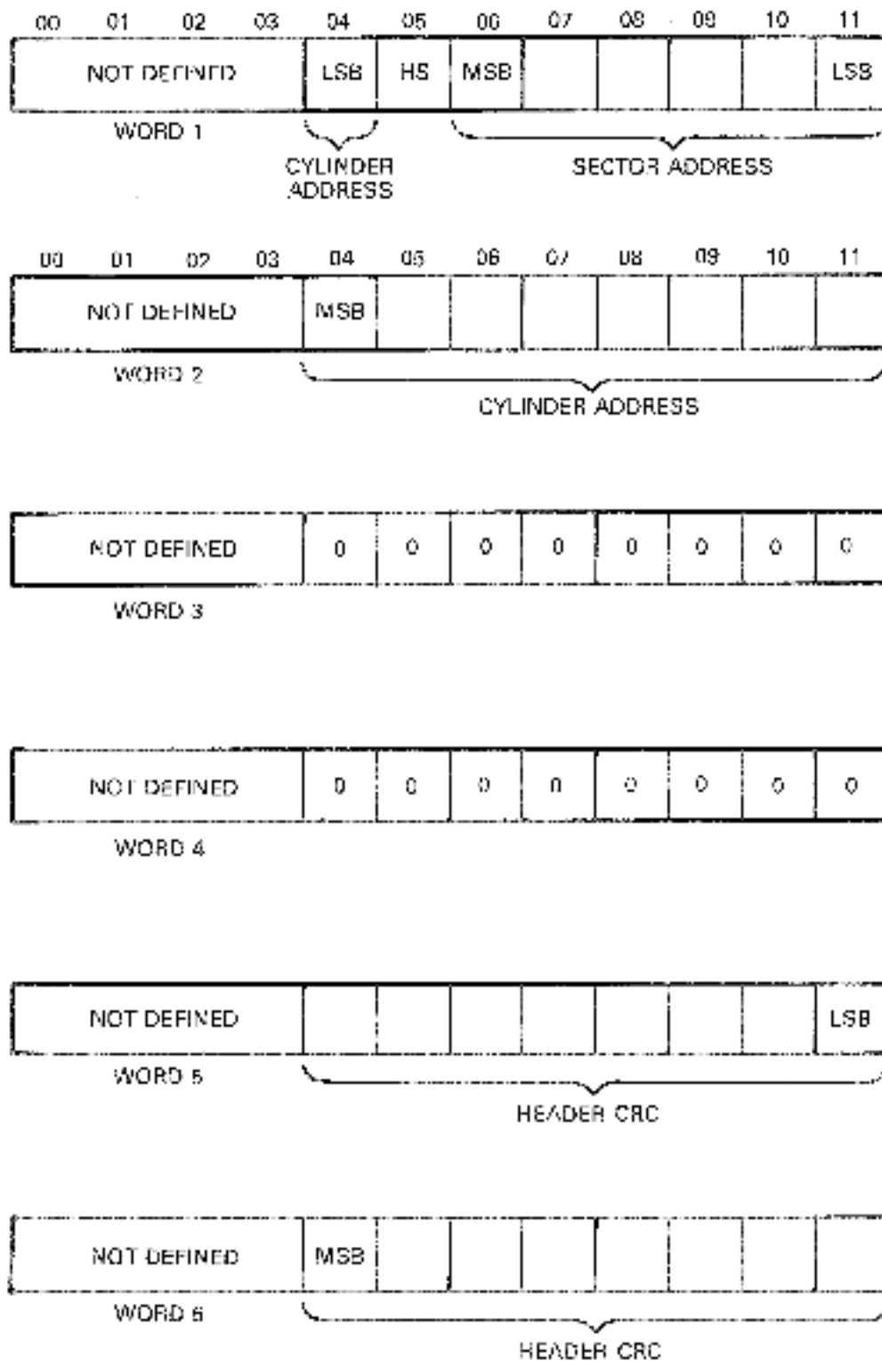
Figure 3-10 Side Buffer for Header Words
