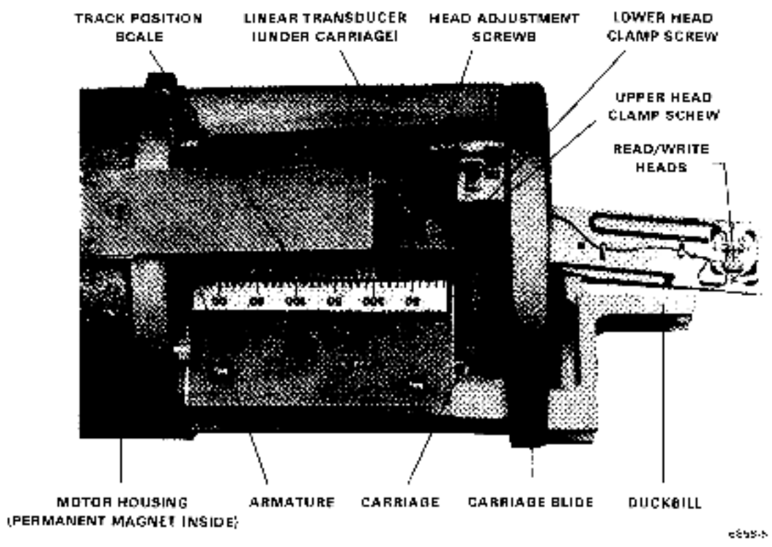
Figure 1-4 Linear Positioner
