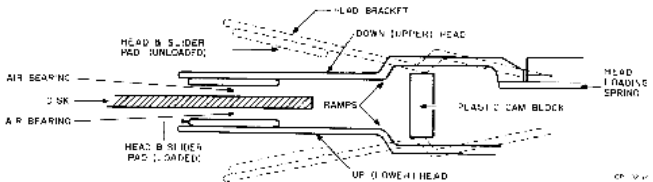
Figure 1-7 Head Landing
