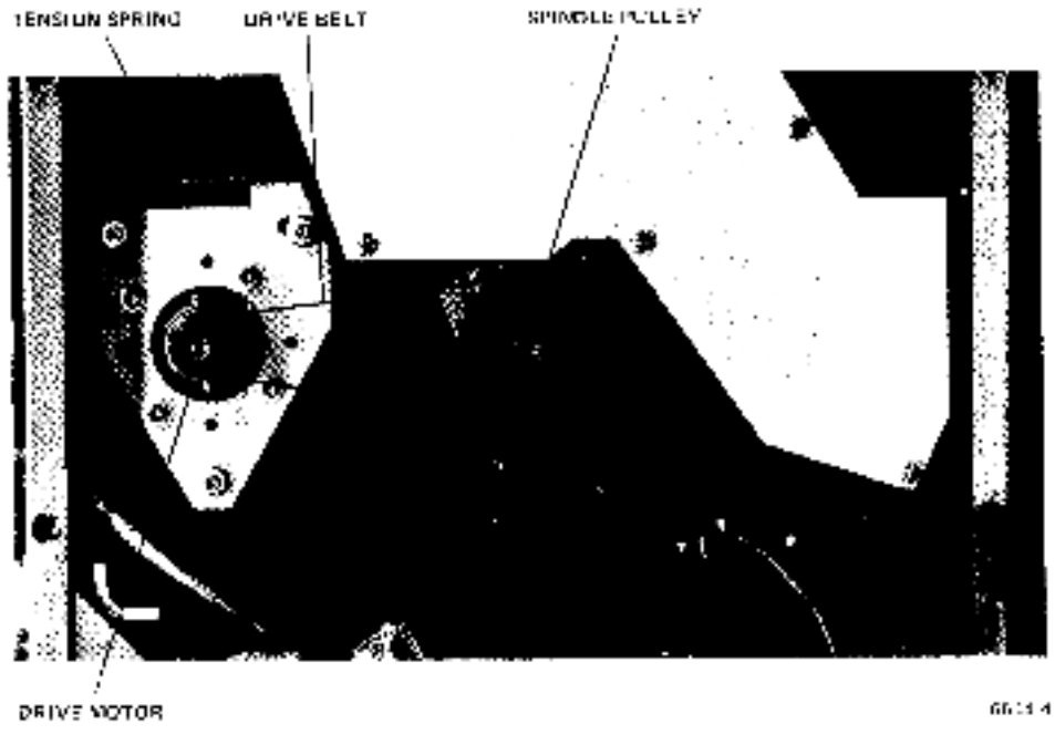
Figure 1-3 Spindle and Drive System
