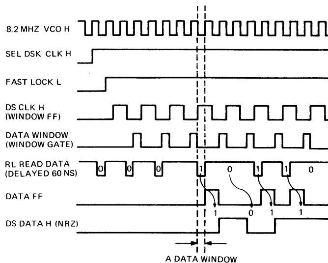
Figure 3-41 Data Separator Timing Diagram
