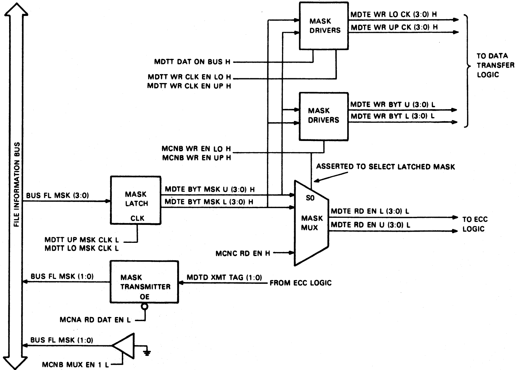
Figure 3-7 Mask Logic
