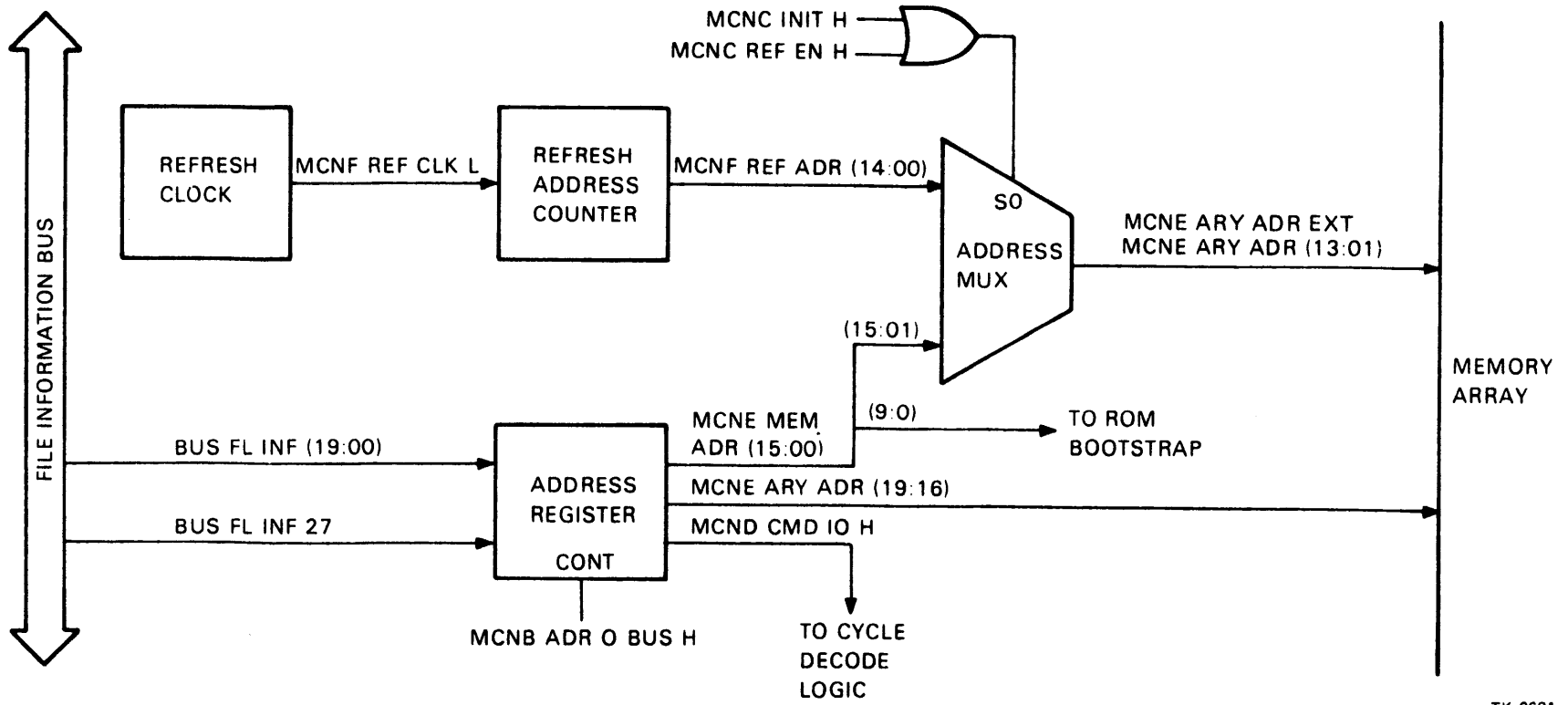
Figure 3-2 Address Logic
