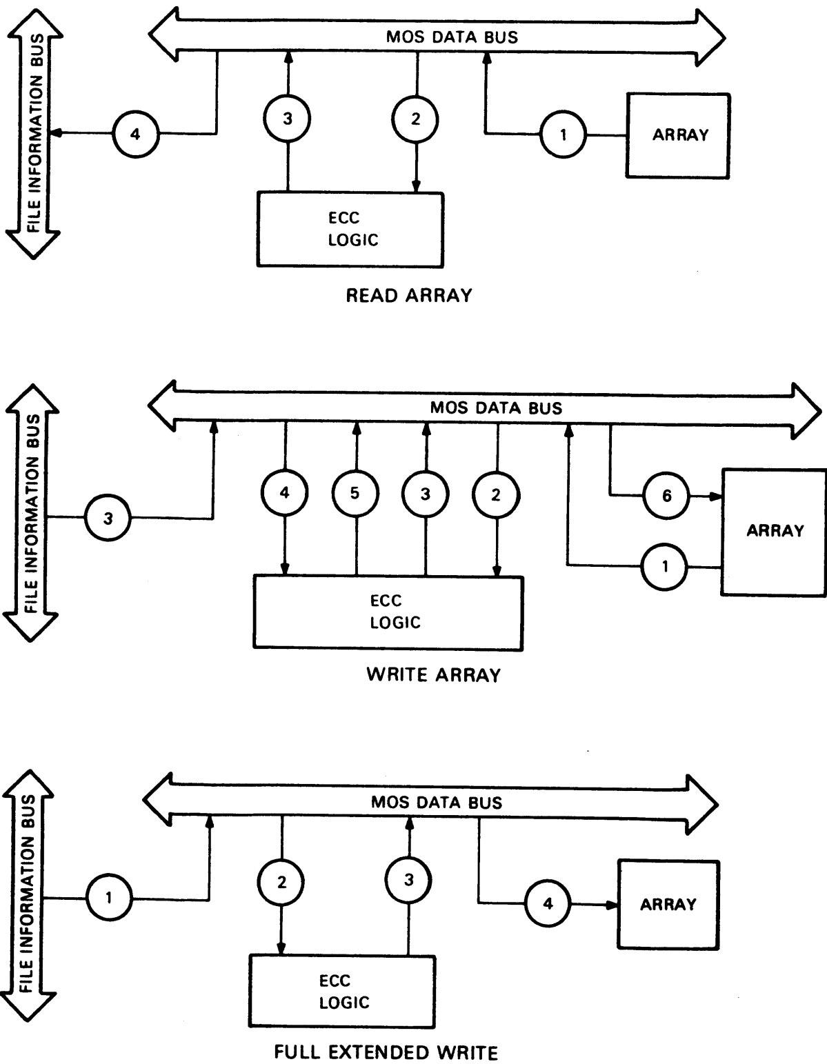
Figure 3-4 Basic Data Flow on the MOS Data Bus
