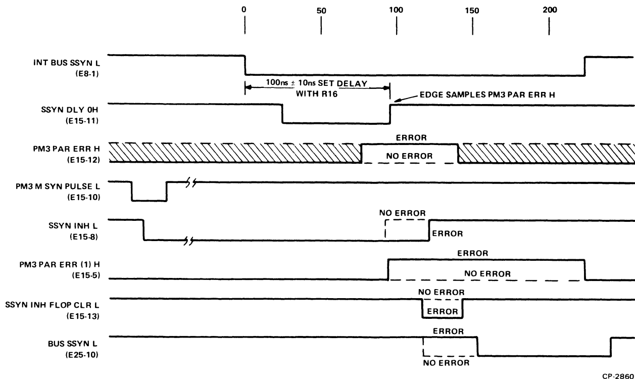
Figure 3-5 Timing Diagram of BUS SSYN Control
