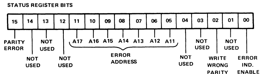
Figure 2-7 Control and Status Register Bit Allocation
