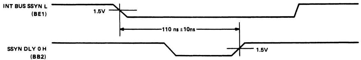
Figure 4-2 Timing Adjust
