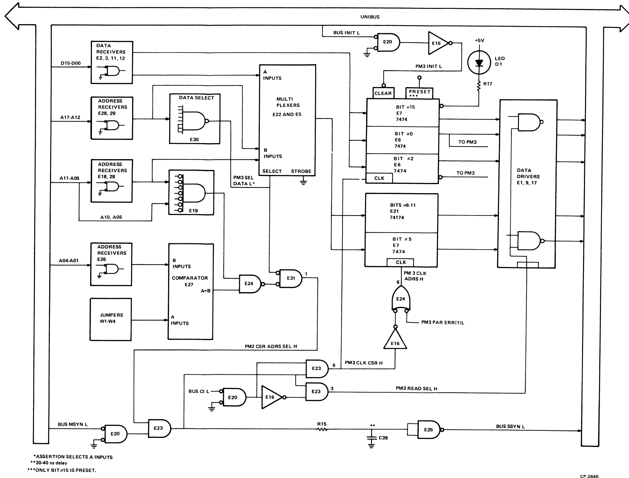
Figure 3-1 CSR Address and Control Circuitry
