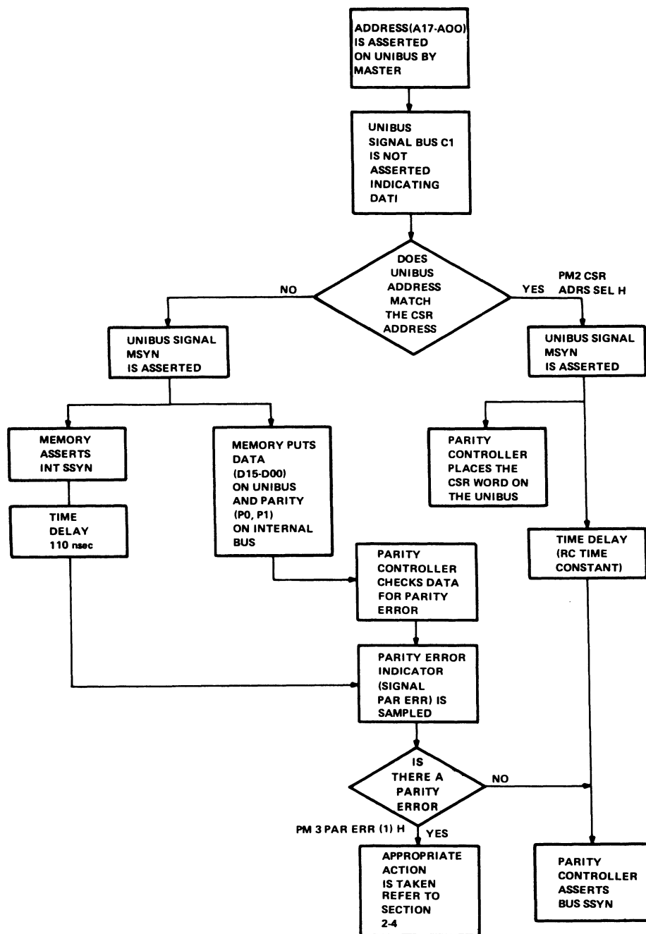
Figure 2-5 DATI Flowchart
