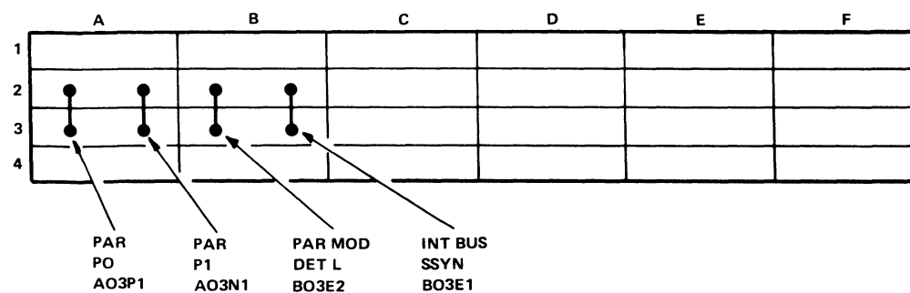
INTERNAL BUS ON 4 SLOT BACKPLANE
