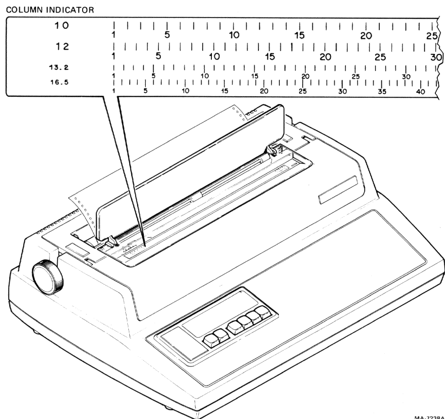
Figure 1-18 Column Indicator
