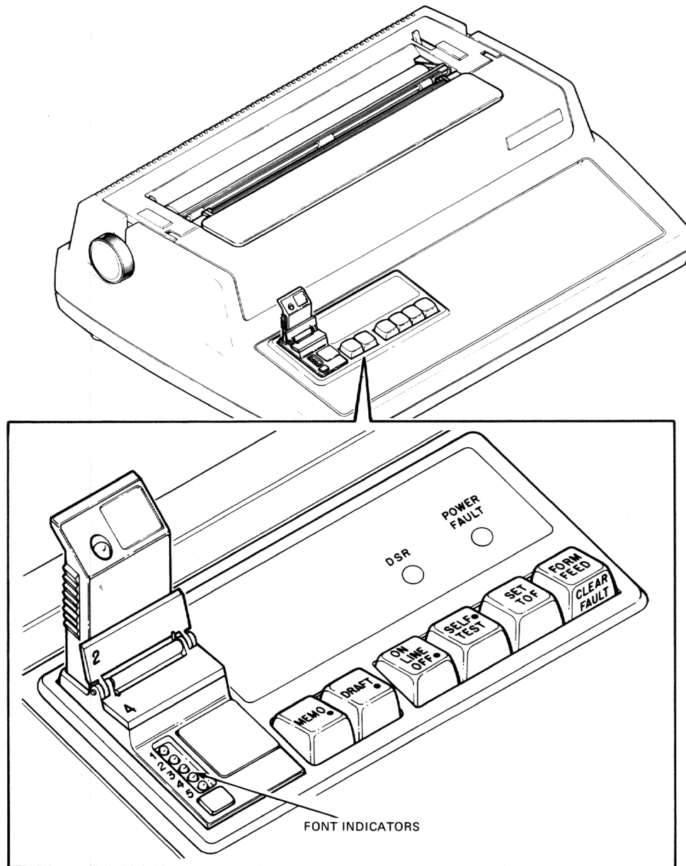
Figure 1-16 Font Indicators
