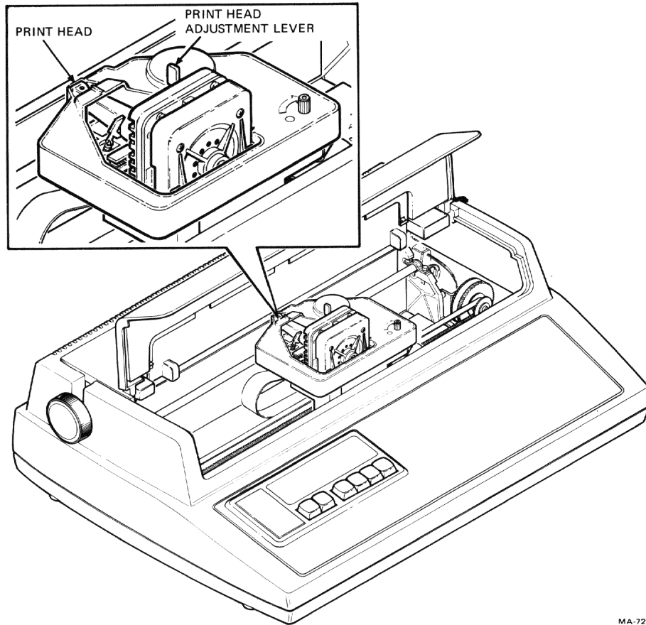
Figure 2-10 Printhead Adjustment
