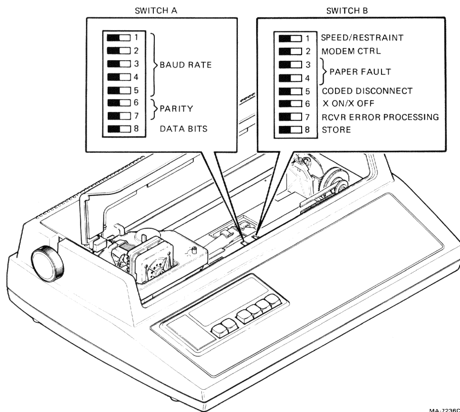
Figure 3-1 Communication Switches
