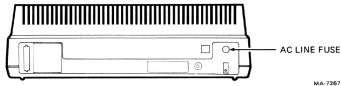
Figure 4-3 AC Line Fuse Location
