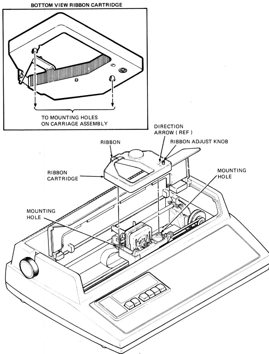
Figure 2-2 Ribbon Cartridge
