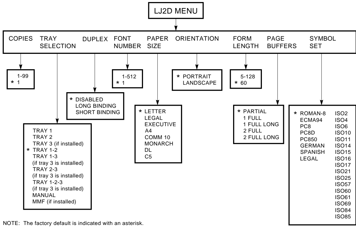
Figure E-2 LJ2D Submenu
