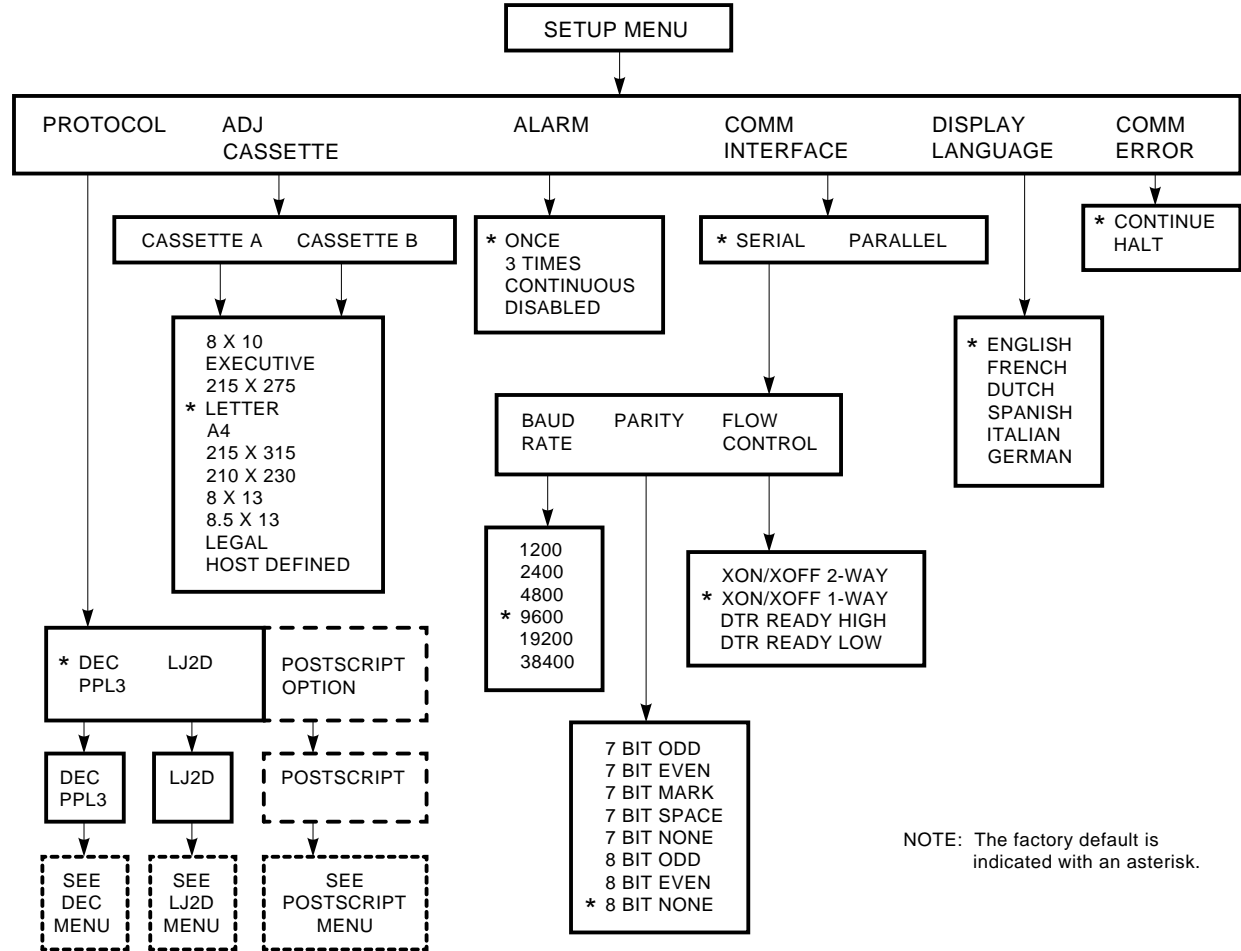
Figure 2-4 Set Up Menu Diagram
