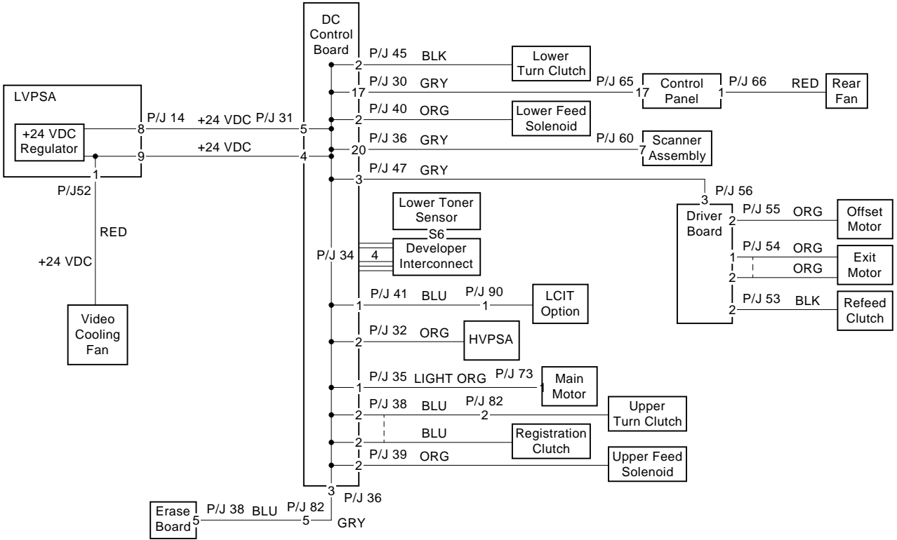
Figure A-6 24 Vdc Distribution
