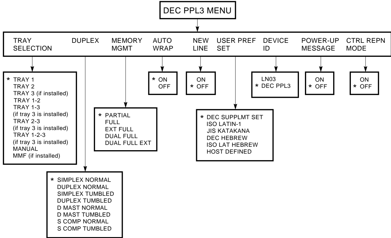
Figure E-1 DEC PPL3 Submenu
