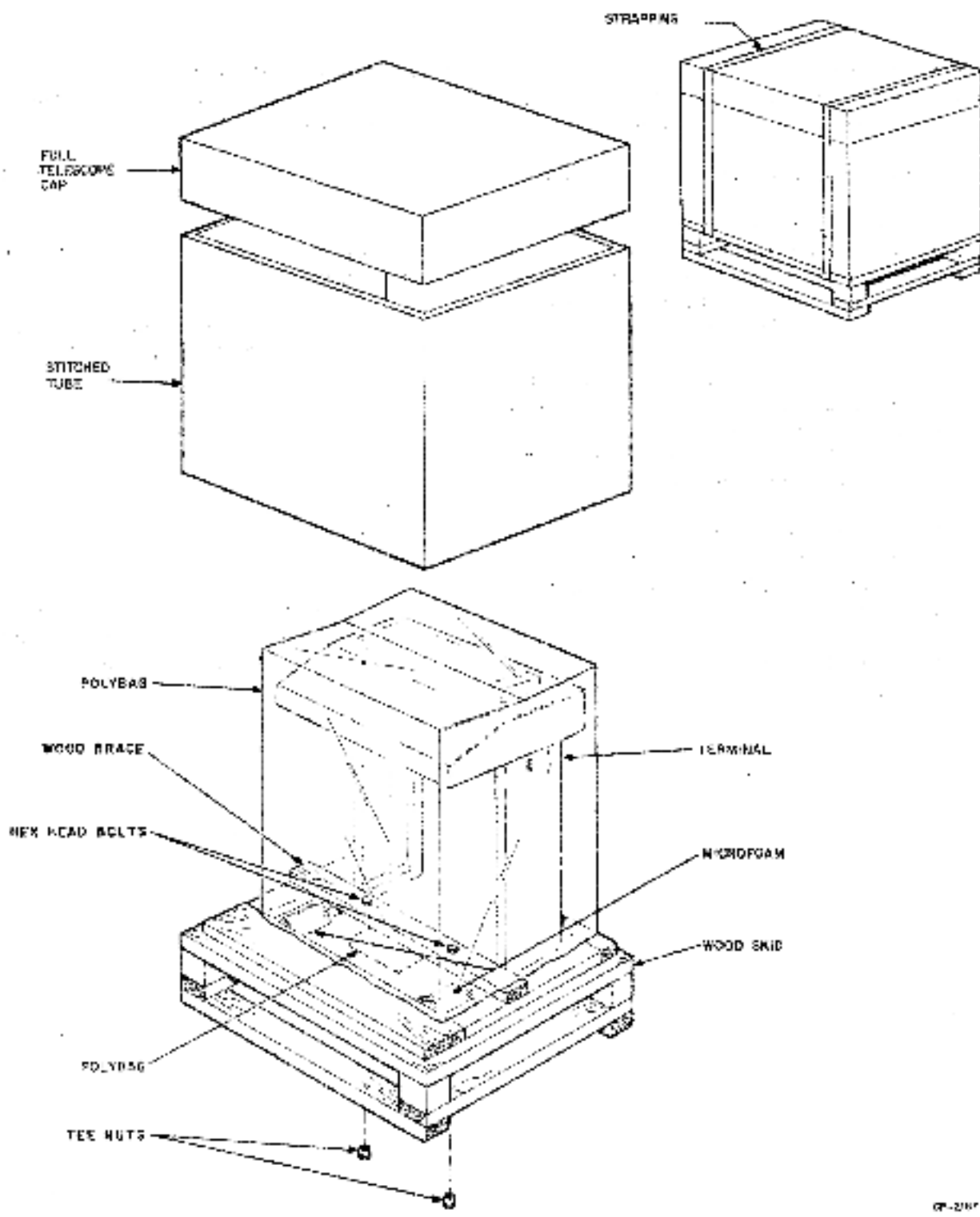
Figure 53 DECwriter Packaging
