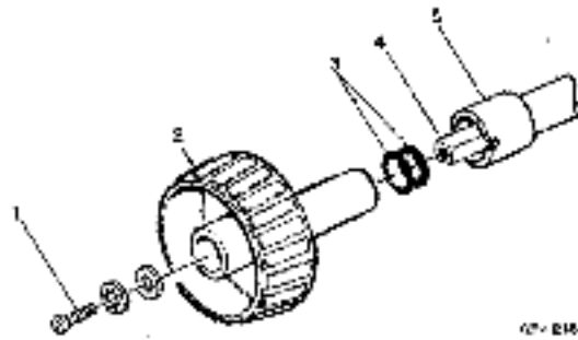
Figure 25 Installation of "C" Ring on Tractor Drive Shaft
