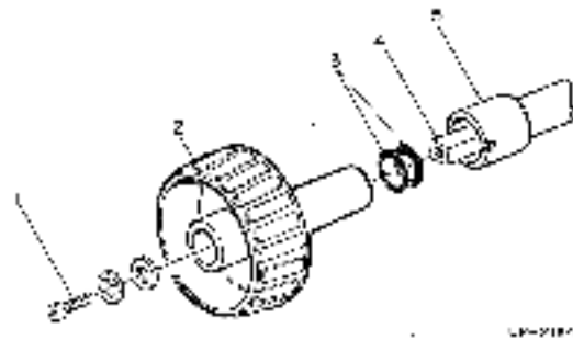
Figure 4B Installation of "O" Ring on Fractor Drive Shaft
