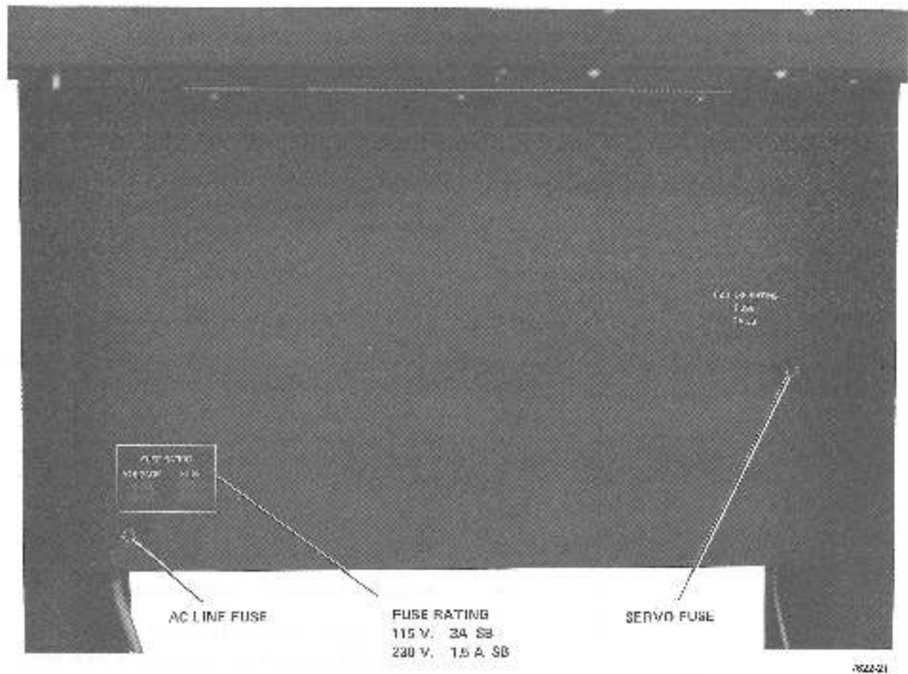
Figure 52 Fuse Locations
