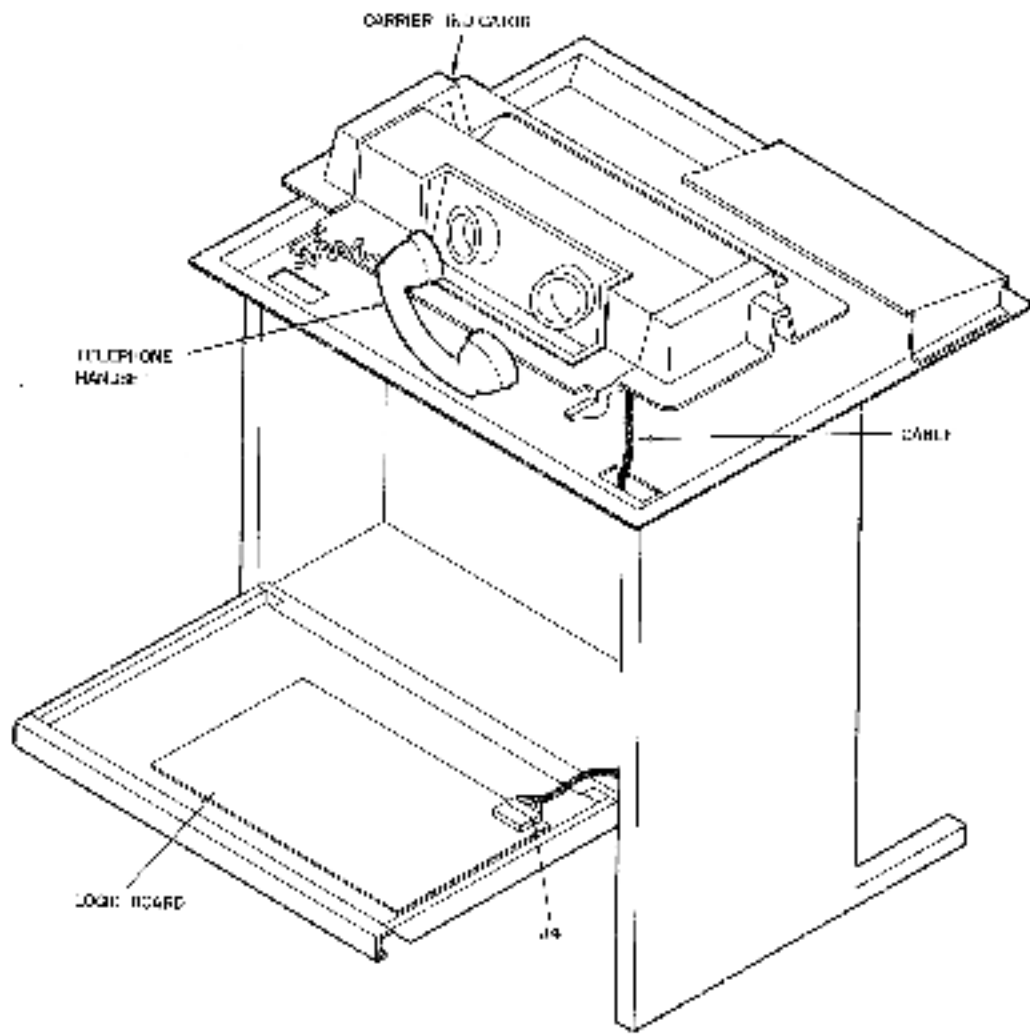
Figure 26 Installation of Acoustical Coupler Option Kit (LAXX-Lfx)
