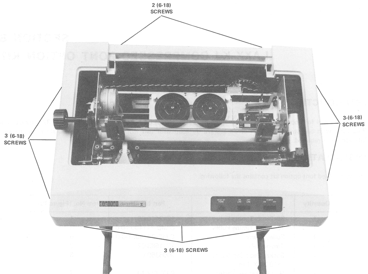
Figure 19 Printer Housing Removal
