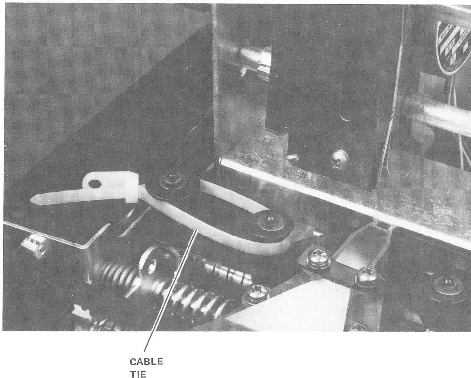
Figure 4 Cable Tie Location
