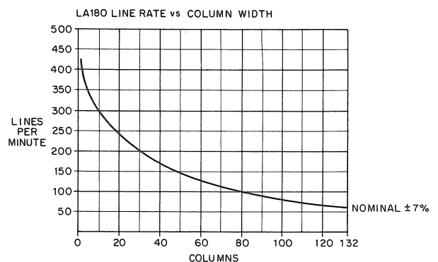
CP-2 250 Figure 9 LA180 Line Rate Versus Column Width
