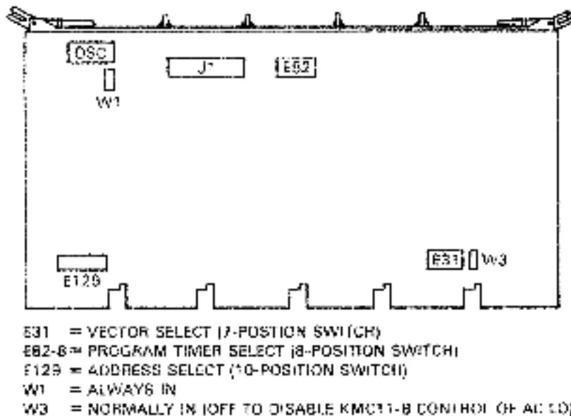
Figure 2-11 KMC11-B (M8206 - Etch Rev E) UNIBUS Microprocessor Board
