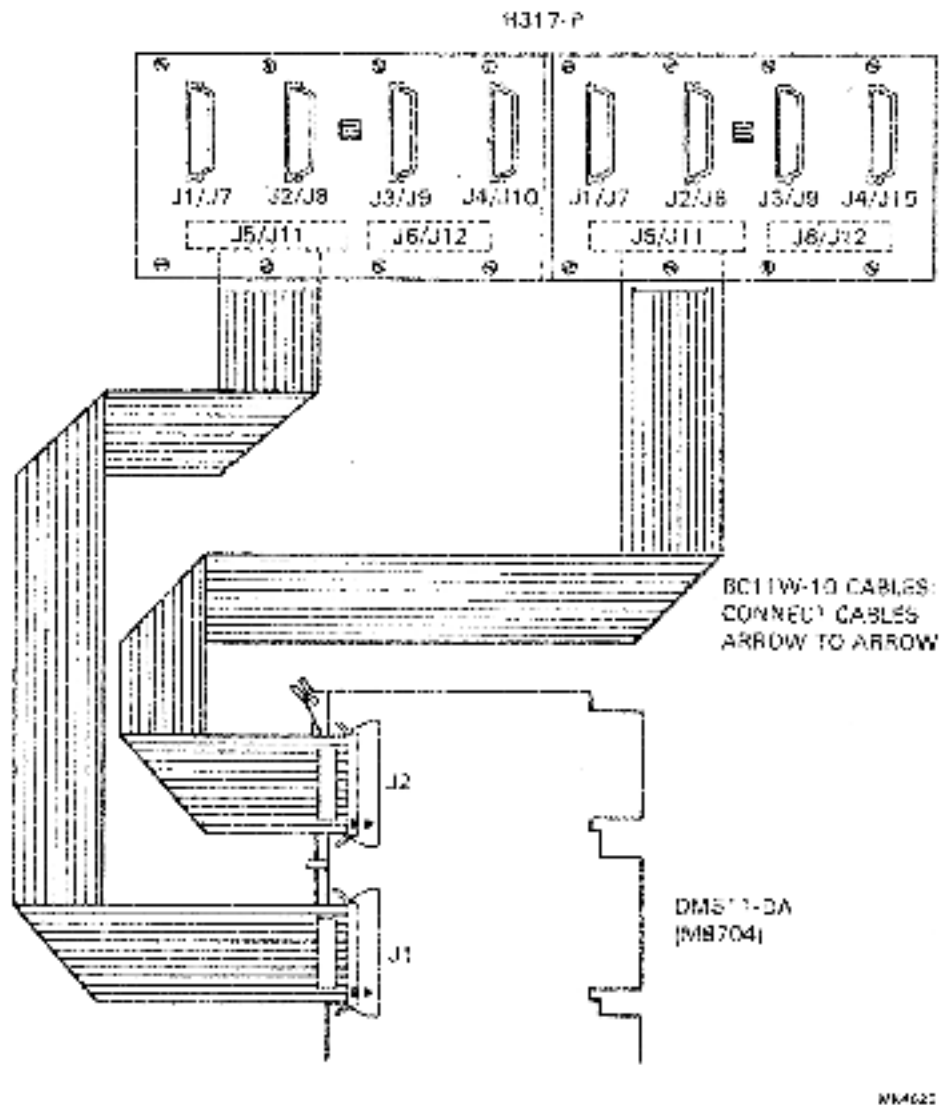
Figure 3-7 DMS11-DA (M8704) Line Unit to H317-P Distribution Panel Cabling
