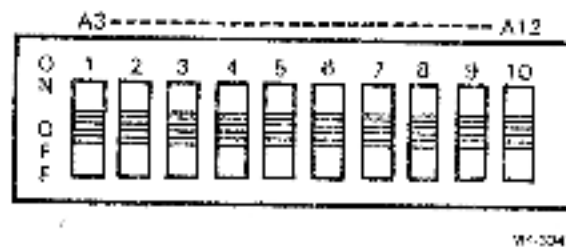
Figure 2-4 KMC11-B (M8206) - Etch Rev C) UNIBUS Microprocessor Address Selection Switch E125
