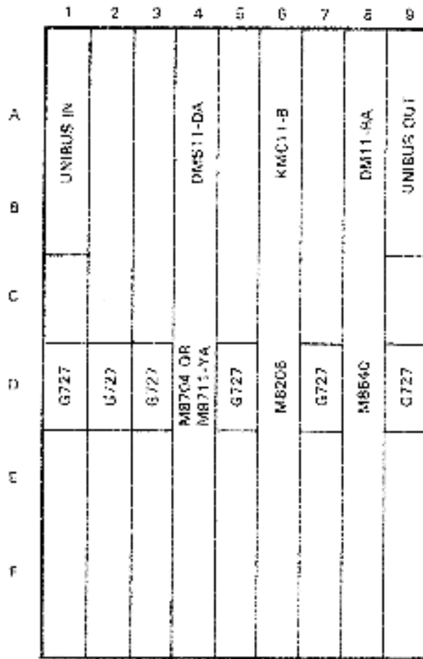
Figure 3-2 DD11-DK Nine-Slot Backplane (Viewed from the Backplane Pin-Side)
