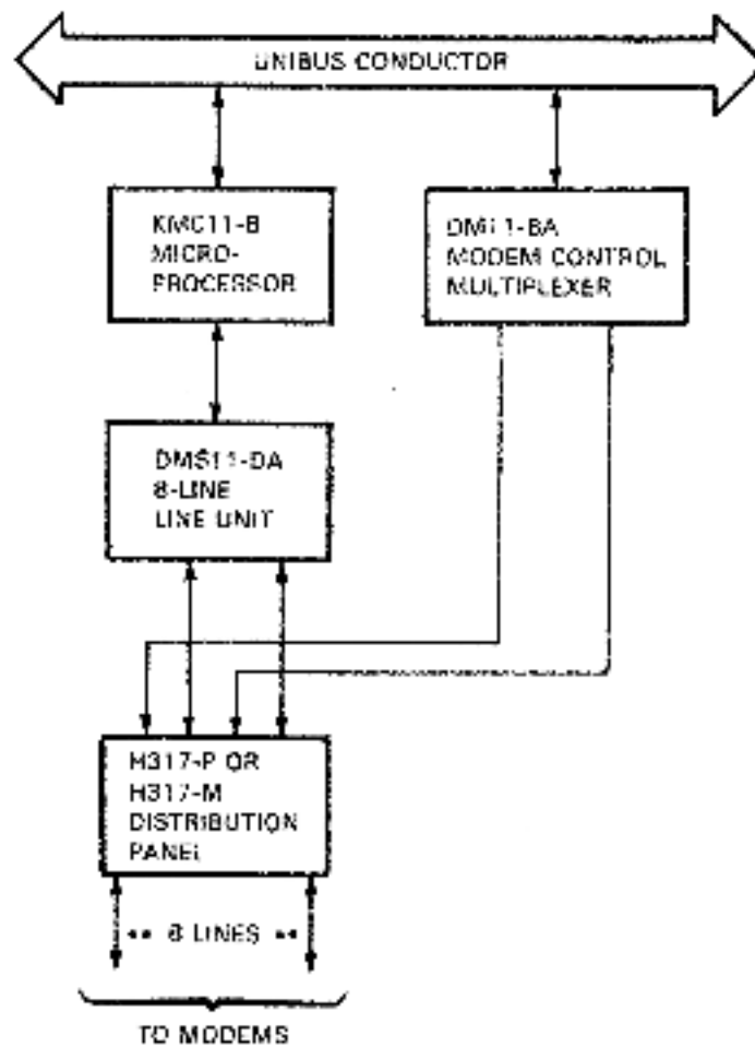
Figure 3-4 KMS11-BD/BE Communications Processor UNIBUS Connector Interface
