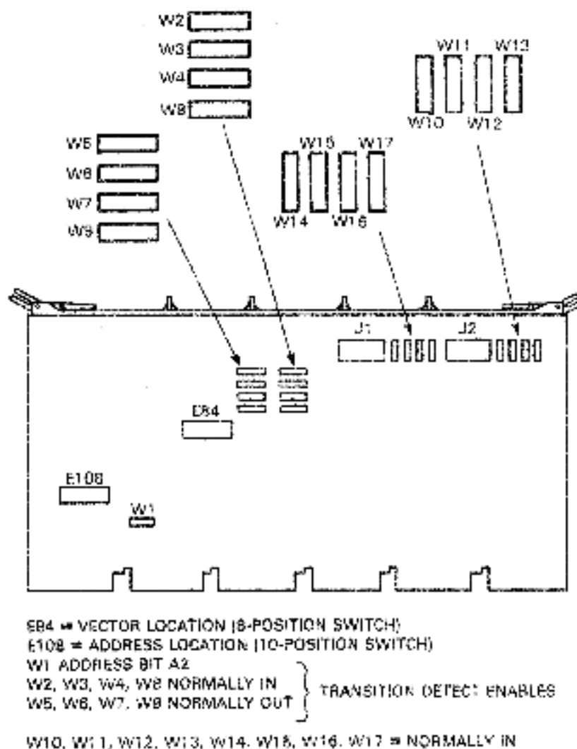
Figure 2-16 DM11-BA (M8640 - Etc Rev B) Modem Control Multiplexer Board
