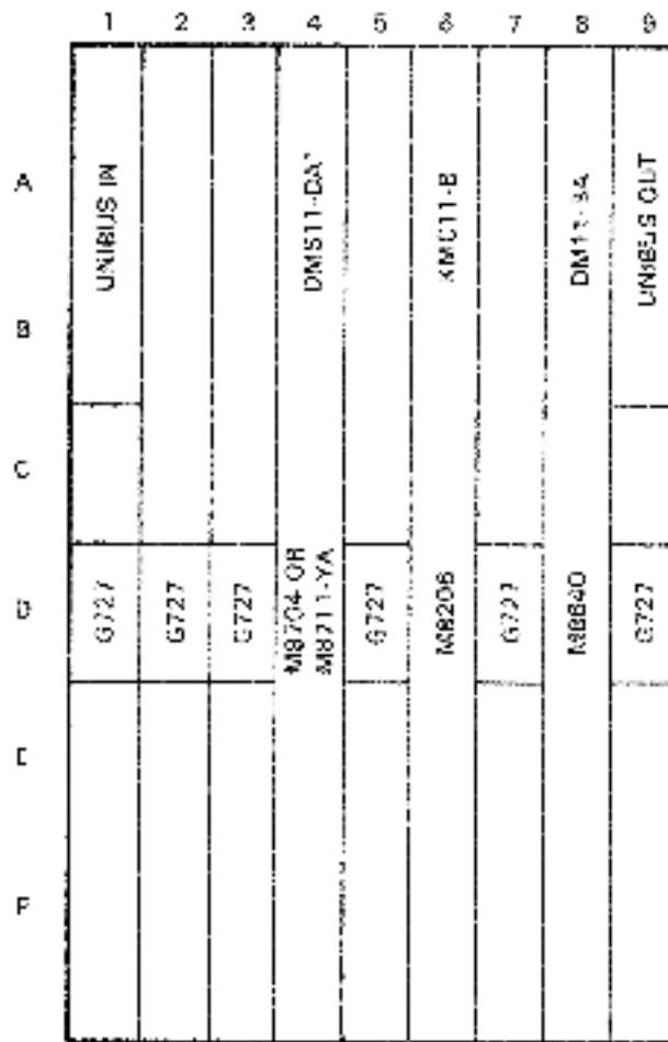
Figure 2-31 DD11-DK Nine-Slot Backplane with KMS11-BD/BE Communications Processor Board Locations (Viewed from the Backplane Pin-Side)
