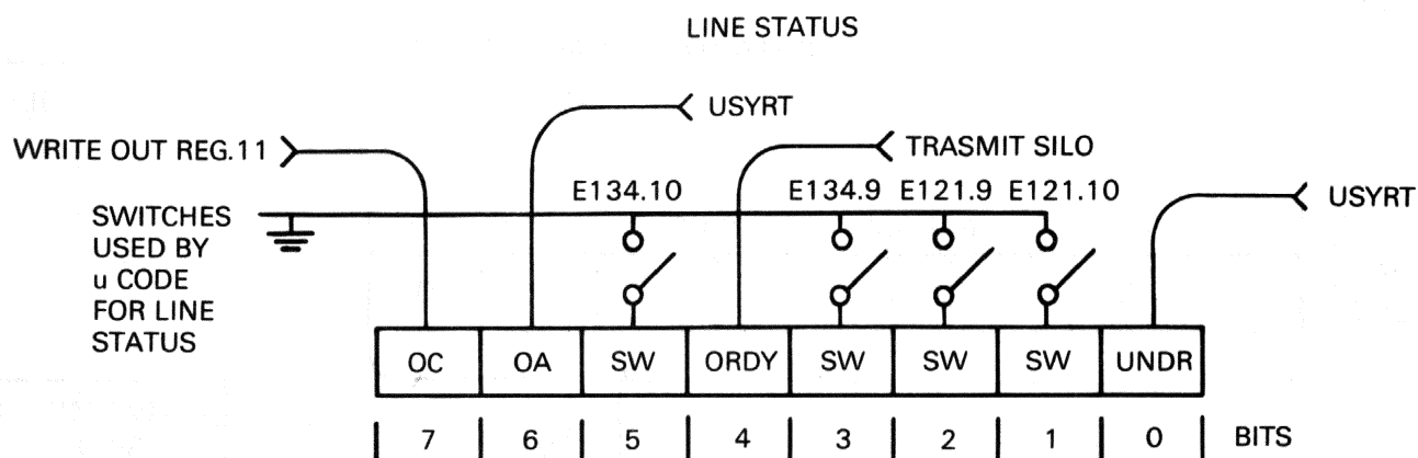
Figure 3-8 IBUS Register 11
