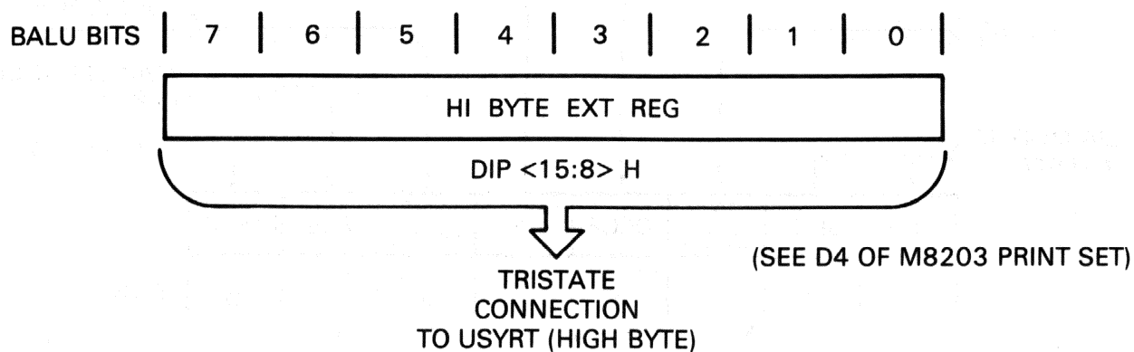
Figure 3-19 OBUS Register 16
