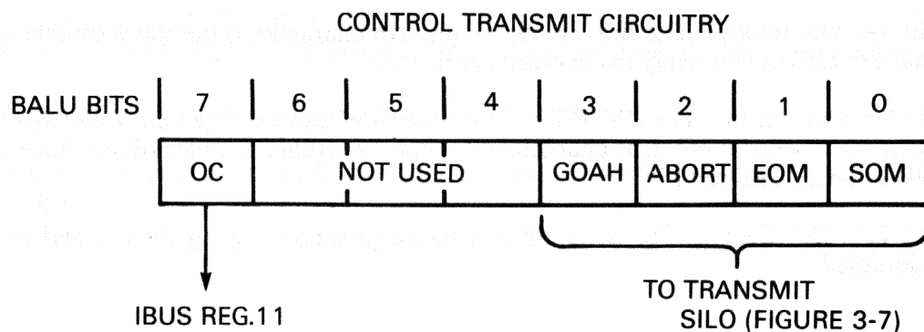
Figure 3-9 OBUS Register 11
