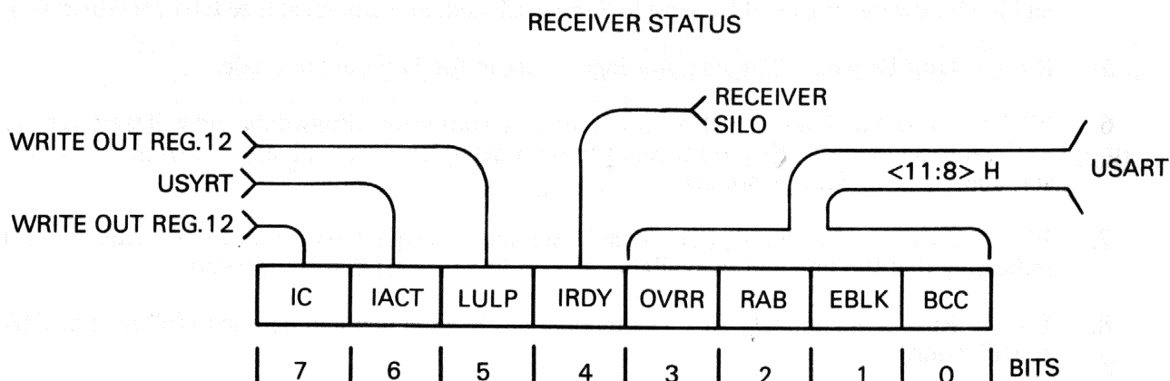
Figure 3-10 IBUS Register 12
