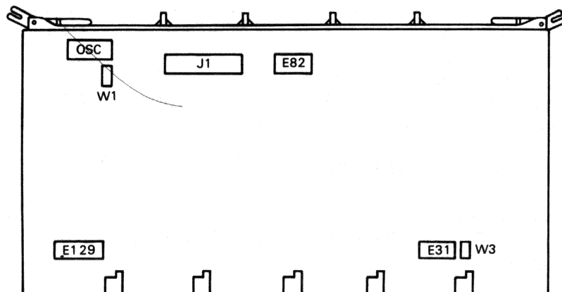
Figure 2-1 M8206 (KMC11-B) Switch and Jumper Locations
