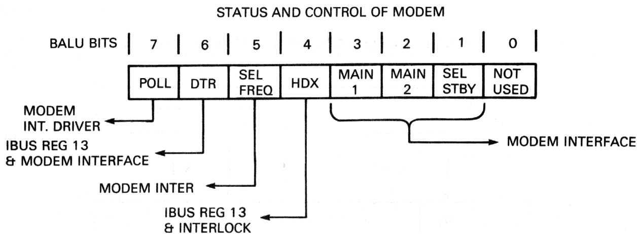
Figure 3-13 OBUS Register 13
