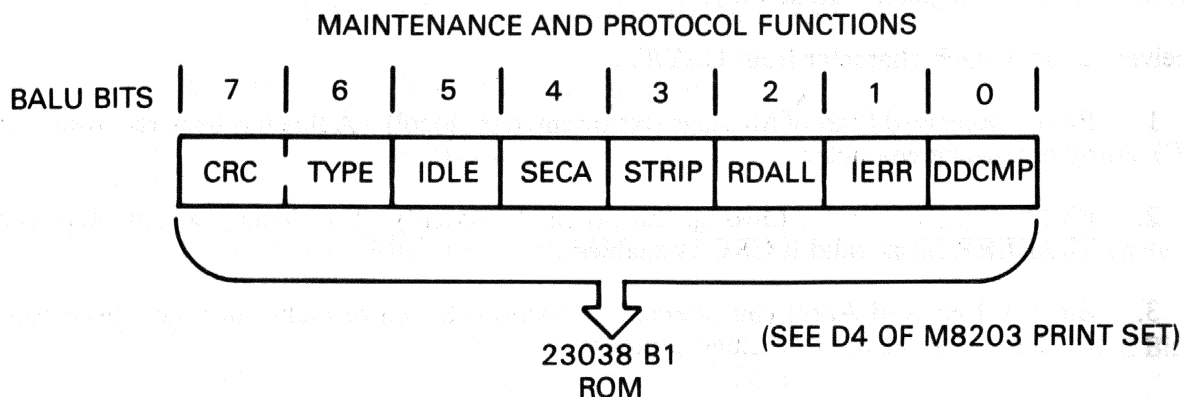
Figure 3-21 OBUS Register 17
