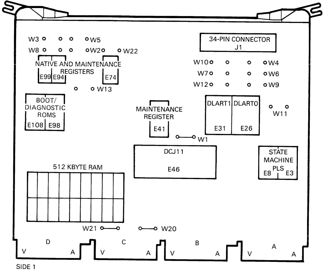
Figure 2-2: KDJ11-D/S Module - Early version (M7554)
