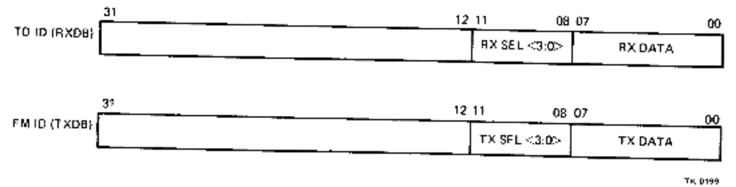
Figure 2-5 Use of the TO ID and FM ID Registers When the VAX-11/780 CPU is Running
