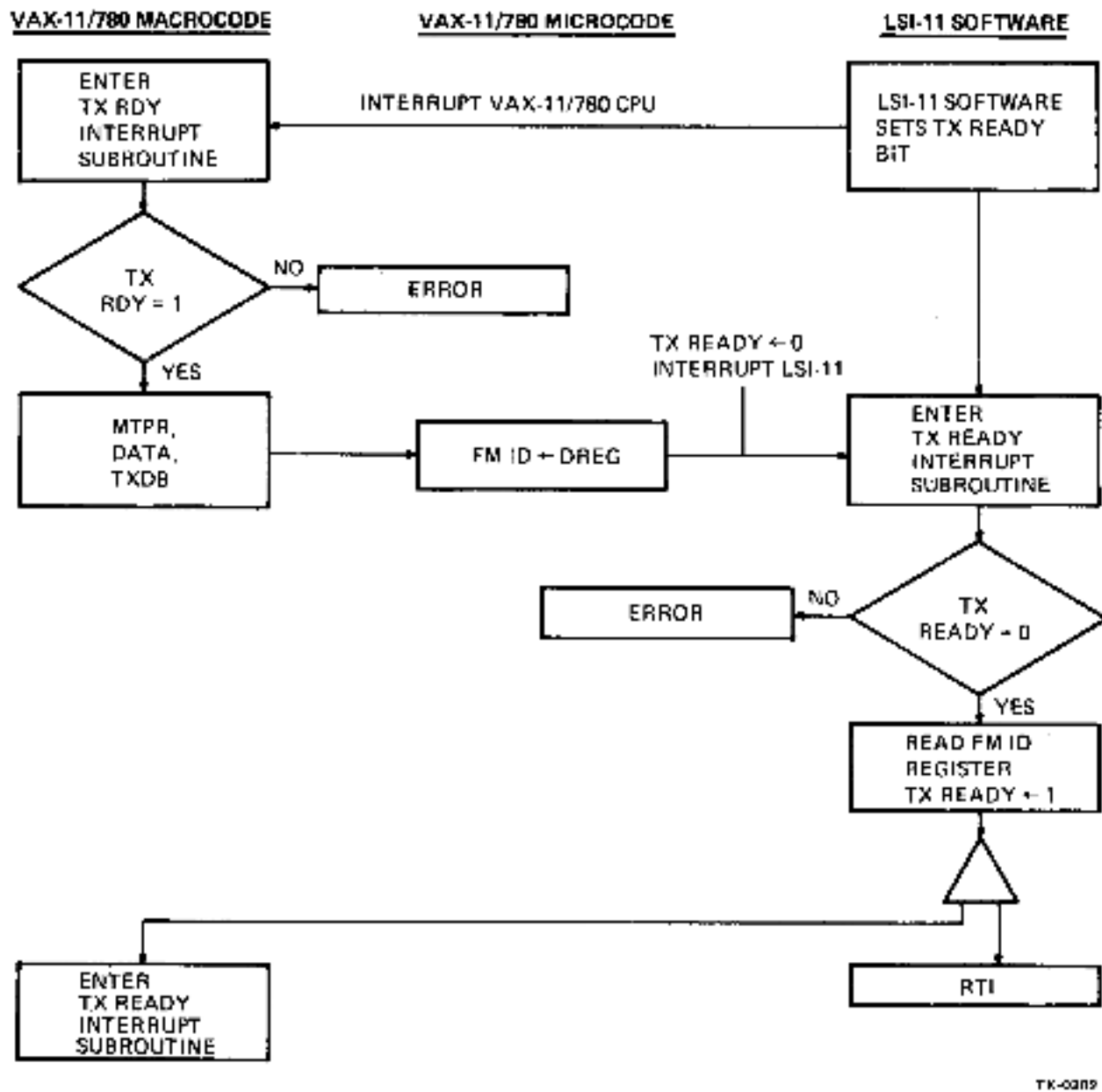
Figure 2-9 VAX-11/780 Sends a Character to the LSI-11, Flowchart
