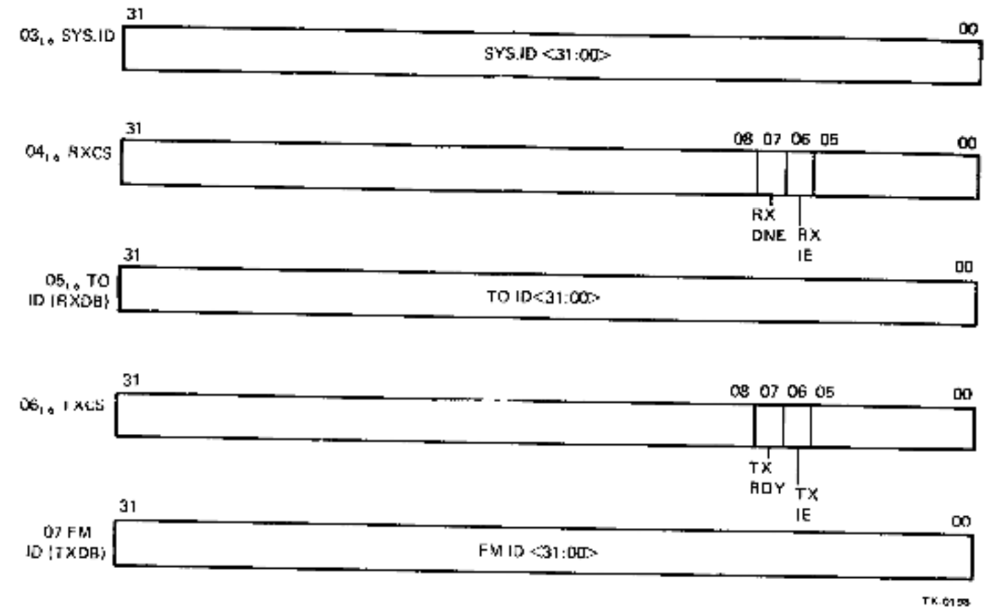
Figure 2-4 ID Bus Registers on the CIB
