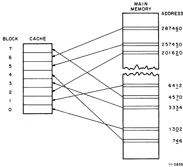
Figure 1-3 Direct Mapping Cache Memory System
