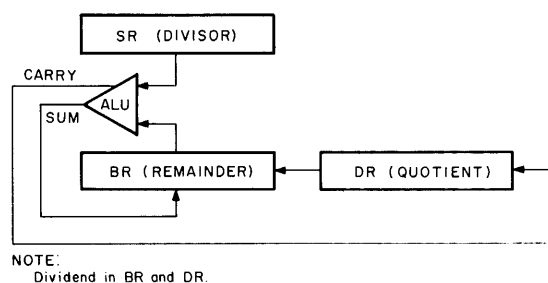
Figure 1-9 Divide Instructions
