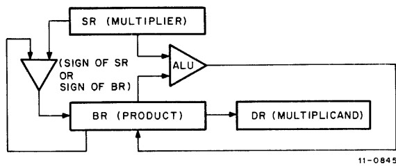
Figure 1-7 Multiply Instruction
