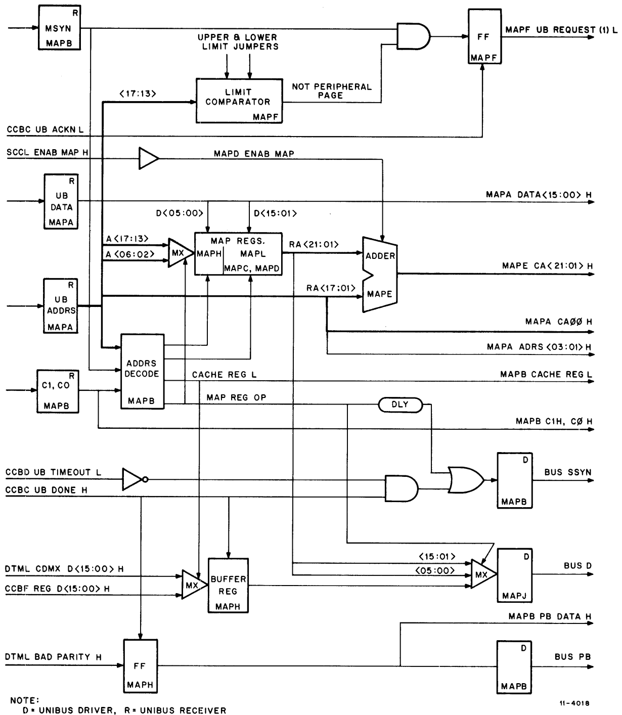
Figure 2-2 Unibus Map Block Diagram
