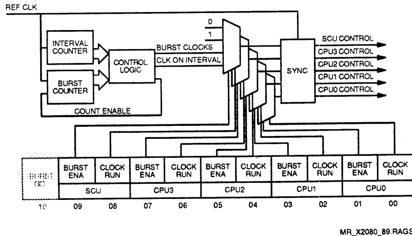
Figure 2-16 CCI Clock Control Implementation
