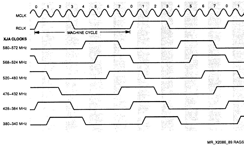
Figure 2-23 XJA Clock Timing
