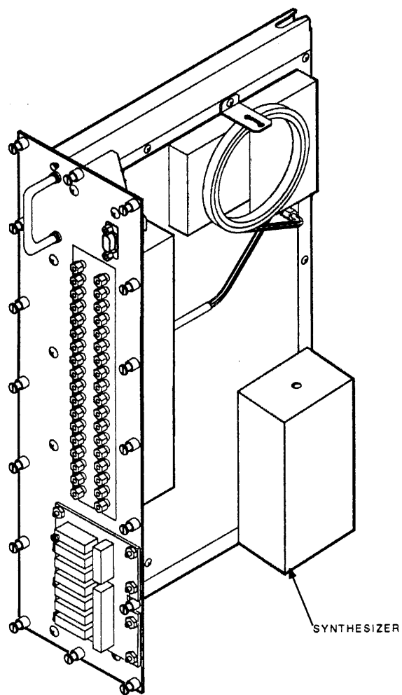
Figure 1-1 MCM Assembly
