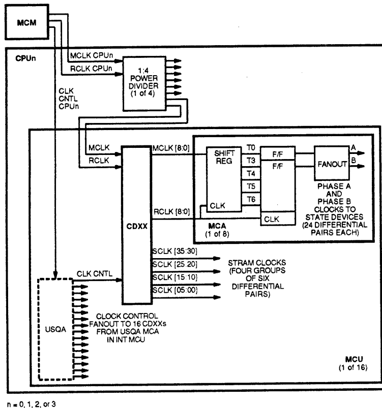
Figure 1-3 Clock Distribution in a CPU
