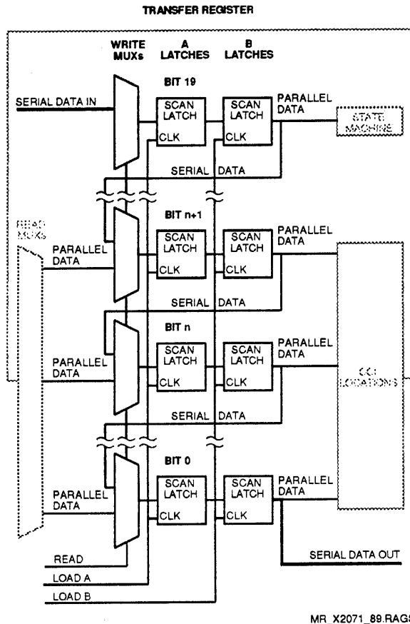
Figure 2-6 CCI Transfer Register Implementation
