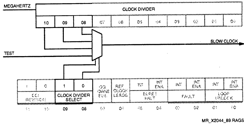
Figure 2-15 CCI Clock Divider
