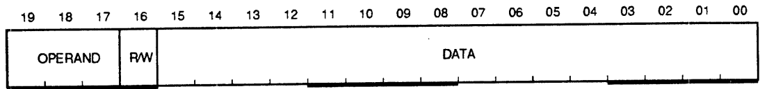
Figure 2-3 CCI Transfer Register Format
