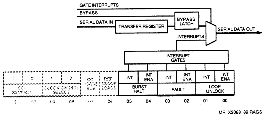
Figure 2-17 CCI Interrupts
