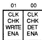
Figure 3-13 CDXX Clock Check Control Register Format
