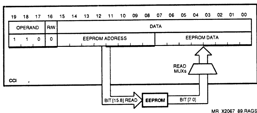
Figure 2-14 CCI EEPROM Read
