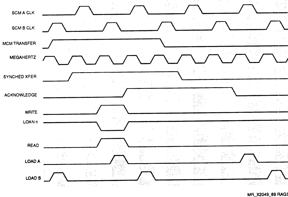
Figure 2-7 CCI Transfer Register Timing
