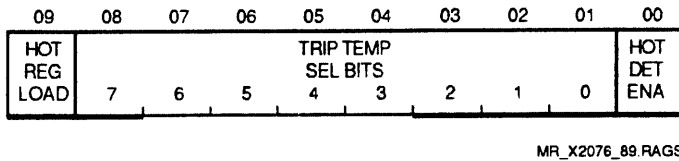
Figure 3-12 CDXX HOT Control Register Format
