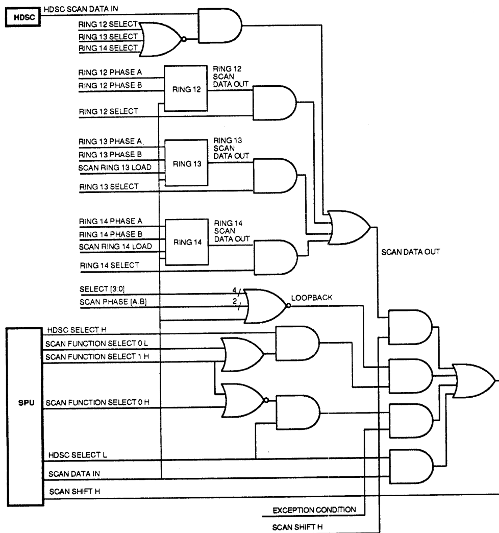
Figure 3-9 CDXX Scan Data Out
