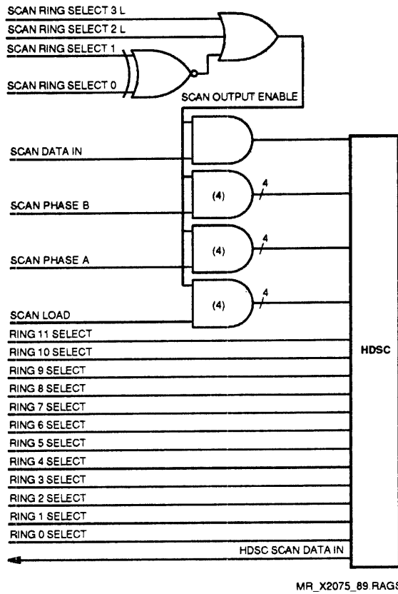
Figure 3-10 CDXX-to-HDSC Scan Signals
