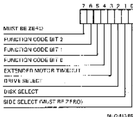
Figure 6-10: Register RX5CS0 Command Function Format
