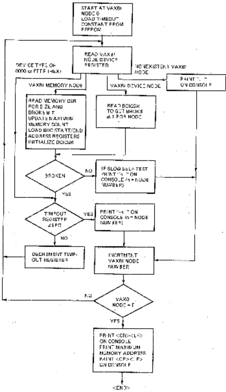
Figure 3-9: System Initialization Sequence
