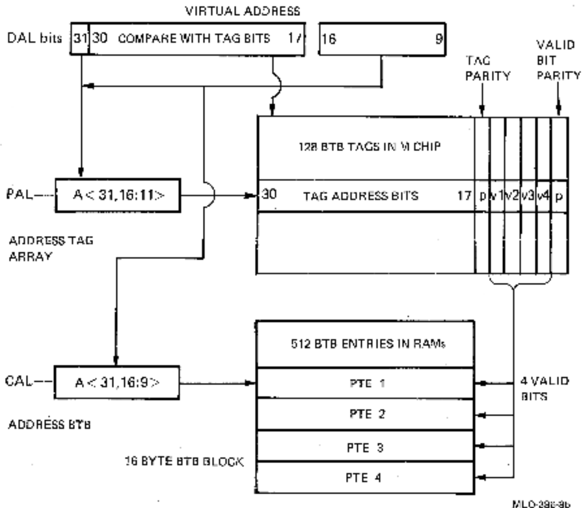
Figure 2-2: BTB and BTB Tag Addressing
