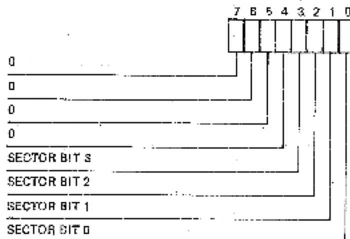
Figure 6-13: RX5CS2 Command Function Format: Sector Register
