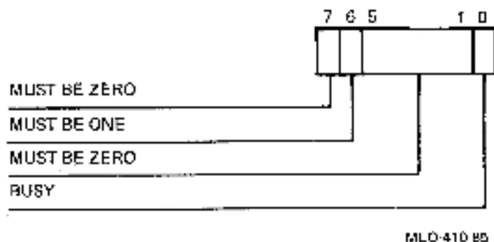
Figure 6-7: Watch Chip CSR A Format
