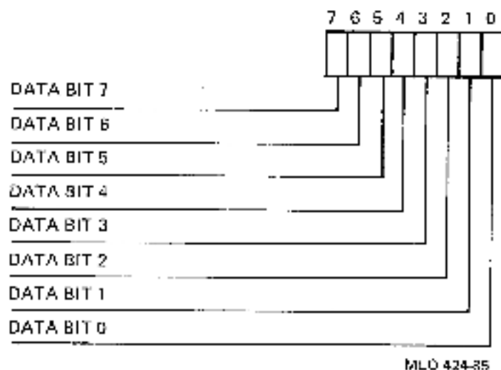
Figure 6-21: RX5FB Format: Fill Sector Buffer Register
