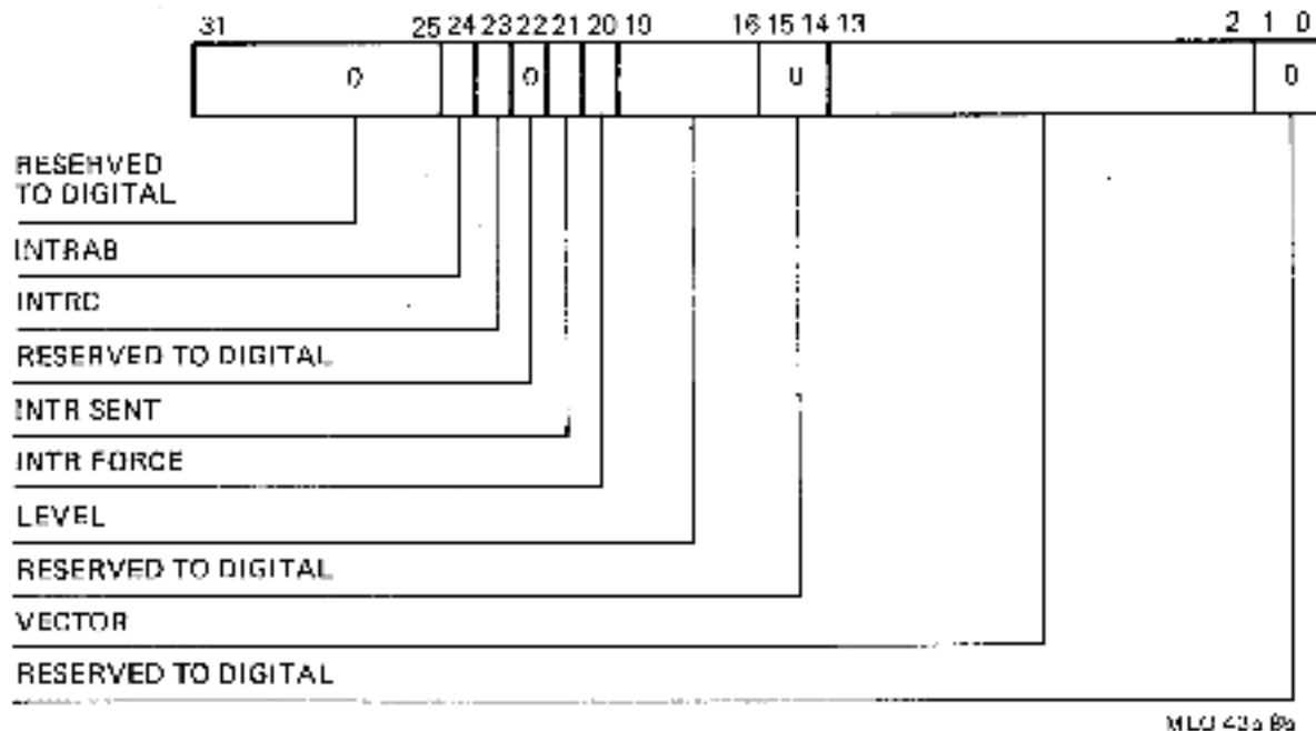
Figure D-4: Error Interrupt Control Register
