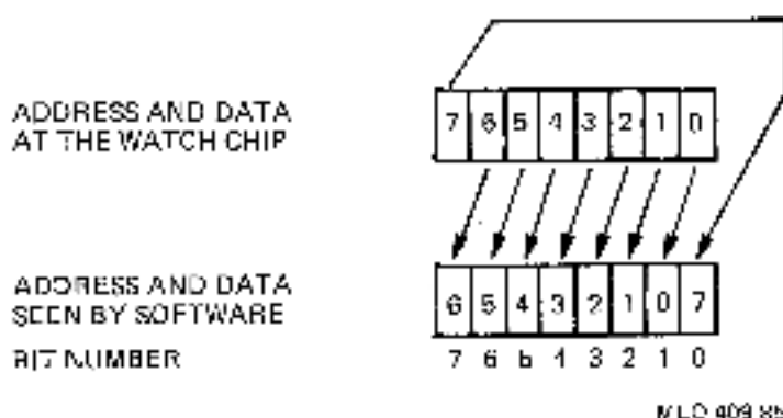
Figure 6-6: Watch Chip Bit Rotation on the PCI Bus
