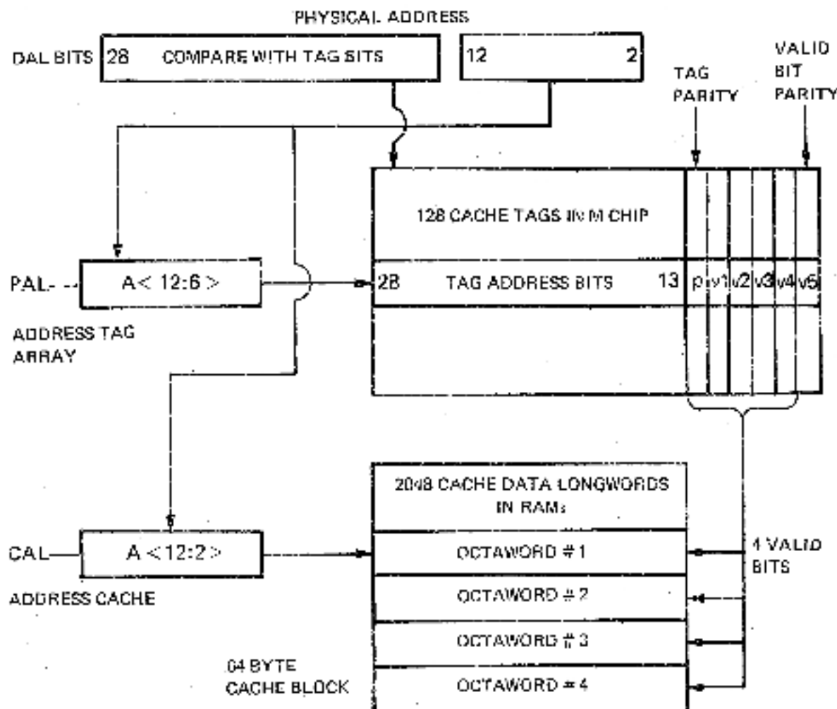
Figure 2-4: Cache and Cache Tag Addressing
