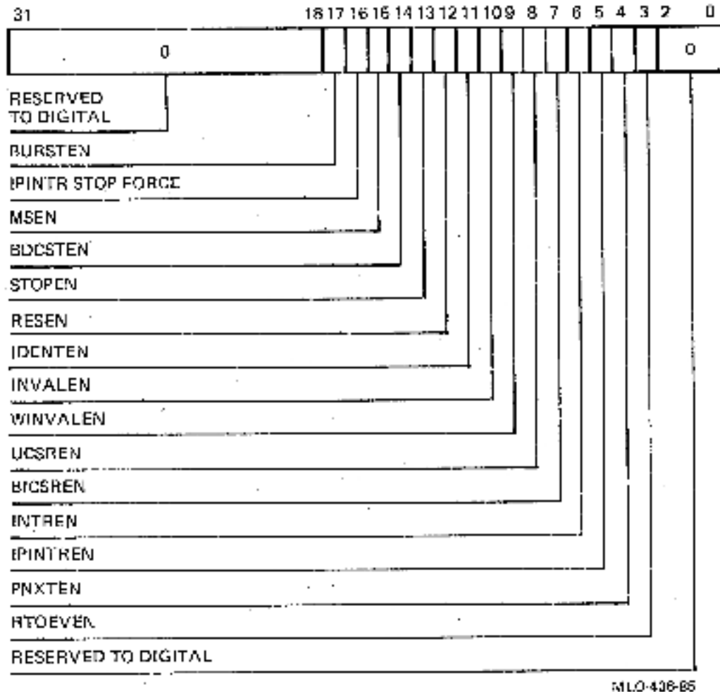
Figure D-5: BCI Control and Status Register
