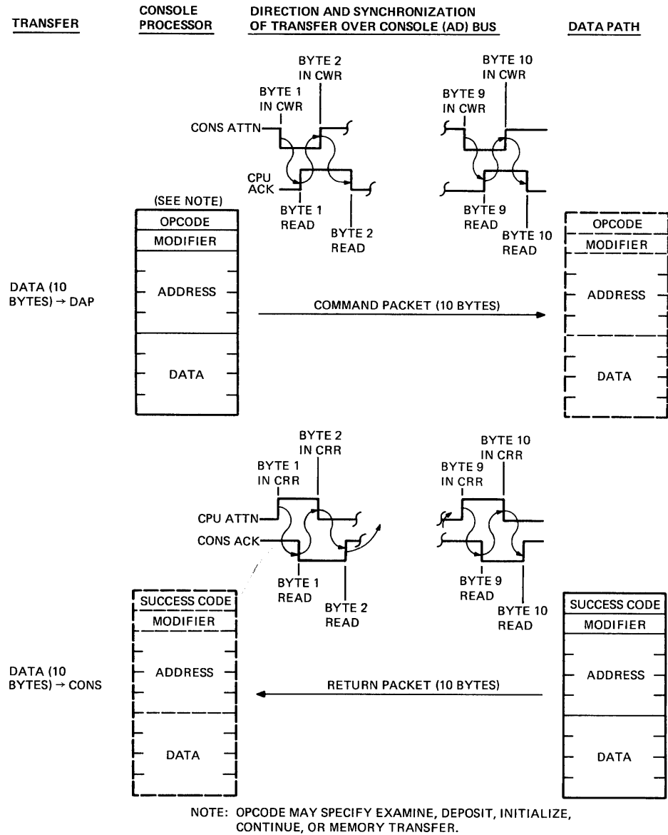
Figure 2-22 Communications Over Console Bus in Console Mode (Sheet 1 of 2)
