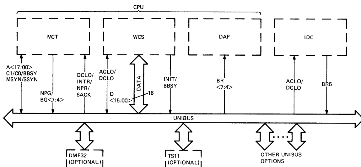
Figure 1-8 VAX-11/730 UNIBUS
