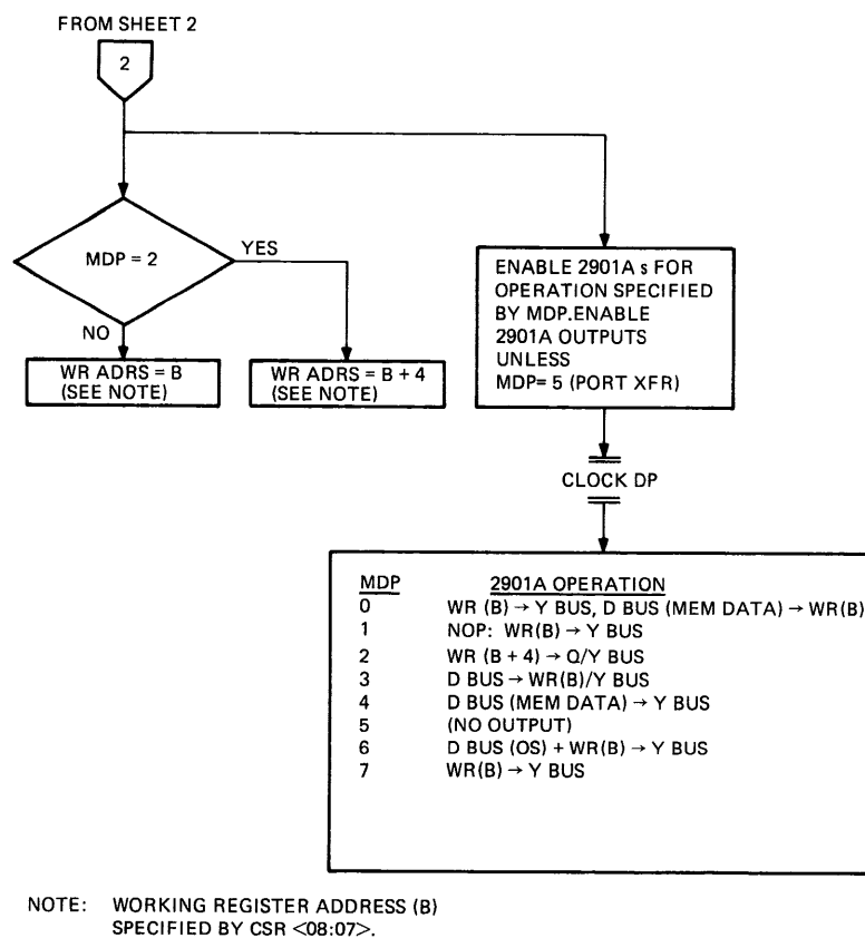
Figure 6-23 MOVE Microinstruction Flow Diagram (Sheet 3 of 3)
