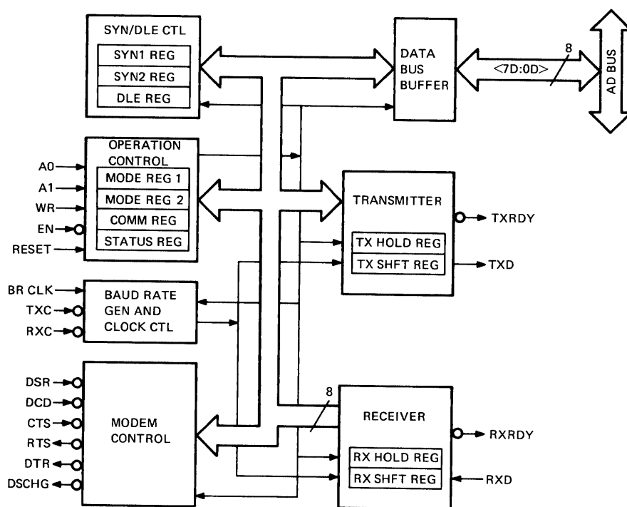
Figure 2-4 2651 USART
