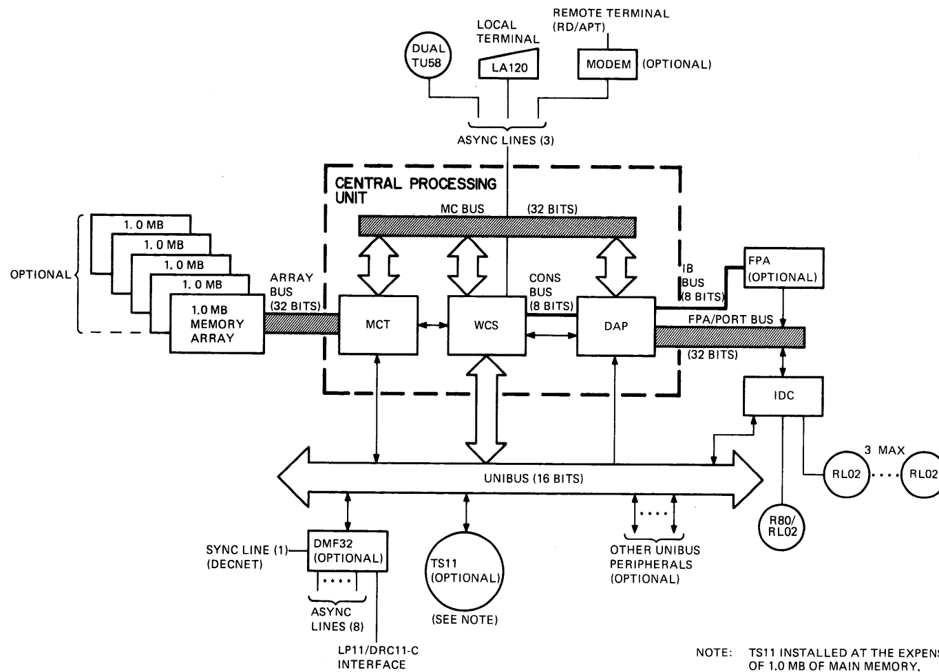
Figure 1-1 VAX-11/730 System
