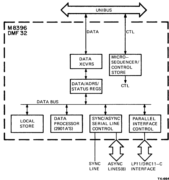
Figure 1-5 DMF32
