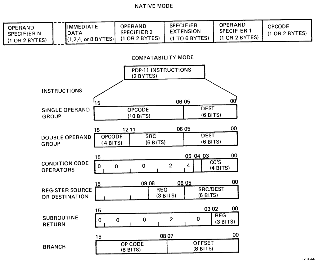
Figure 5-2 Basic Instruction Formats (Native and Compatibility Modes)
