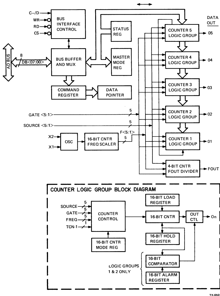
Figure 2-10 9513 Interval Timer Block Diagram
