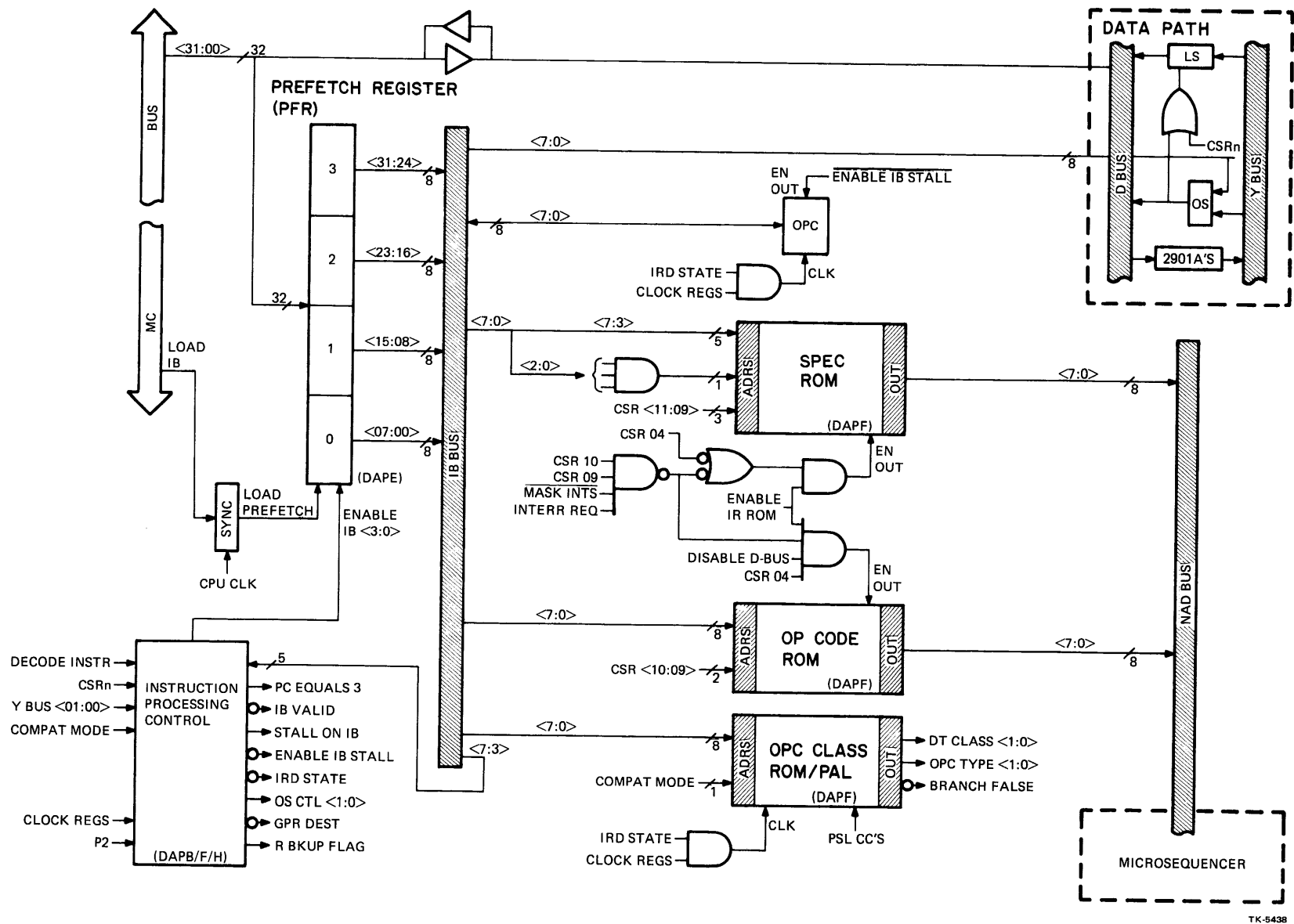
Figure 5-1 Instruction Processing Hardware Block Diagram
