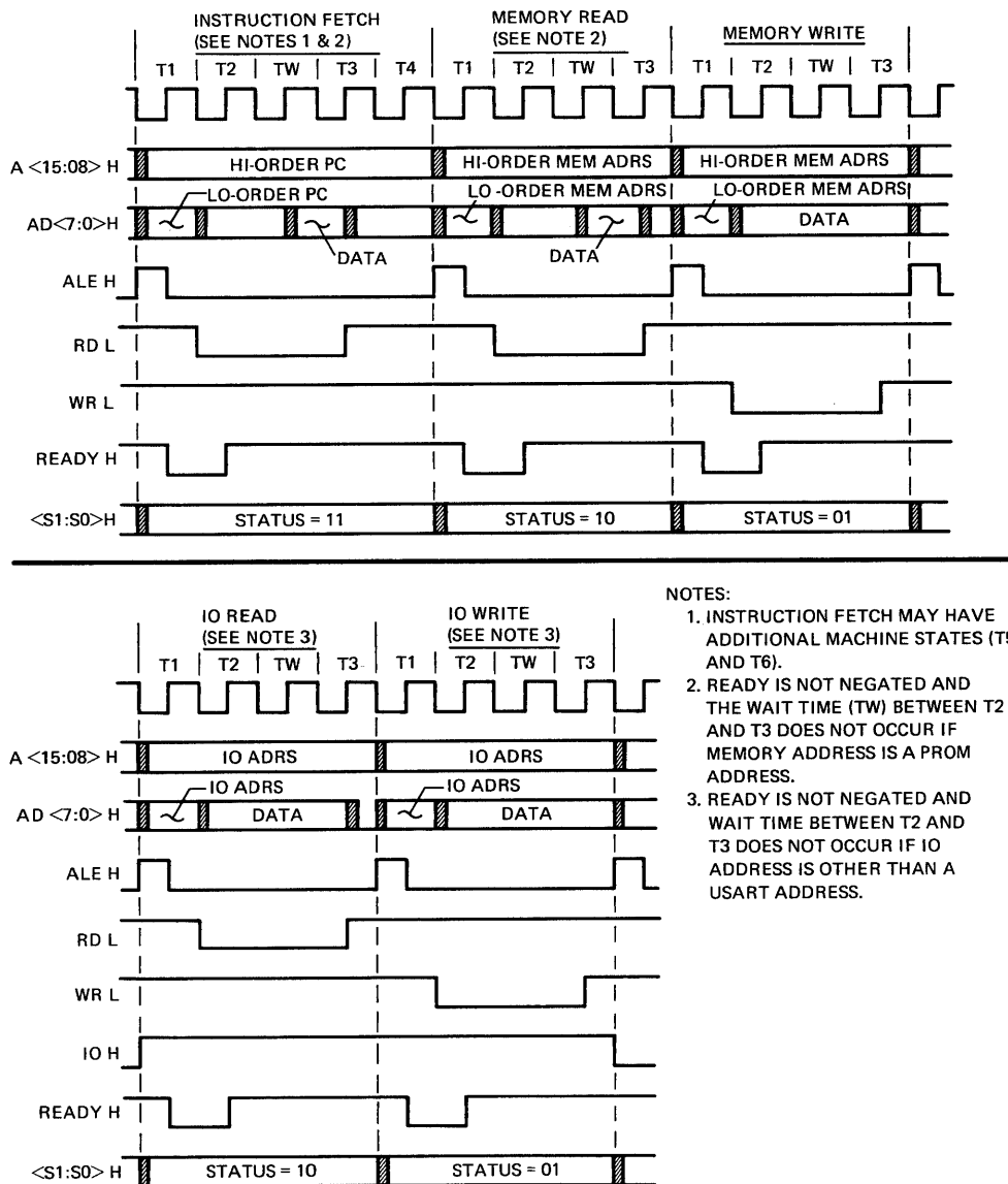
Figure 2-3 8085A Machine Cycles Timing Diagram
