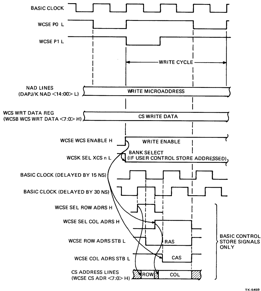
Figure 4-6 Control Store Write Operation Timing Diagram (Sheet 2 of 2)
