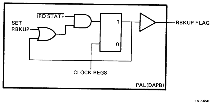
Figure 5-12 RBKUP FLAG Control Logic
