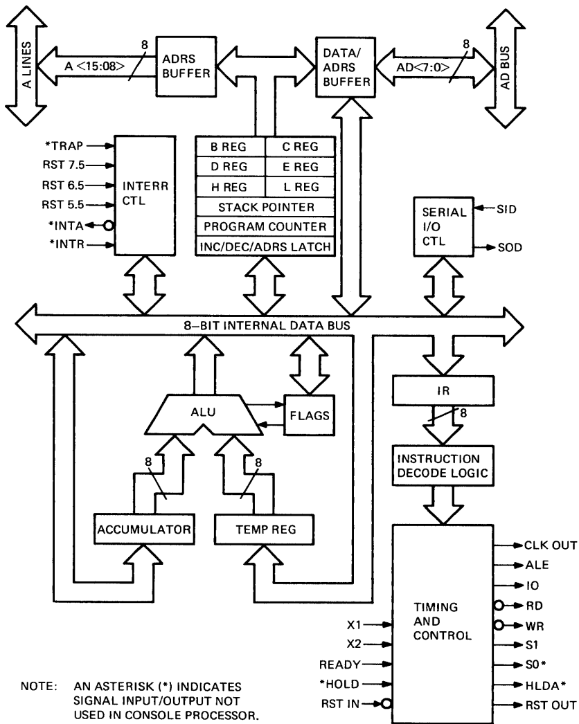
Figure 2-2 8085A Microprocessor
