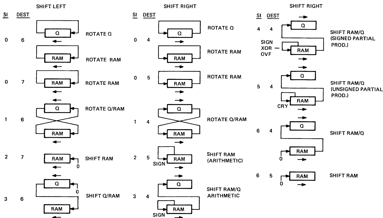
Figure 6-9 Shift Configurations
