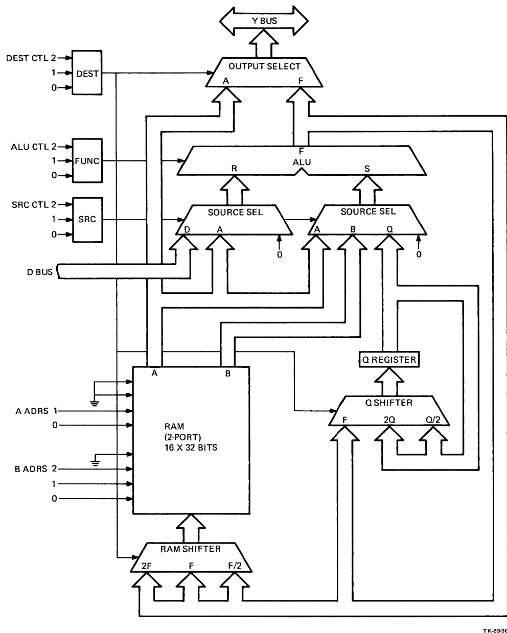
Figure 6-5 Data Processor (Eight 2901As) Simplified Block Diagram
