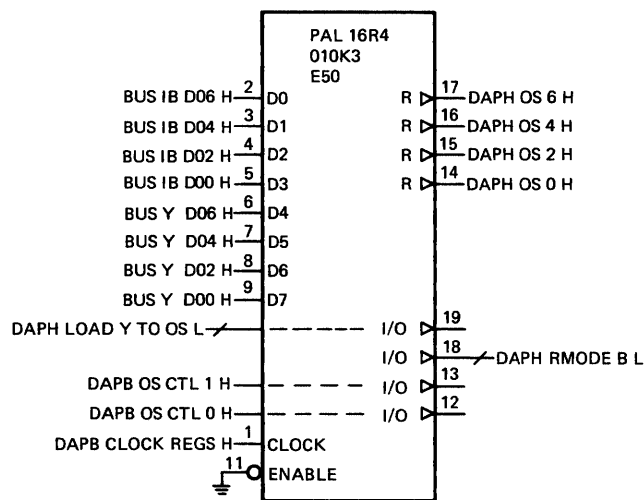
Figure A-3 Typical PAL Symbolology
