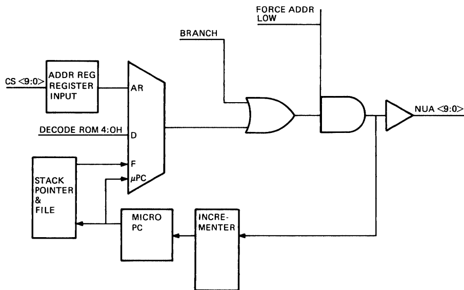
Figure 5-16 2909 Microprogram Sequencer
