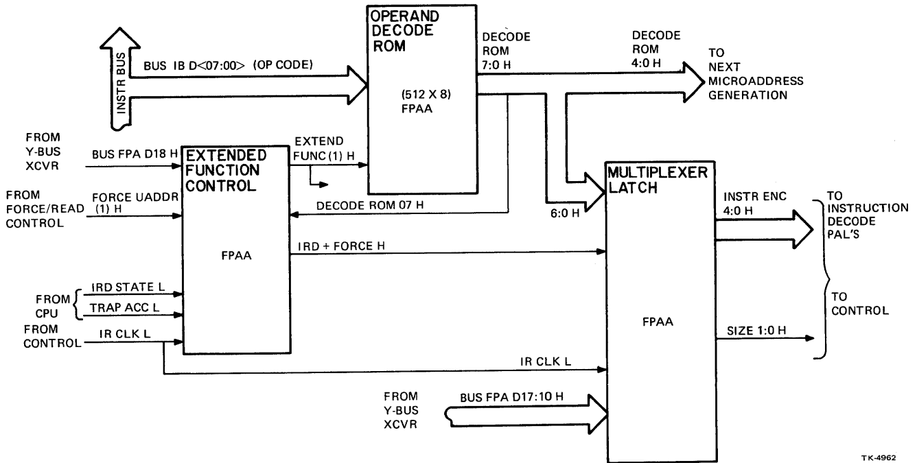
Figure 5-12 Instruction Decoding
