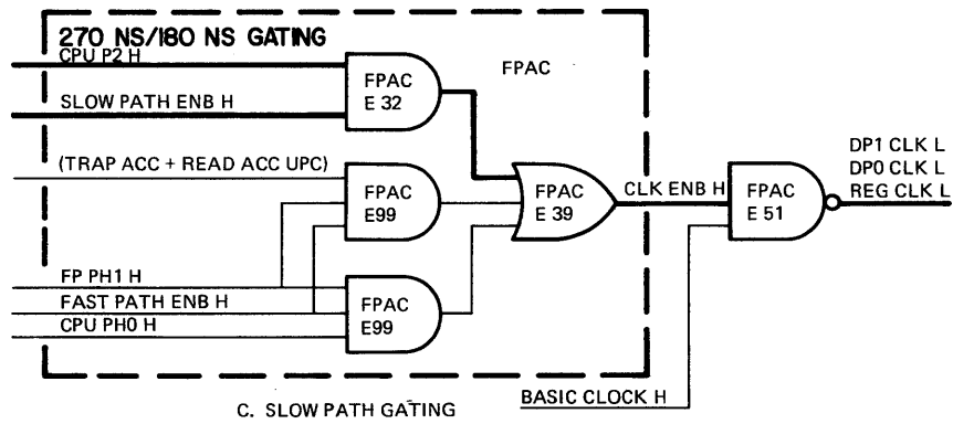
Figure 5-8 Fast/Slow Cycle Gating
