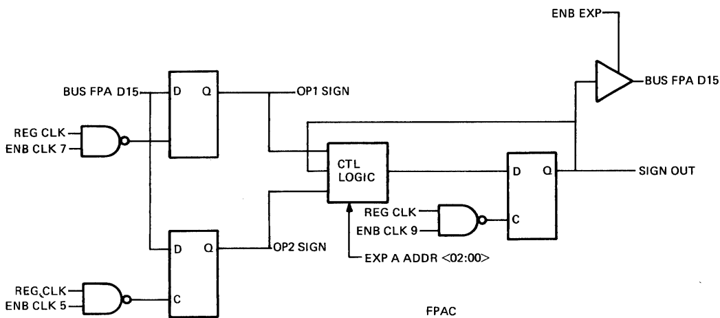
Figure 5-22 Sign Control PAL Logic
