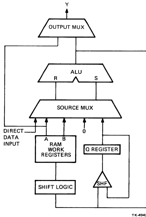
Figure 5-20 2901 Block Diagram
