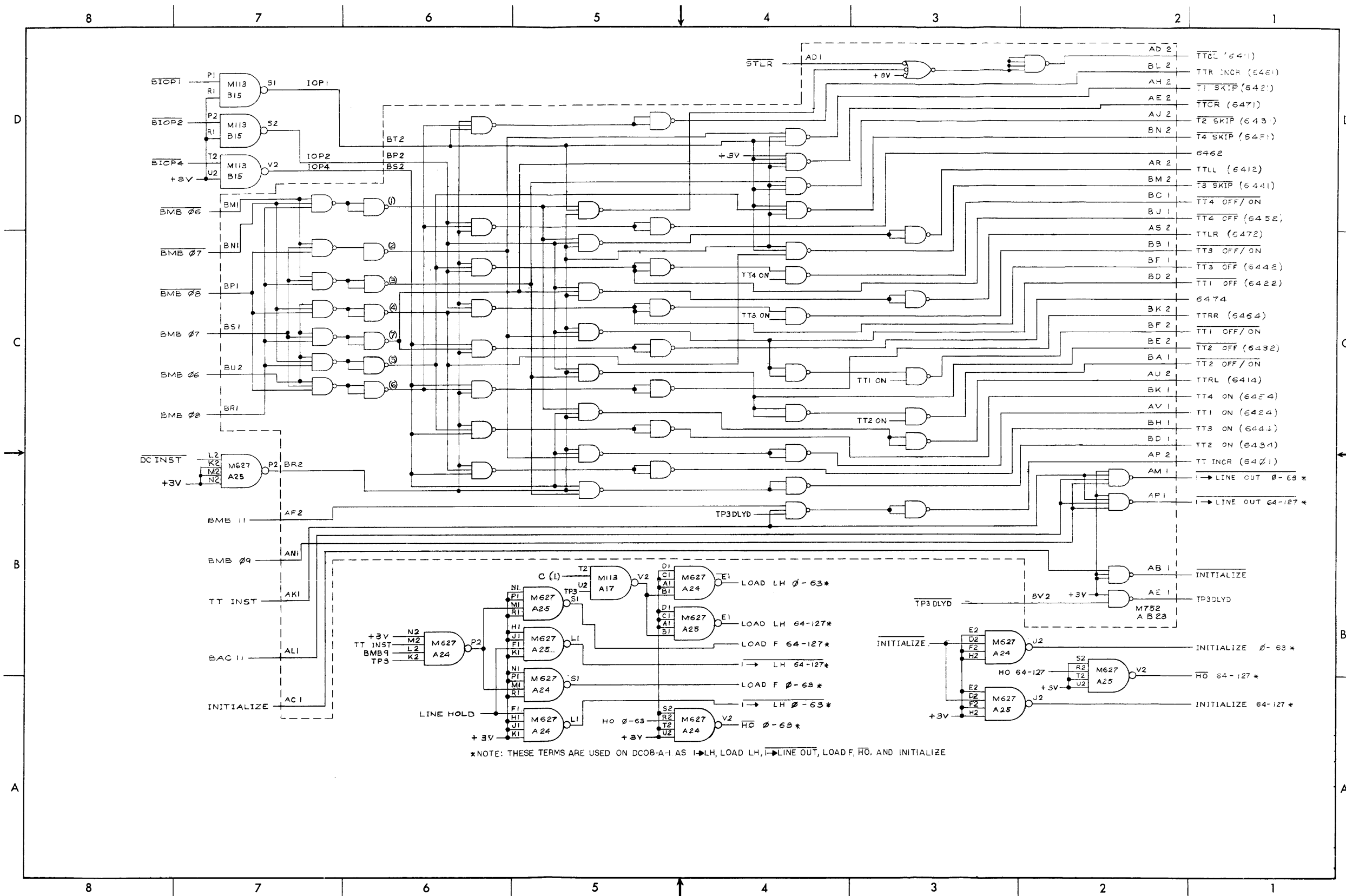
D-BS-DC08-A-4 DC08-A Instruction Decoding
