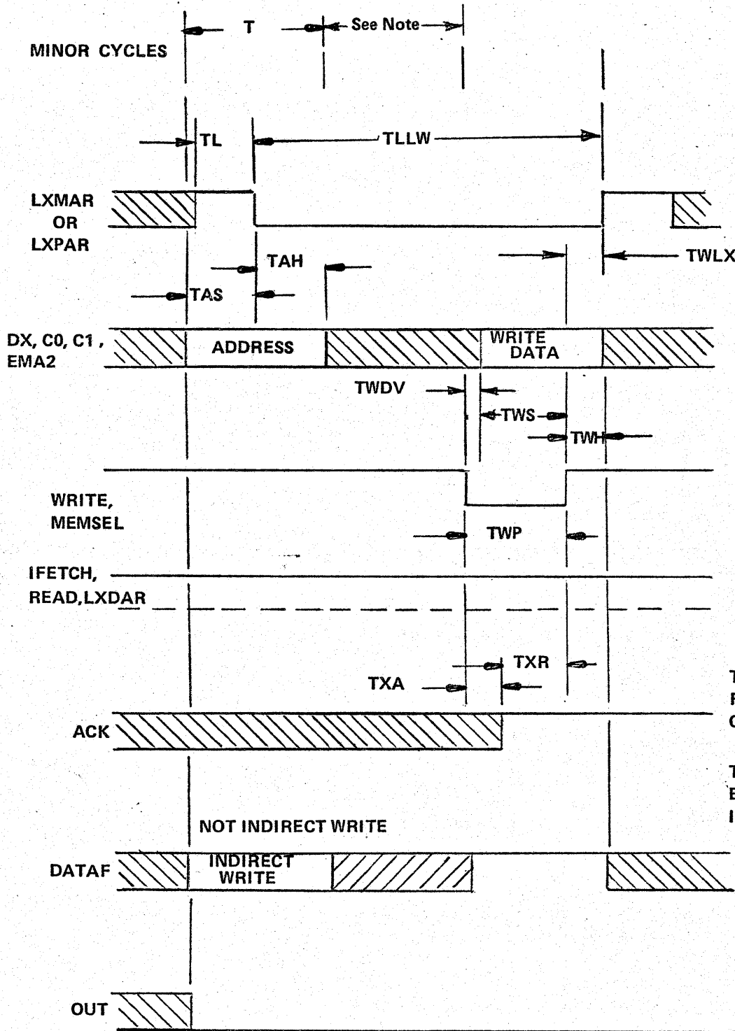
FIGURE 4 MEMORY WRITE OPERATION
