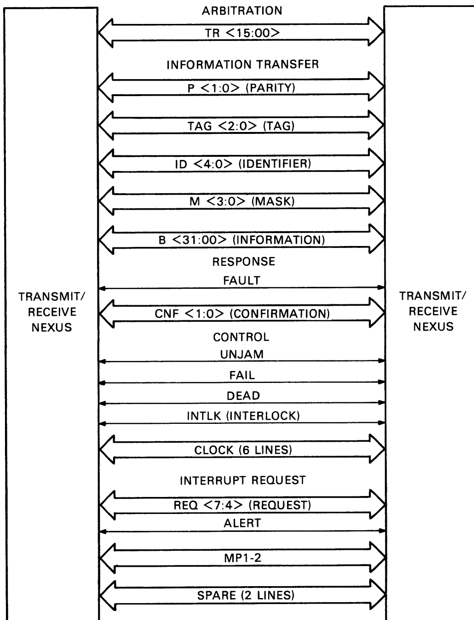
Figure 2-4 SBI Configuration
