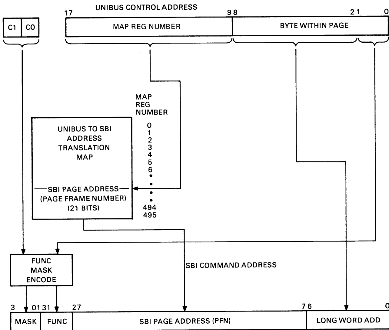
Figure 2-38 Unibus to SBI Address Translation
