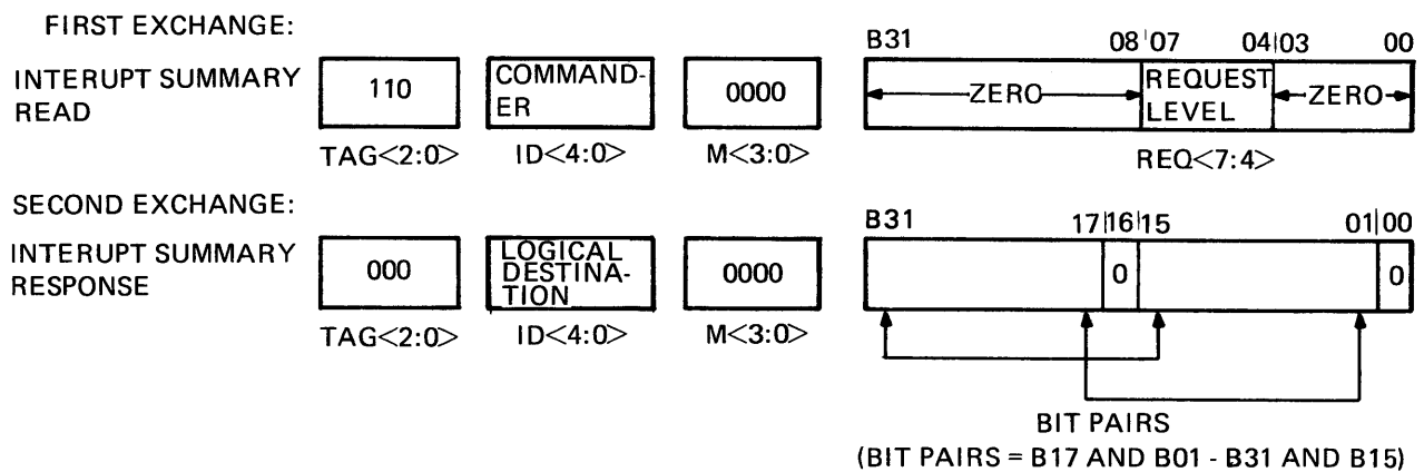
Figure 2-10 Interrupt Summary Formats
