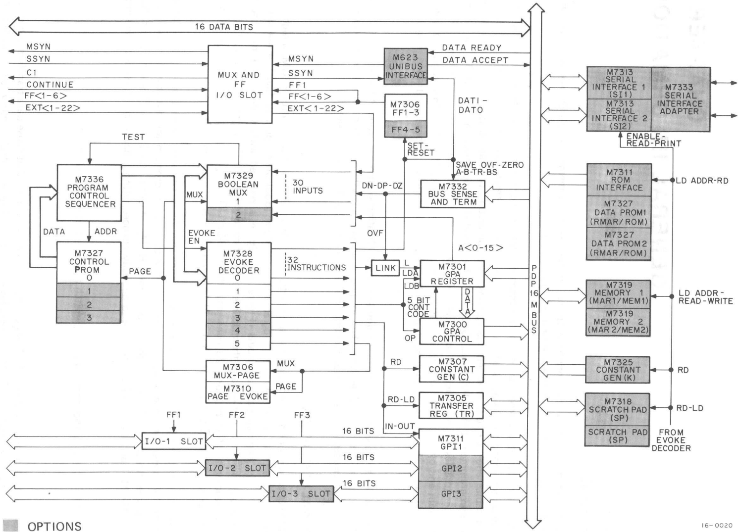
Figure 1-1 PDP16-M Minicomputer, Block Diagram
