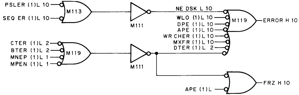
Figure 4-28 Error and Freeze
