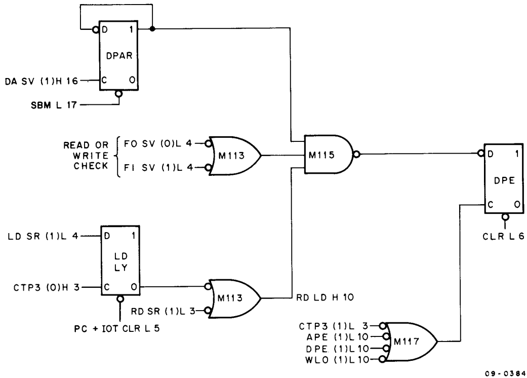
Figure 4-31 Data Parity Error
