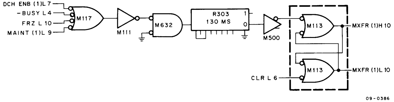
Figure 4-30 Missed Transfer Error
