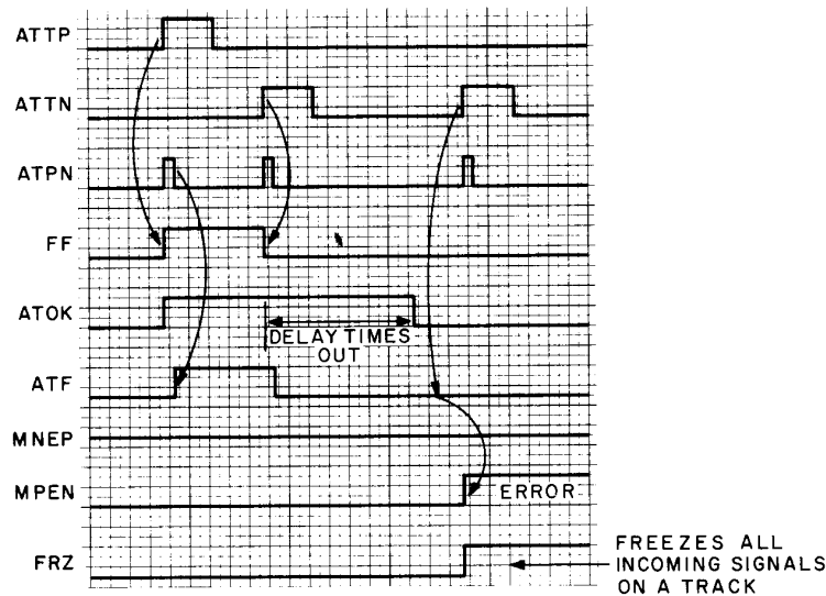
Figure 4-2 A Track Error Detection, Timing Diagram
