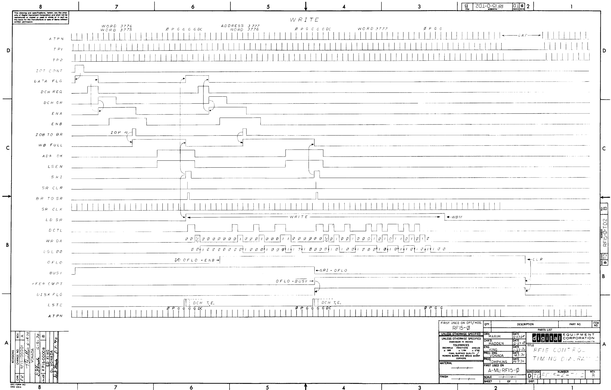
Figure 4-22 RF15 Write Control Timing Diagram
