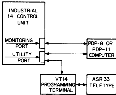
Figure 1-16 A Block Diagram of Industrial 14 System Interfacing
