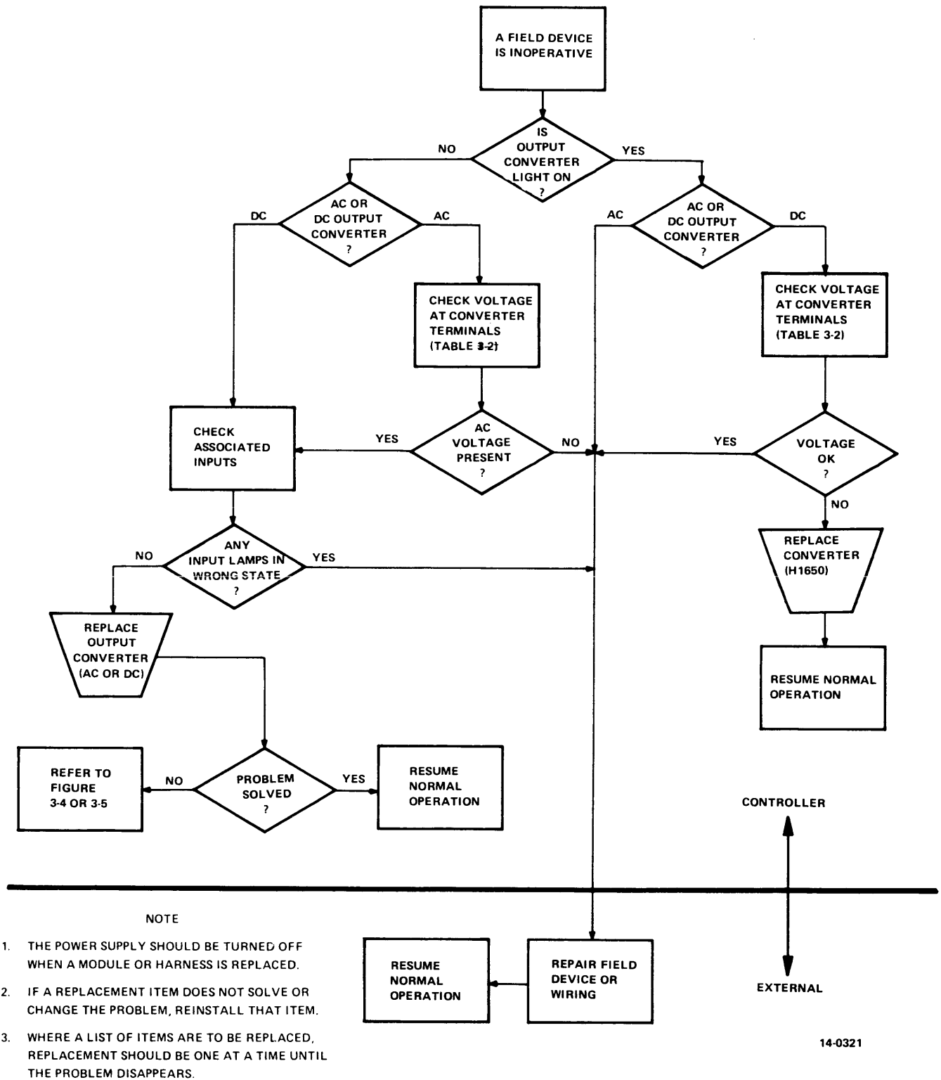
Figure 3-3 Partial Failure Isolation Procedure Using I/O Lights
