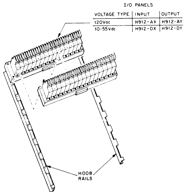
Figure 2-5 Installing an I/O Mounting Panel
