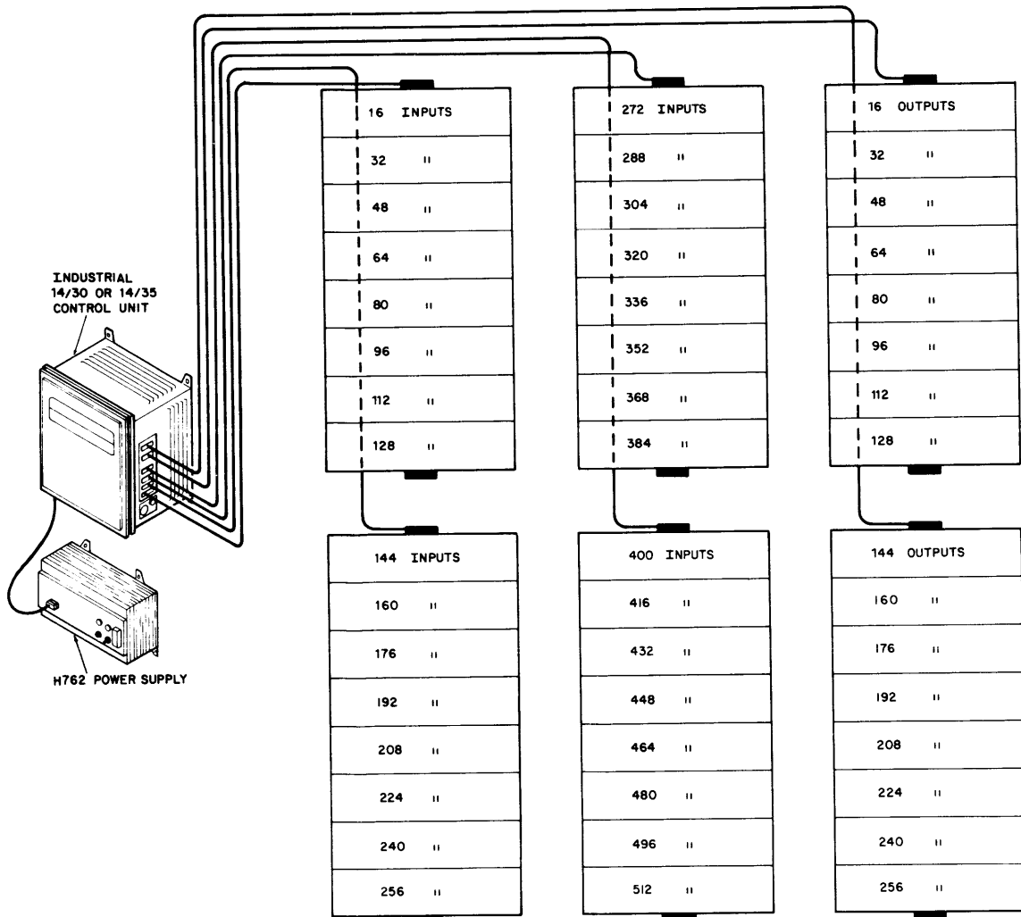
Figure 1-4 A Maximum Configuration Industrial 14 System
