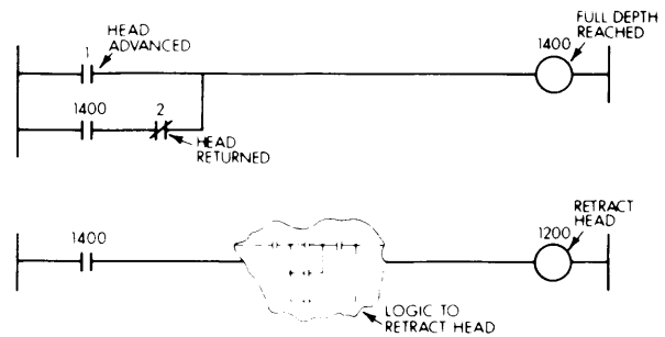
Figure 1-21 Record Full-Depth Reached Using Retentive Memory
