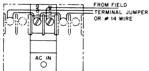
Figure 2-7 Field Wiring Connections to Converters
