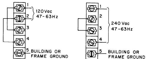
Figure 2-6 Power Supply Connections for 120 V and 240 Vac
