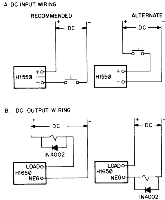
Figure 2-8 Wiring Diagram for the DC I/O Converter
