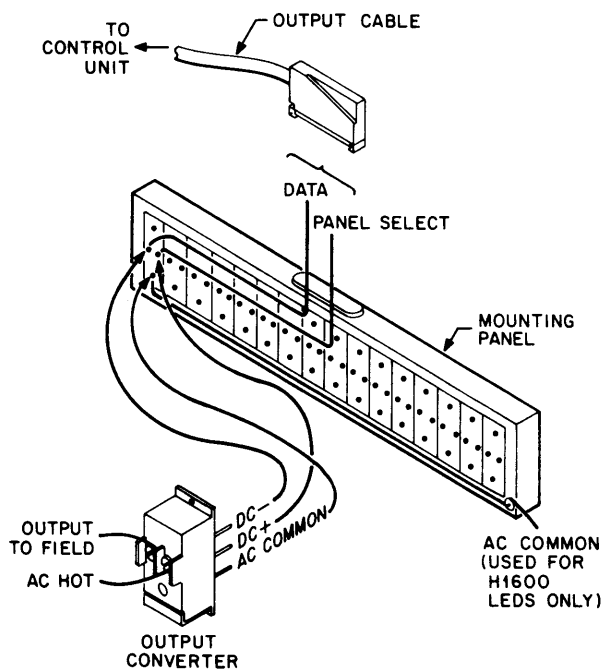
Figure 1-32 A Mounting Panel with Output Converter and Control Unit Connections Indicated
