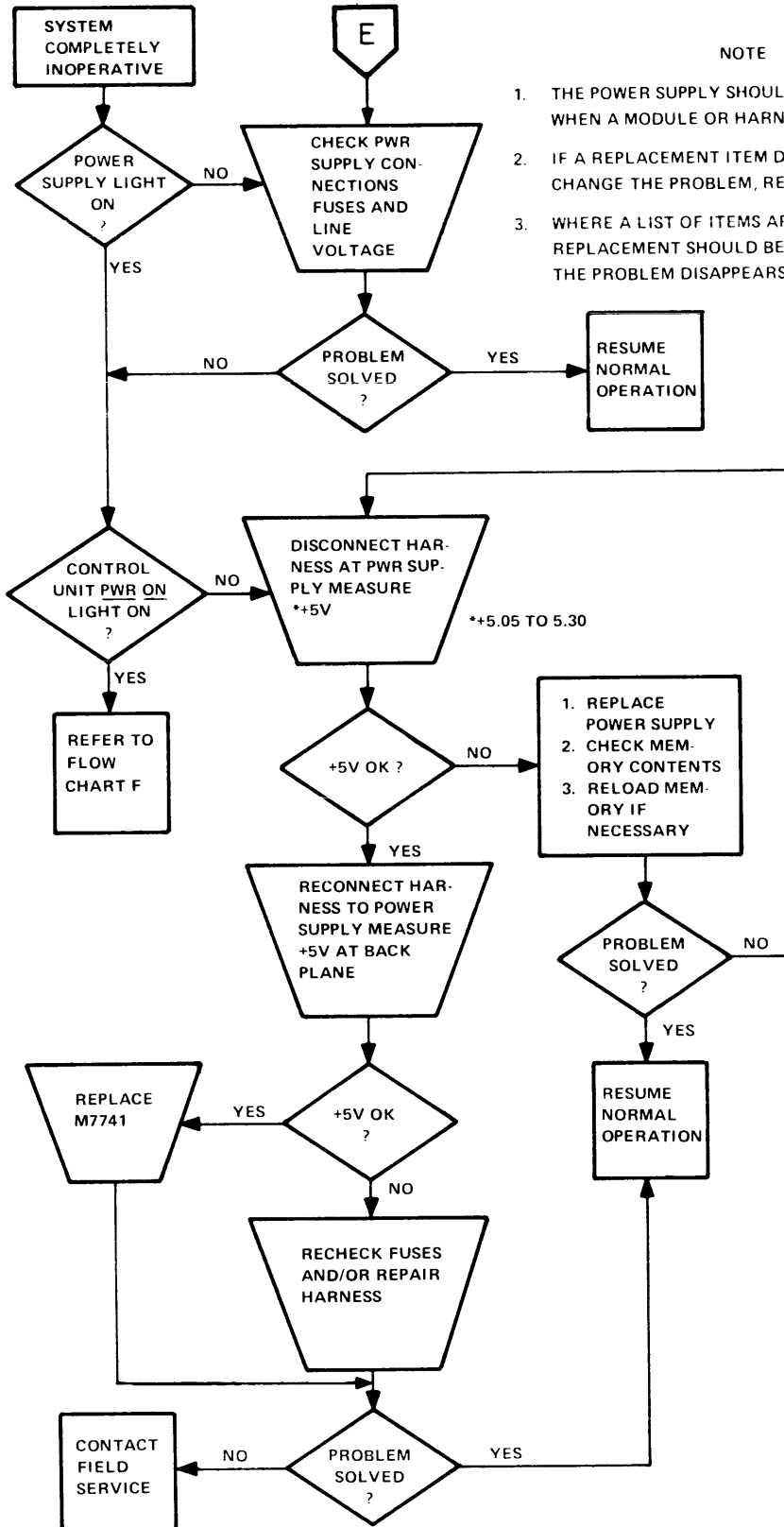
Figure 3-8e Power Up Unsuccessful (Power On Lights)
