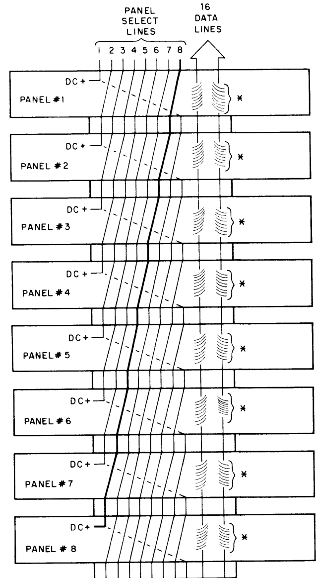
Figure 1-33 H912 Panel Selection Technique
