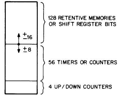
Figure 1-20 Internal Function Partitioning
