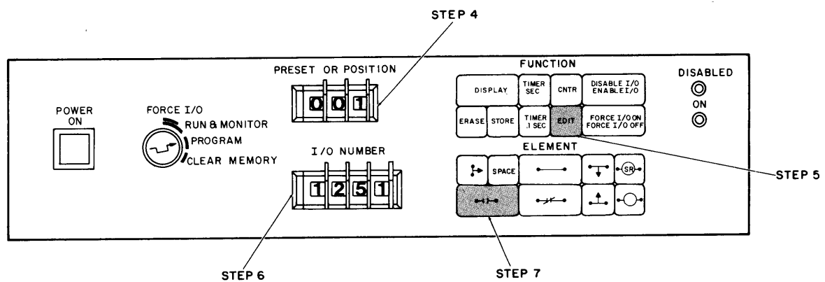
Figure 3-5 Procedure for Changing the Position of an Element
