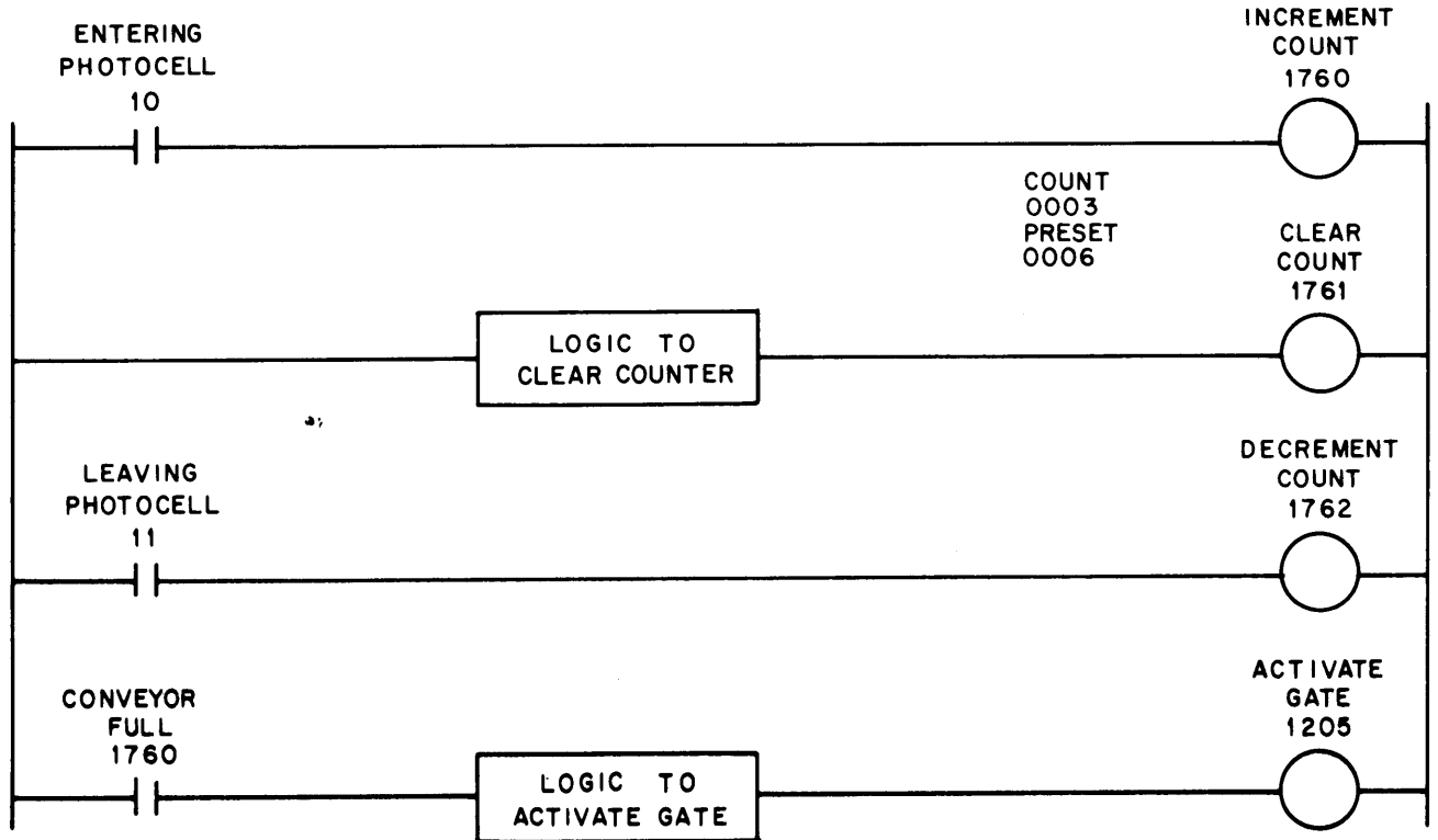
Figure 2-16 Up/Down Counter Circuit to Limit Parts on a Conveyer to a Maximum of Six
