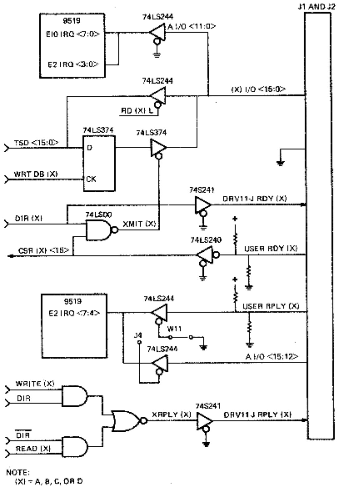
Figure 4-3 I/O Bus Interface, Simplified Schematic
