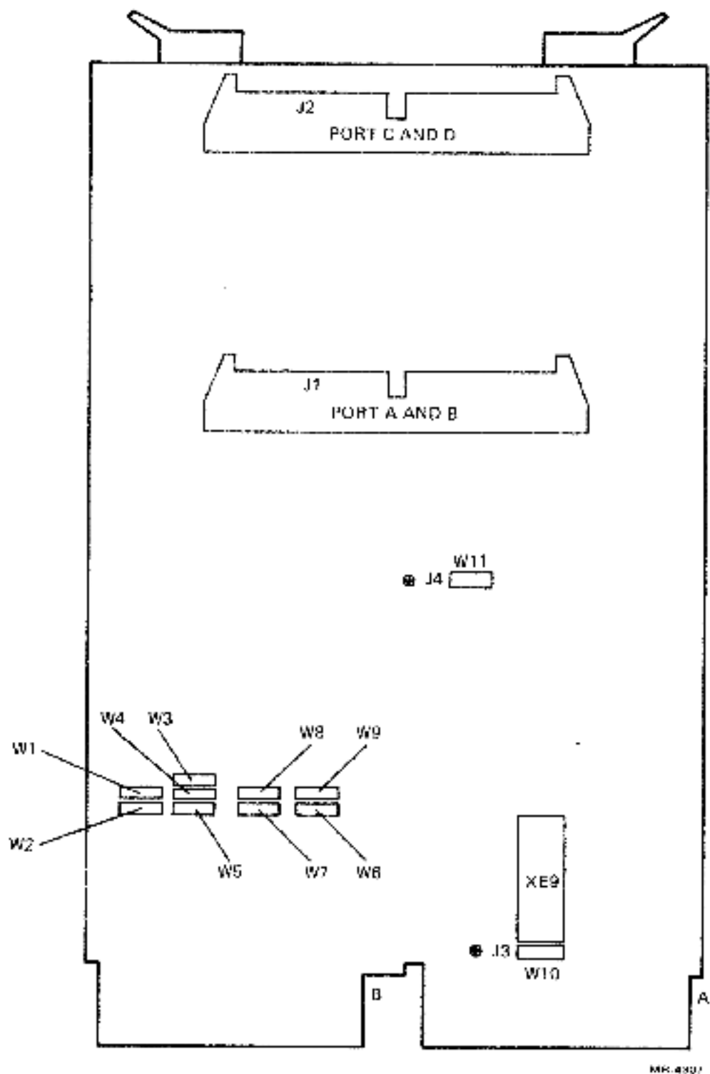
Figure 3-1 DRV10-J Jumper Locations
