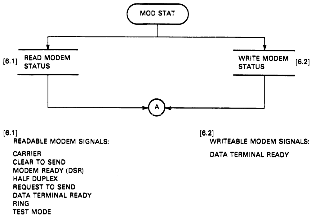
Figure D-6 Modem Control (Modem Status)
