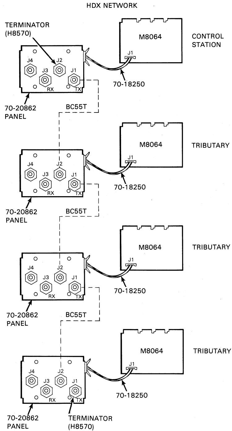
Figure 2-12 Half-Duplex Multipoint Network (Control Station End Node)
