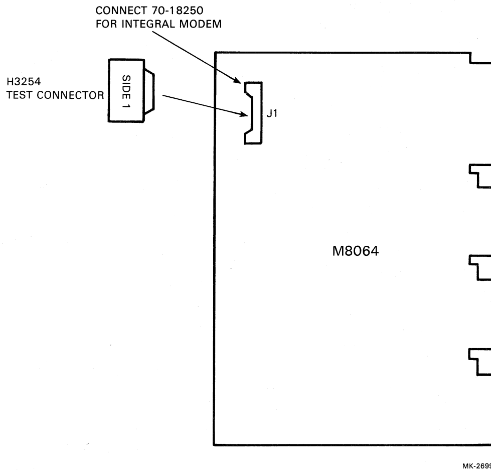
Figure 2-7 Test Connector Insertion for the M8064
