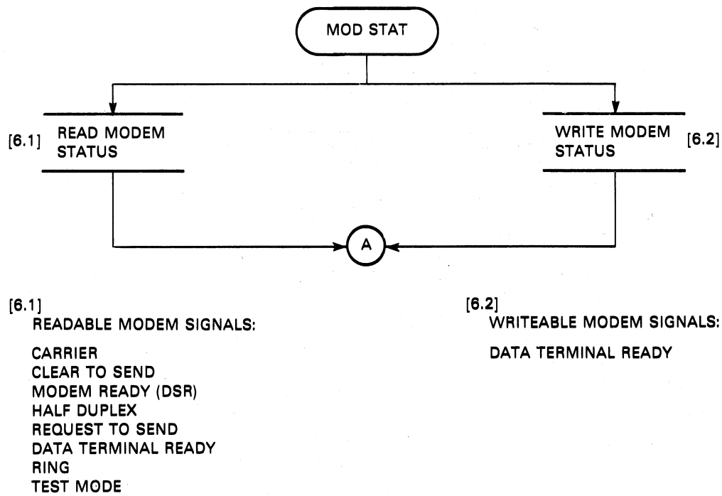
Figure D-6 Modem Control (Modem Status)
