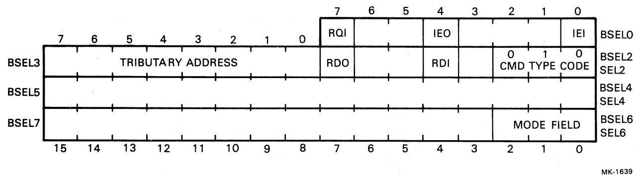
Figure 3-5 Mode Definition Command Format
