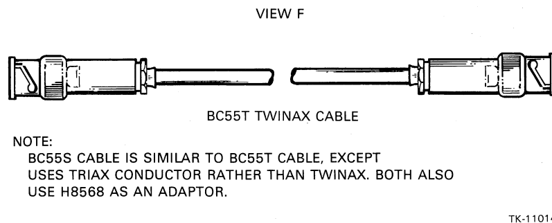
Figure 2-9 DMV11 Cable Drawings (Sheet 2 of 3)
