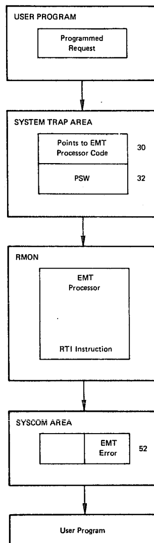
Figure 1-1: System Flow During Programmed Request Execution
