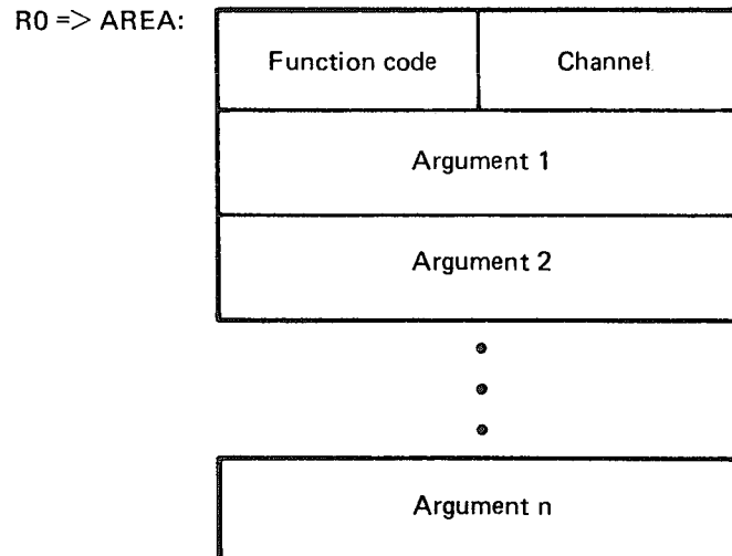
Figure 1-4: EMT 375 Argument Block
