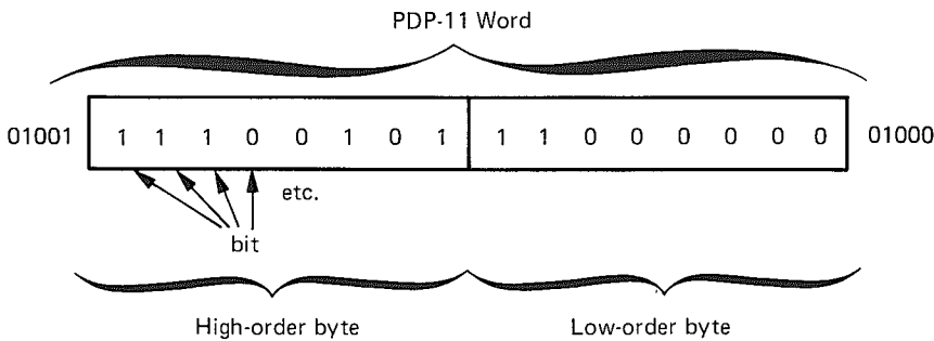
Figure 11-5 PDP-11 Word
