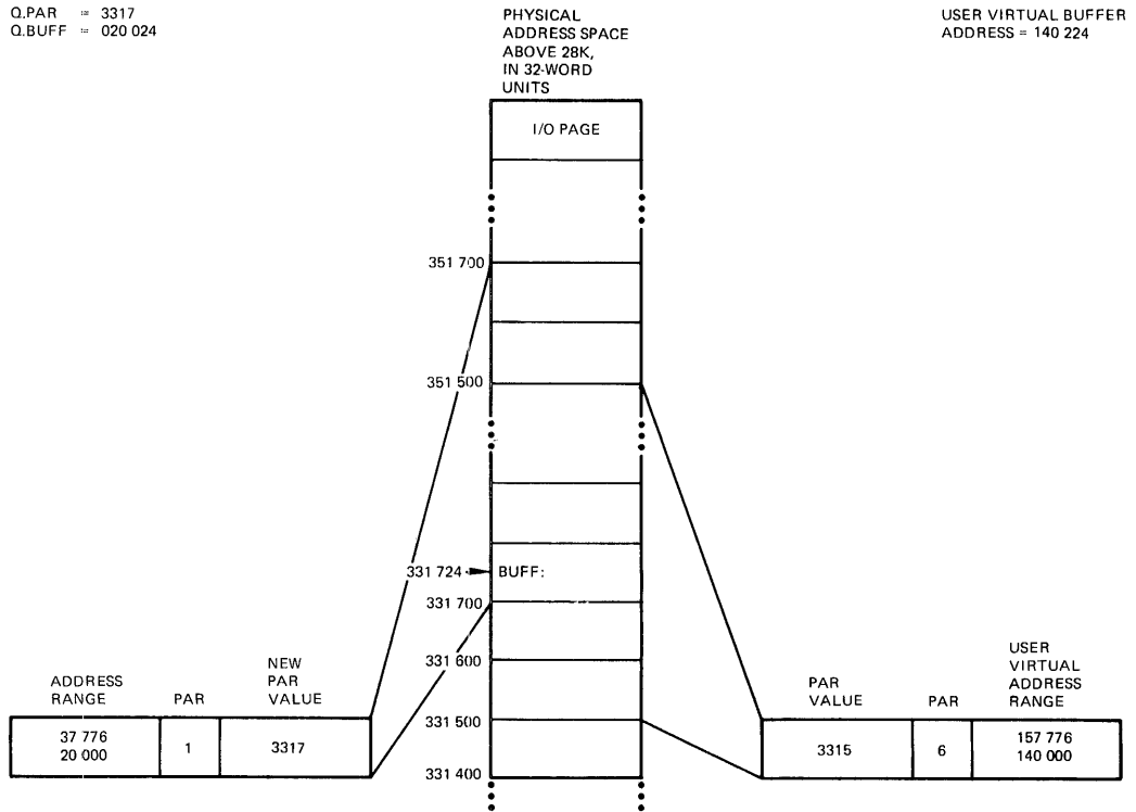
Figure 7-6: PAR1 Mapping
