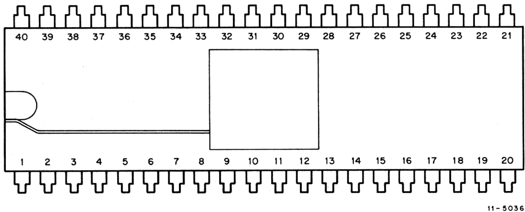
Figure A-12 UART Pin Locations
