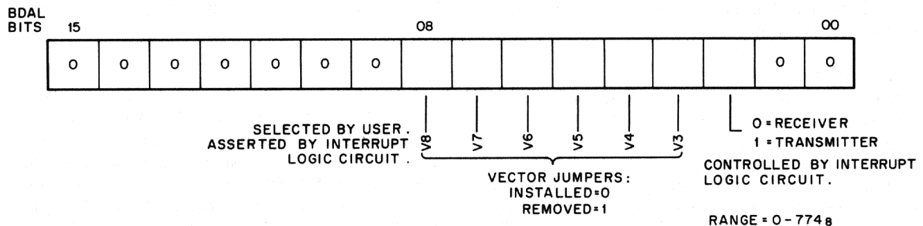
Figure 5-2 DLV11-E and DLV11-F Interrupt Vectors
