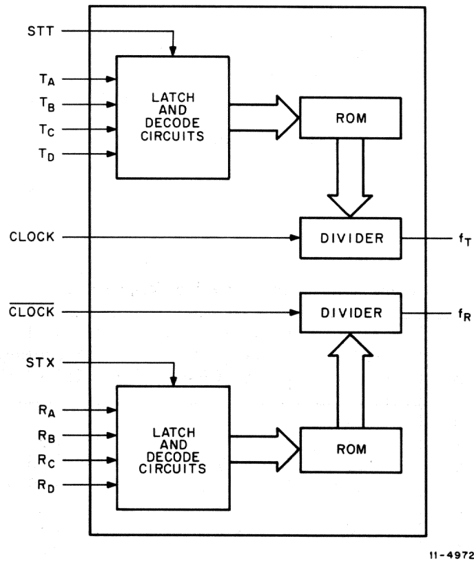
Figure A-13 5016 Block Diagram
