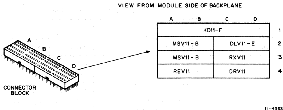
Figure 3-5 Typical Backplane Configuration
