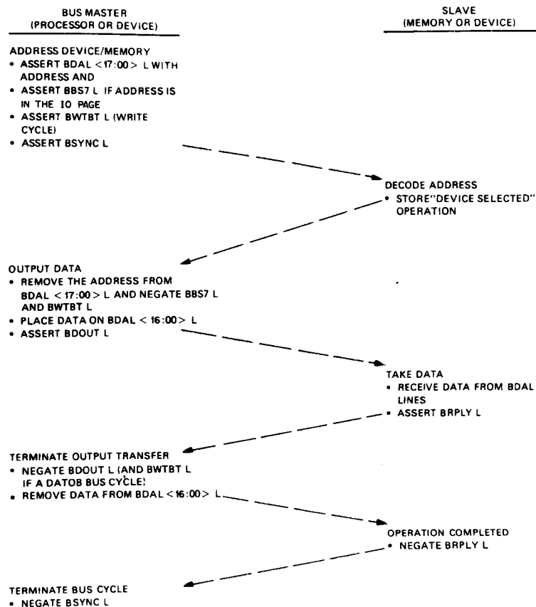
Figure 4-3 DATG or DATOB Bus Cycle
