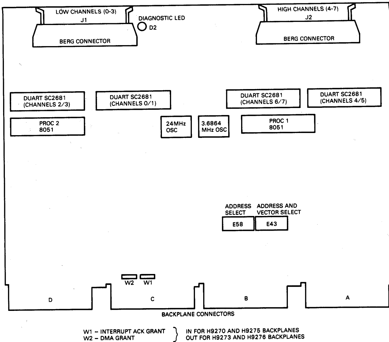
Figure 1-1 M3104 Module
