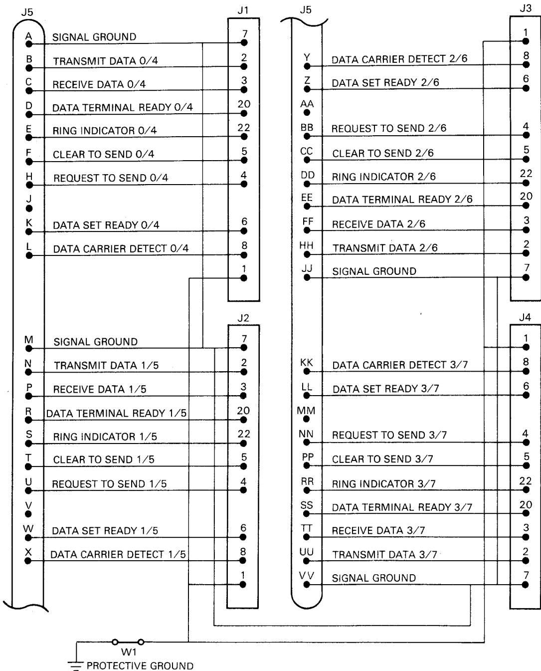
Figure 2-7 H3173-A Circuit Diagram
