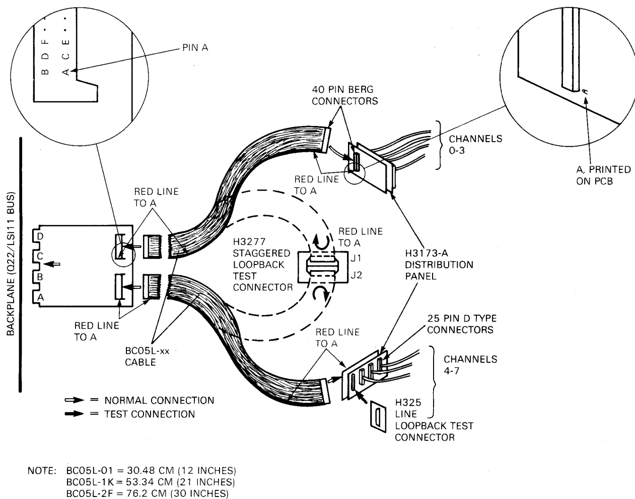
Figure 2-5 DHV11 Installation
