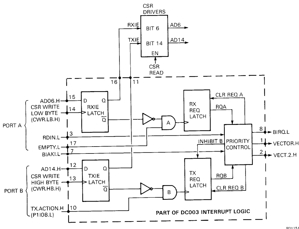
Figure 4-17 Interrupt Logic
