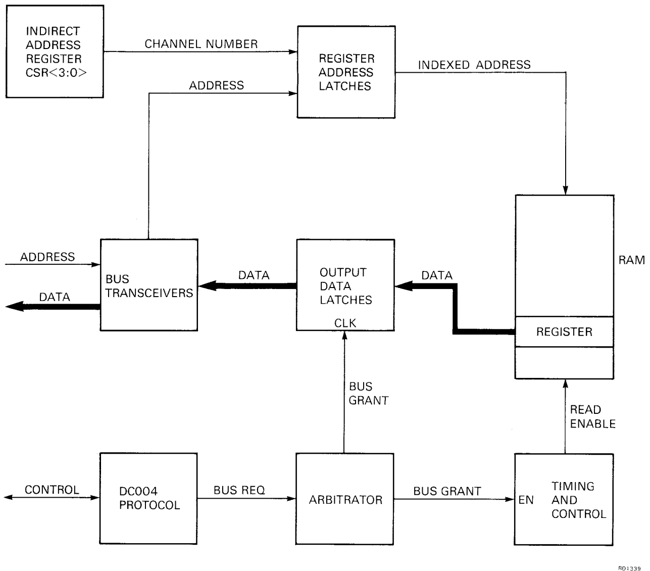
Figure 4-8 Reading from a Register
