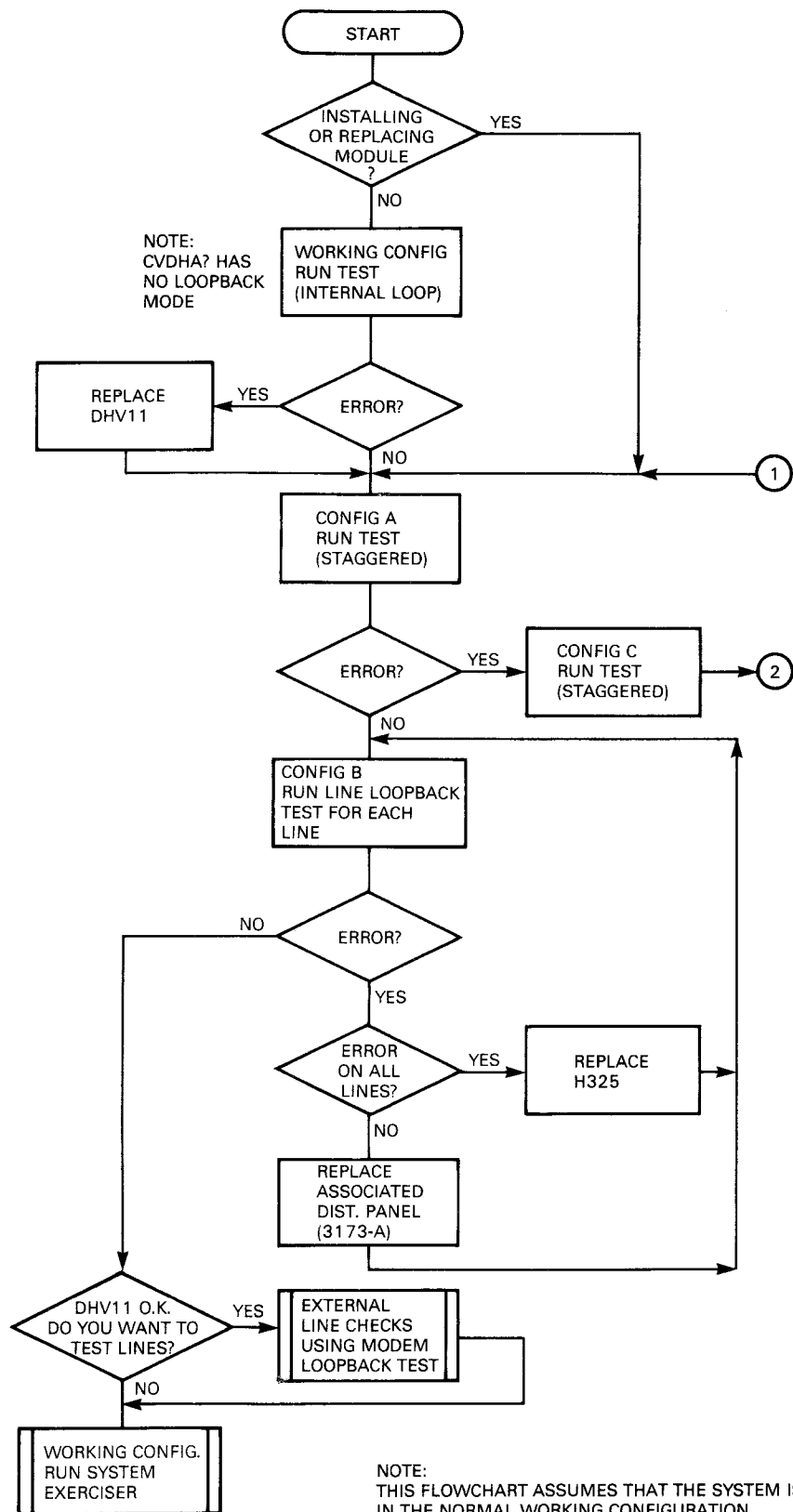
Figure 5-2 Troubleshooting Flowchart
