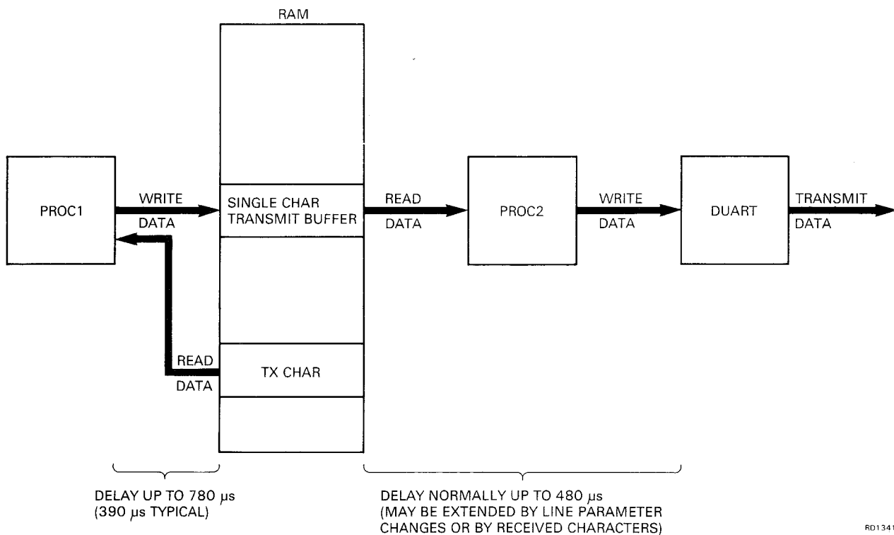
Figure 4-10 Single-Character Transmit
