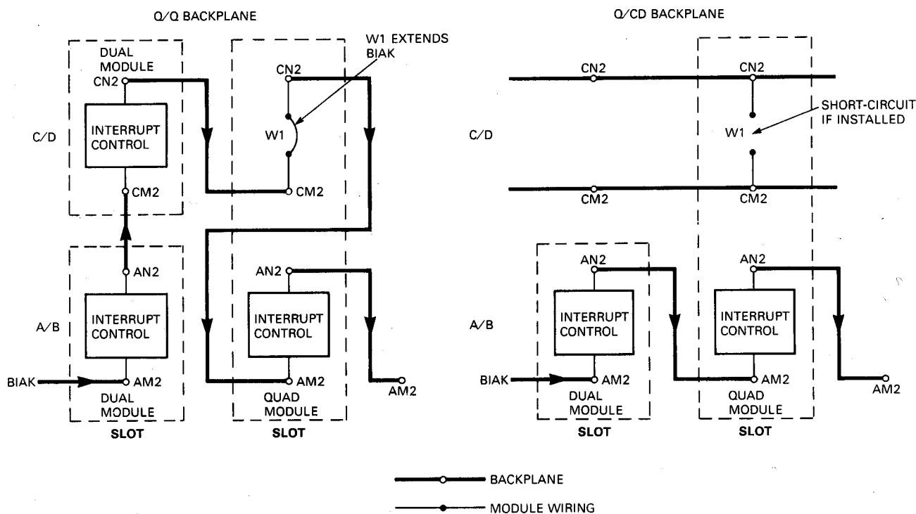
Figure 2-4 Bus Grant Continuity
