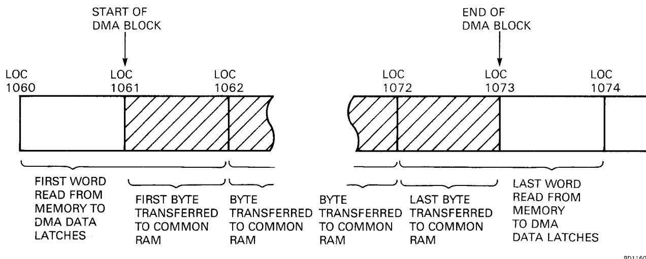
Figure 4-12 DMA Character Handling
